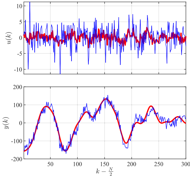
FIGURE 11. I/O data (Example 3, \text{SNR}_u = -6.7 dB, \text{SNR}_y = 11.5 dB, only the middle 300 samples are shown).
