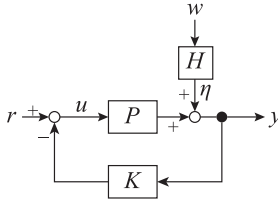
FIGURE 1. Closed-loop system.
