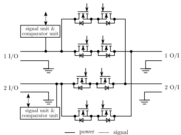
Fig. 3: Switching circuit of proposed router. MOS-FETs are SiC MOSFETs (SCT3022AL).
