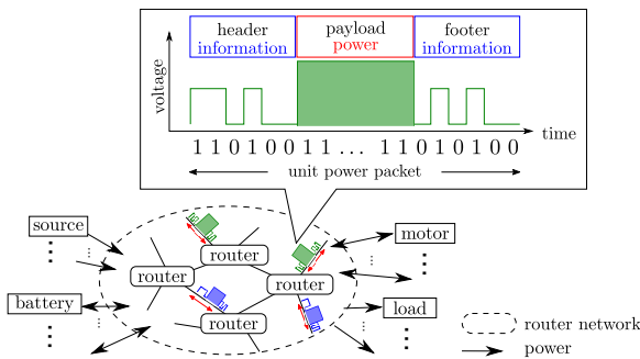
Fig. 1: Concept of power packet and its dispatching system.
