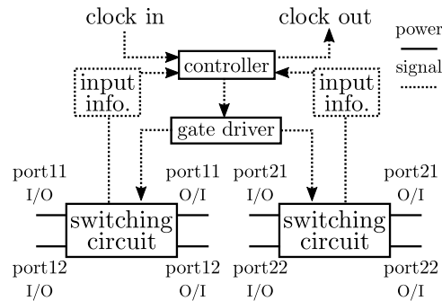
Fig. 2: Schematic diagram of bidirectional power packet router proposed in this brief.
