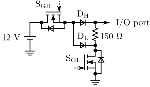
Fig. 4: Schematic diagram of signal unit. FETs are GaN HEMT (EPC2010) and diodes are (MBRS3201T3G). 12.0 V source is the same as the source of the router.
