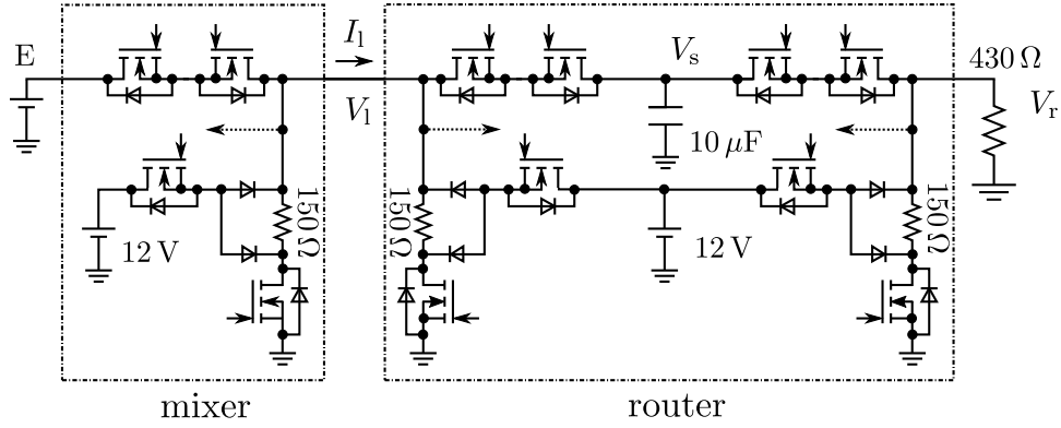
Fig. 6: Experimental circuit configuration with one power source and one load. The source voltage E is set at 100 V. Dotted arrows show the connections to the comparator units.
