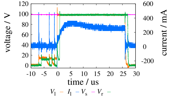
Fig. 7: Example of experimental waveforms. V_1 and I_1 show the voltage and the current waveforms of the power line between the mixer and the router. V_s and V_r show the voltage waveforms of the storage and the load, respectively. V_s was measured with DC offset of 80 V to reduce the effects of noise.
