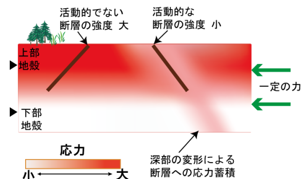
Fig.1 Generating process of intraplate earthquakes
