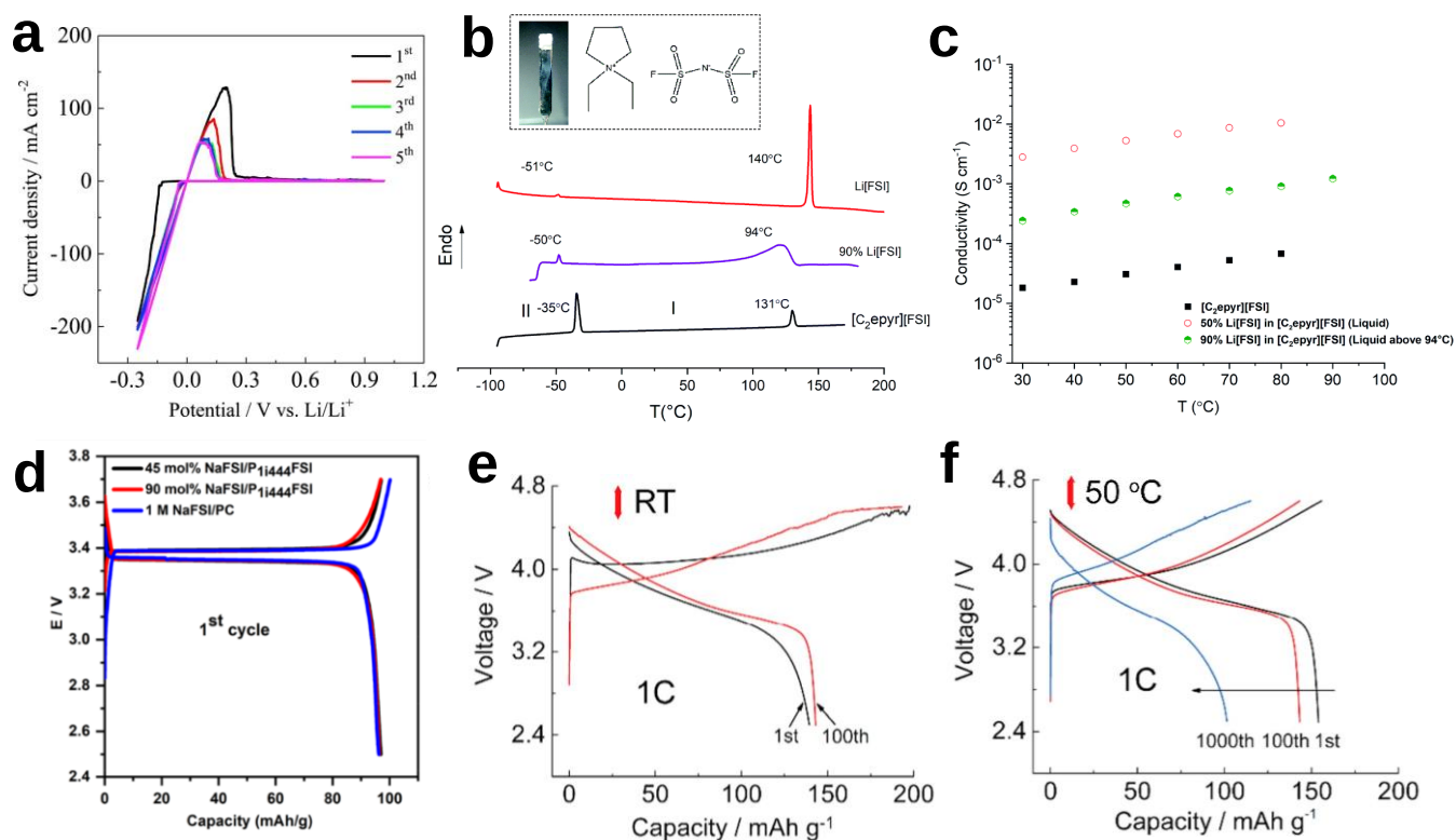
Fig. 12 a. Cyclic voltammograms of a Ni electrode in the 5 mol% Li[FSA]-[C 2 C 2 pyrr][FSA] IPC at 60 °C, corresponding to Li metal deposition/dissolution. Reproduced with permission. 300 Copyright 2019, Elsevier. b. DSC curves and c. the temperature dependence of ionic conductivity for the 90 mol% Li[FSA]-[C 2 C 2 pyrr][FSA] quasi-solid state material and those of related materials. The inset of b. indicates the structure of [C 2 C 2 pyrr][FSA] and a photograph of the quasi-solid state material on a spatula held vertically to demonstrate its solid nature. Reproduced with permission. 321 Copyright 2019, The Royal Society of Chemistry. d. The first cycle charge-discharge curves of the Na/Na 3 V 2 (PO 4 ) 3 cell with the 90 mol% Na[FSA]-[P 11444 ][FSA] quasi-solid state material and related electrolytes at 0.2C. Reproduced with permission. 350 Copyright 2020, American Chemical Society. e, f. The charge-discharge curves of the Li/LiNi 1/3 Mn 1/3 Co 1/3 O 2 cell with the composite electrolyte of PVDF particles and IPC (60 wt% PVDF-40 wt % IPC (50 mol% Li[FSA]-[C 2 C 2 pyrr][FSA])) at 1.0C at room temperature (RT) and 50 °C. Reproduced with permission. 338 Copyright 2018, Elsevier.
