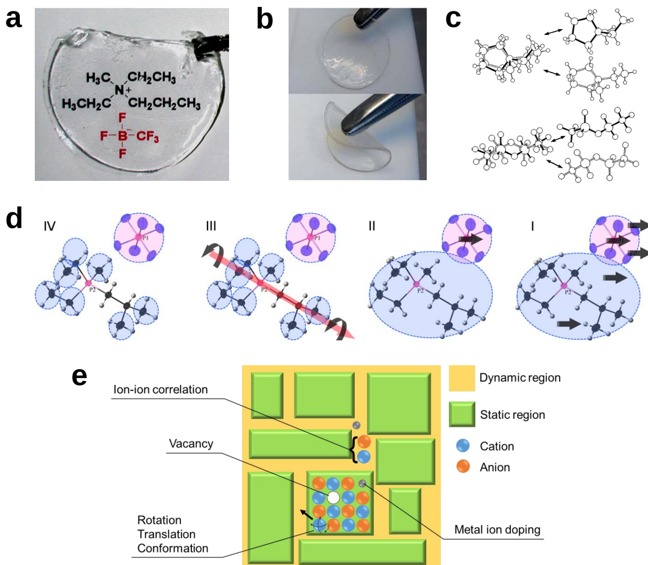
Fig. 11 a. An Image of free-standing IPE film (ca. 50 mm in diameter) of the [N_{1223}][CF_3BF_3] IPE. Reproduced with permission. 255 Copyright 2007, Elsevier. b. Image of the PIL/ [C_2C_1pyrr][FSA]/Li[TFSA] (PIL: [P(DADMA)][TFSA] ) SPE film, reaching a flexion angle of about 180^\circ without breaking. Reproduced with permission. 127 Copyright 2017, The Royal Society of Chemistry. c. Disorder modes of the cation and anion in the [C_2C_1pyrr][TFSA] structure at -60^\circ C . Reproduced with permission. 258 Copyright 2006, American Chemical Society. d. Schematic of molecular motions in the different phases (IV to I) of [P_{12214}][PF_6] in response to increasing temperature. Reproduced with permission. 283 Copyright 2012, American Chemical Society. e. Schematic of possible factors affecting ion conduction in IPEs.
