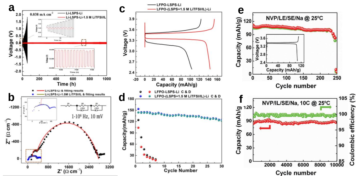
Fig. 6 a. Li deposition-dissolution test employing a Li/Li 10 SnP 2 S 12 /Li symmetric cell with and without the Li[TFSA]-[C 3 C 1 pyrr][TFSA] IL. b. EIS Nyquist plots of the Li/LSPS/Li symmetric cell with and without the IL. Electrochemical performance of Li/LSPS/LiFePO 4 cell with and without IL c. Charge-discharge curves and d. cycle tests Li/LSPS/LiFePO 4 cells with and without IL. Reproduced with permission. 55 Copyright 2018, American Chemical Society. Cycle performance of NVP/Na cell e. without IL and f. with IL. Reproduced with permission. 30 Copyright 2017, Wiley-VCH.
