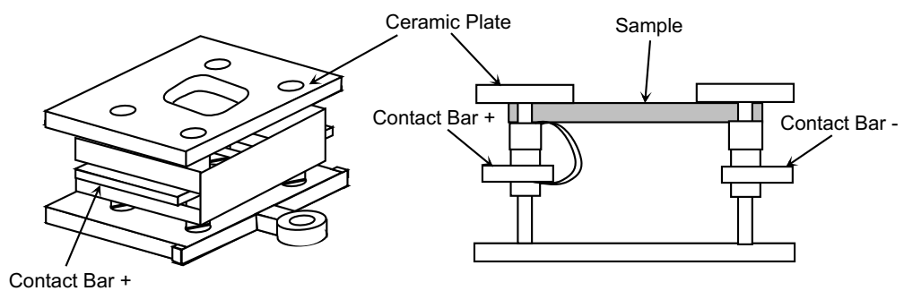
Figure 2.4: Schematic diagram of a sample holder of the VT-STMicroscopy system.
