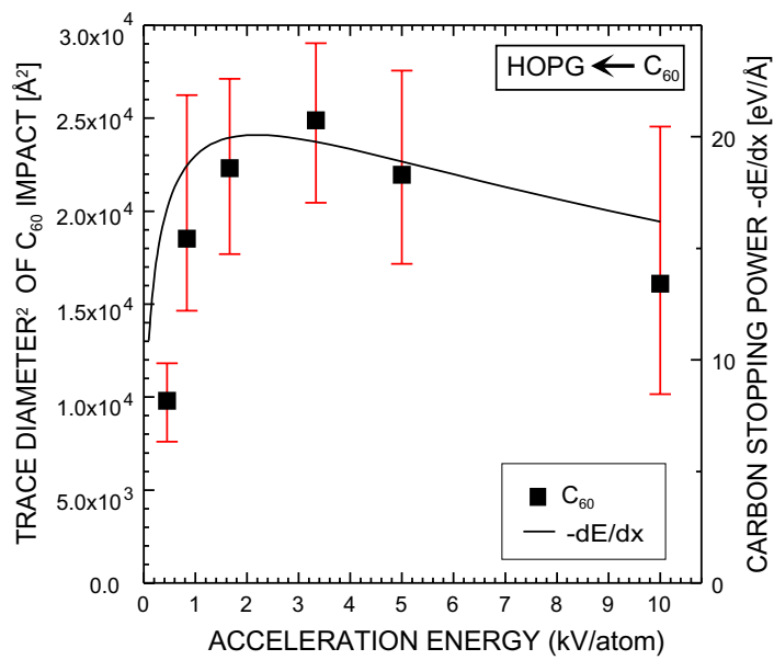
Figure 4.11: Dependence of trace area of C_{60} impact on an HOPG surface on acceleration voltage. The solid line is nuclear stopping power of a carbon atom in graphite calculated by using ZBL potential.
