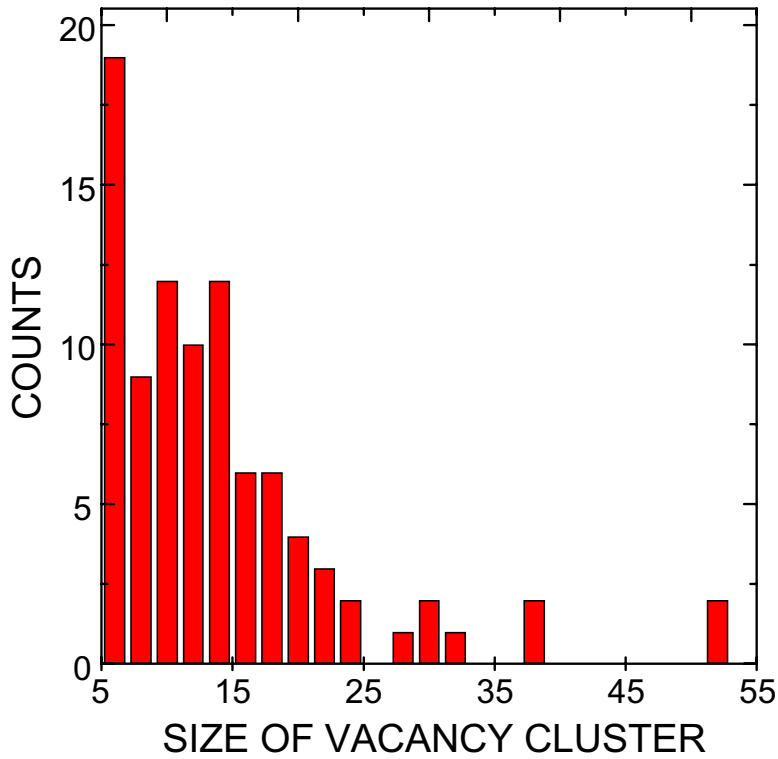
Figure 3.9: The size histogram of vacancy clusters at 600°C. Vacancy clusters of size smaller than 5 were ignored from the analysis.
