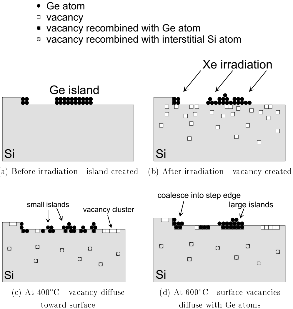
Figure 5.10: Model of the complex surface structure formation.
