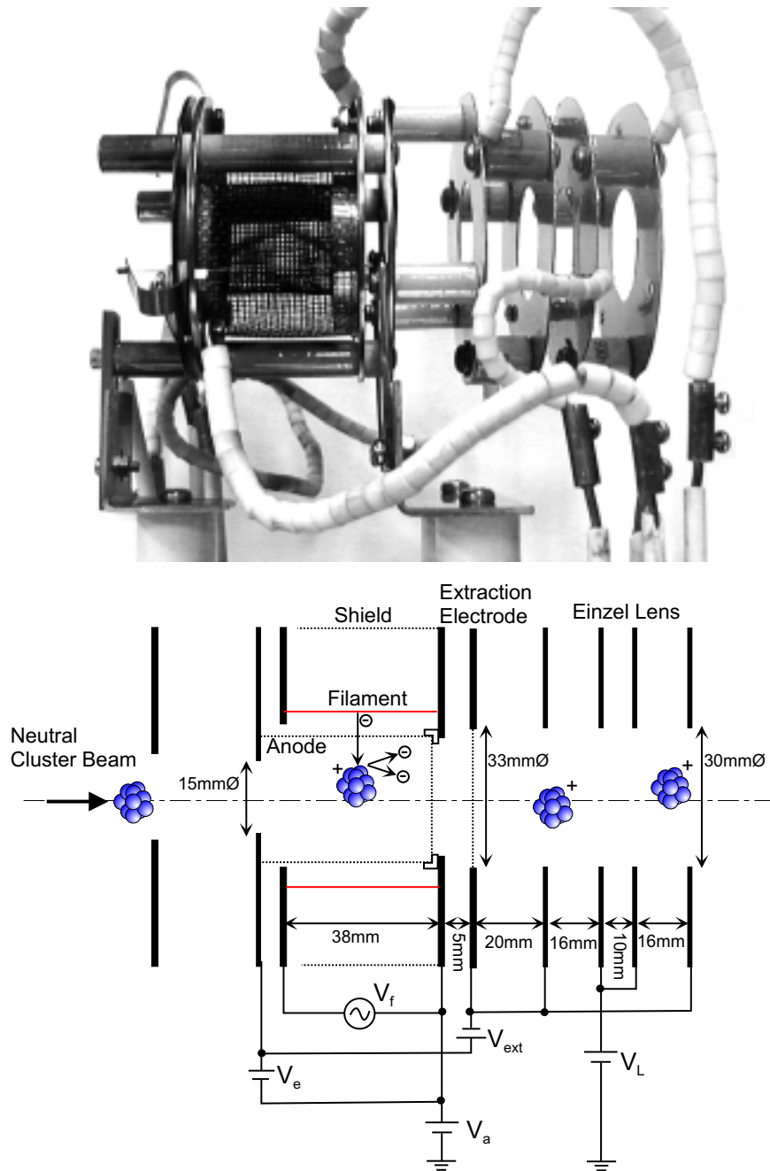
Figure 2.7: Picture and schematic diagram of an ionizer.
