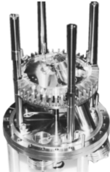
Figure 2.3: VT-STMicroscopy system.
