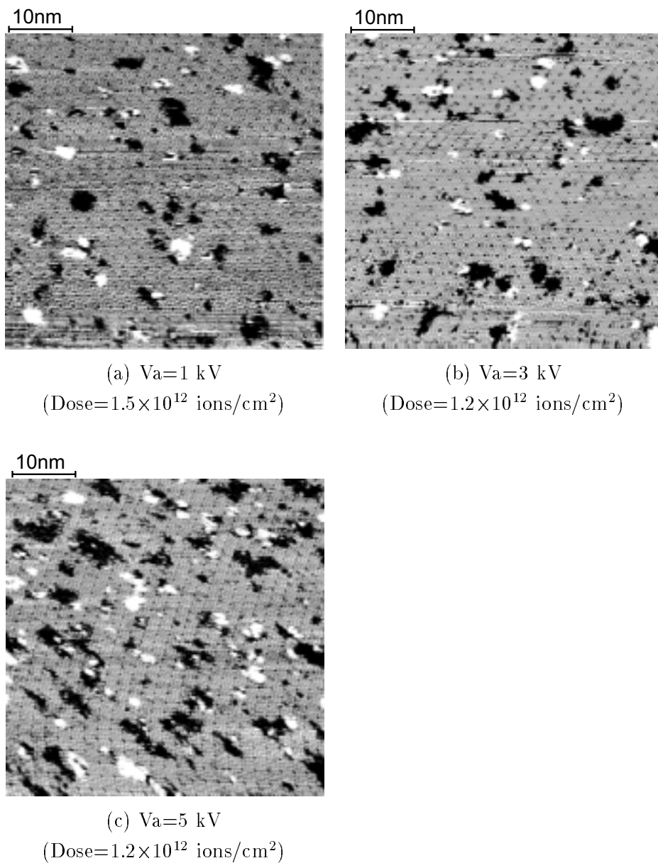
Figure 3.7: Xe-irradiated Si(111) 7x7 surface after annealing at 600°C. (Annealed for 30 minutes)
