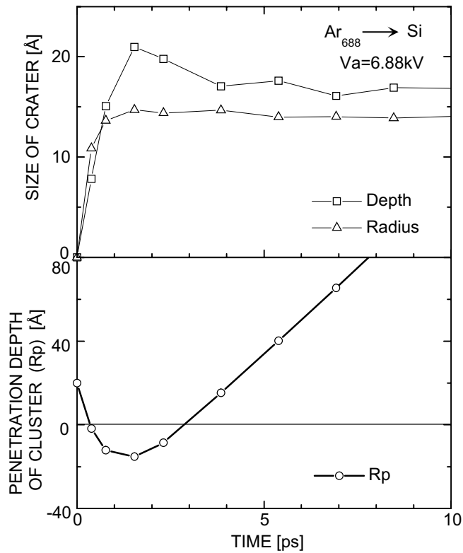
Figure 4.5: Time dependence of the penetration depth of the cluster and of the crater size.
