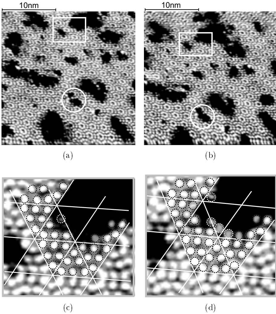
Figure 3.10: A series of images of same area obtained at 600^{\circ}\text{C} . (b) was observed at following late 60 sec after (a). (c) and (d) were high-resolution images of (a) and (b), respectively.
