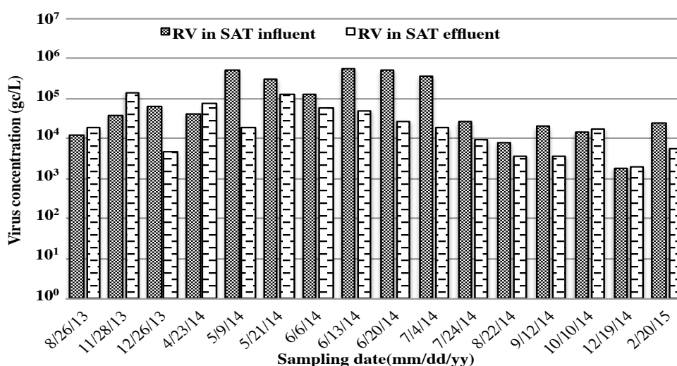
Figure 4.14: RV influent and effluent with 1-month pairing data of influent and effluent sample for estimating its removal
