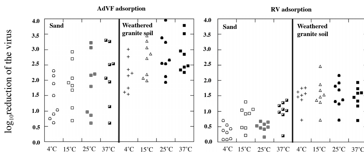
Figure 3.2: AdVF adsorption and RV virus adsorption: the left side is the AdVF adsorption onto sand and weathered granite soil at 4°C, 15°C, 25°C and 37°C, respectively. The right side is the RV adsorption onto sand and weathered granite soil at 4°C, 15°C, 25°C and 37°C, respectively.
