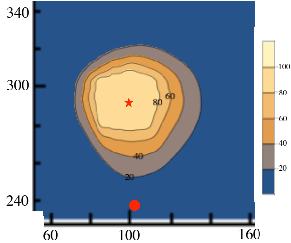
Figure 5.12: Case 1 of RV simulation profile after 2D transport model in Katsura River Basin with 0.168 \text{ day}^{-1} reduction rate coefficient; ★ denotes the injection point, • denotes the withdrawal point; x-and y-axes show the distance values in meters
