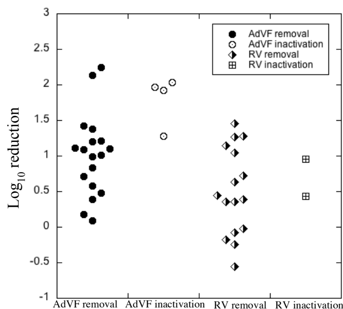
Figure 4.17 Infectious viruses with 1-month paring data of influent and effluent samples for estimating the inactivation capacity
