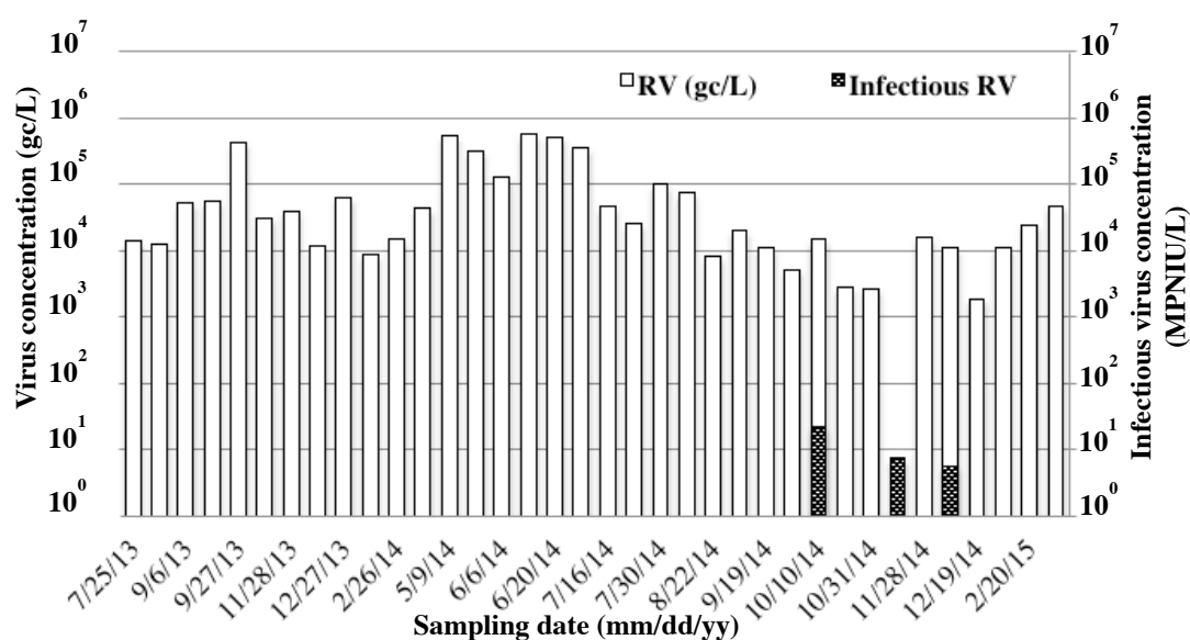
Figure 4.11 RV and infectious RV in SAT influent samples
