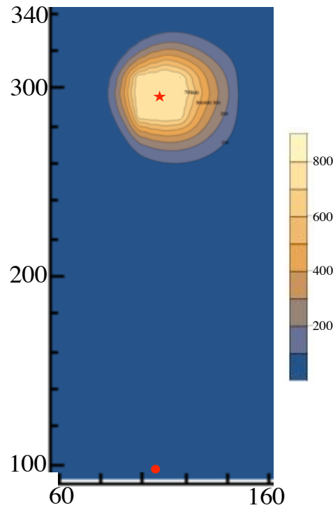
Figure 5.11: Case 7 of AdVF simulation profile after 2D transport model in Katsura River Basin with 0.164 \text{ day}^{-1} reduction rate coefficient; ★ denotes the injection point, • denotes the withdrawal point; x-and y-axes show the distance values in meters
