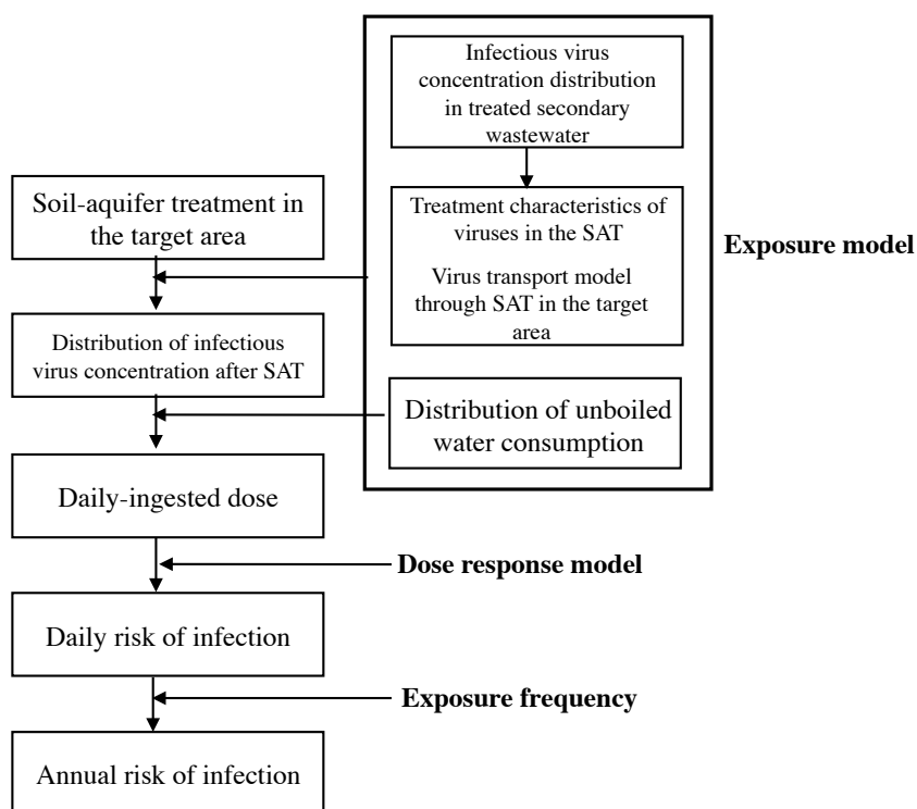
Figure 6.1: The procedure to estimate the expected annual infection risk from consumption of effluent-treated secondary sewage by SAT
