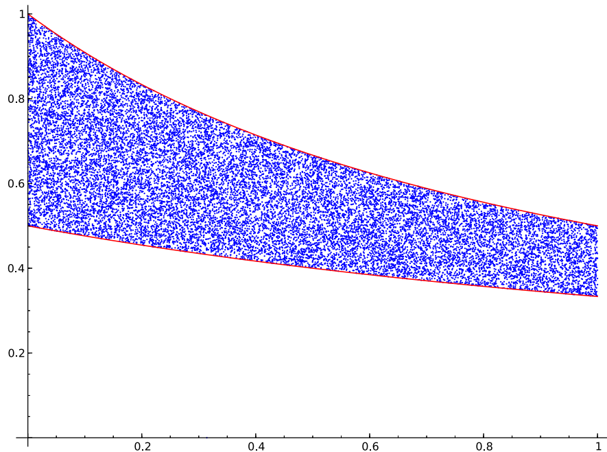
Figure 3. 20 000 points of an orbit of \tilde{S}
