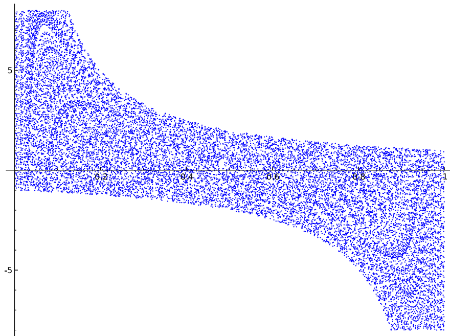
Figure 7. 50 000 points of an orbit of the natural extension of Farey continued fraction
