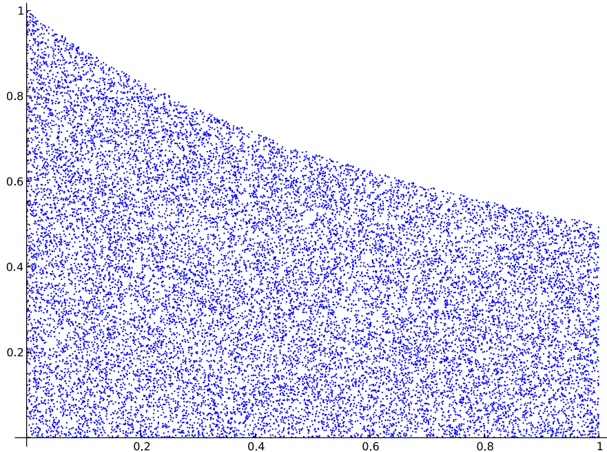
Figure 1. 20 000 points of an orbit of \tilde{T}
