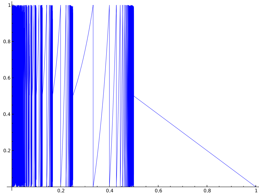
Figure 4. The graph of Ralston continued fraction g
