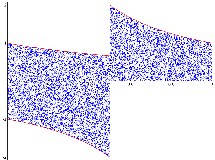
Figure 5. 20 000 points of an orbit of \tilde{g}
