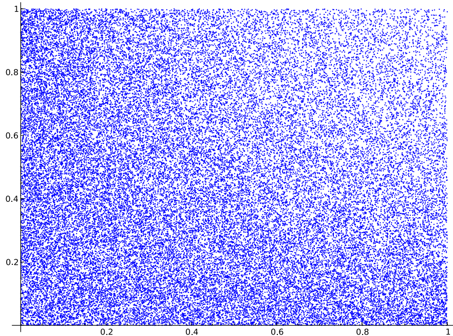
Figure 2. 50 000 points of an orbit of \overline{T}
