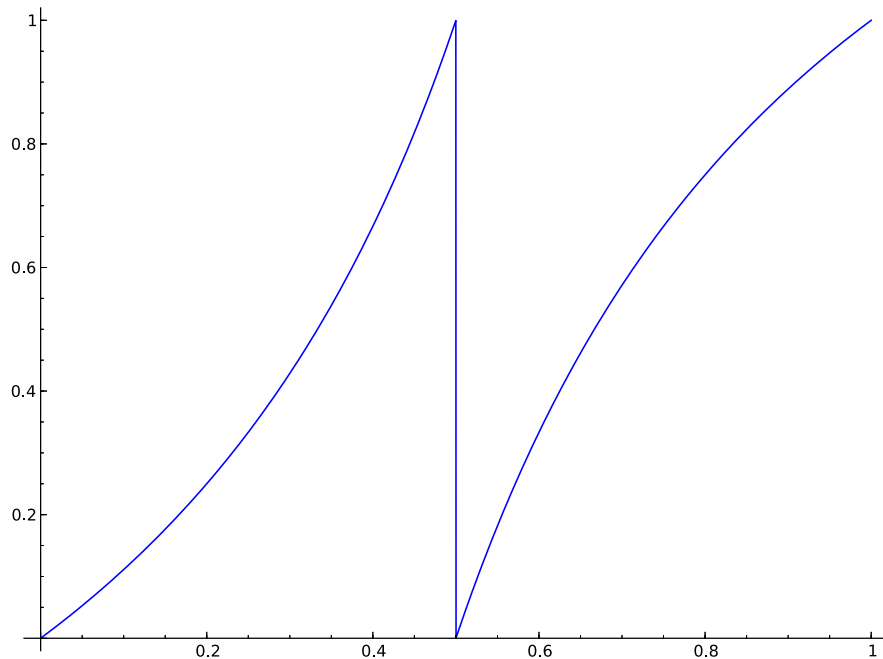
Figure 6. The graph of the Farey continued fraction g
