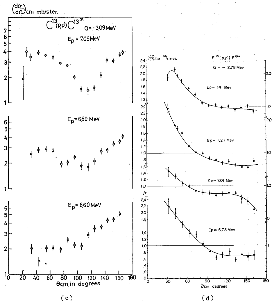
Fig. 4-2-1. Angular distributions of protons scattered inelastically from several odd-A elements. (a) \text{Be}^9 , 2.43 MeV state. (b) \text{B}^{11} , 2.13 MeV state. (c) \text{C}^{13} , 3.09 MeV state and (d) \text{F}^{19} , 2.78 MeV state.
