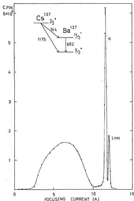
Fig. 3-4-1. Beta-ray spectrum of Cs 137 obtained by the thin lens spectrometer.
