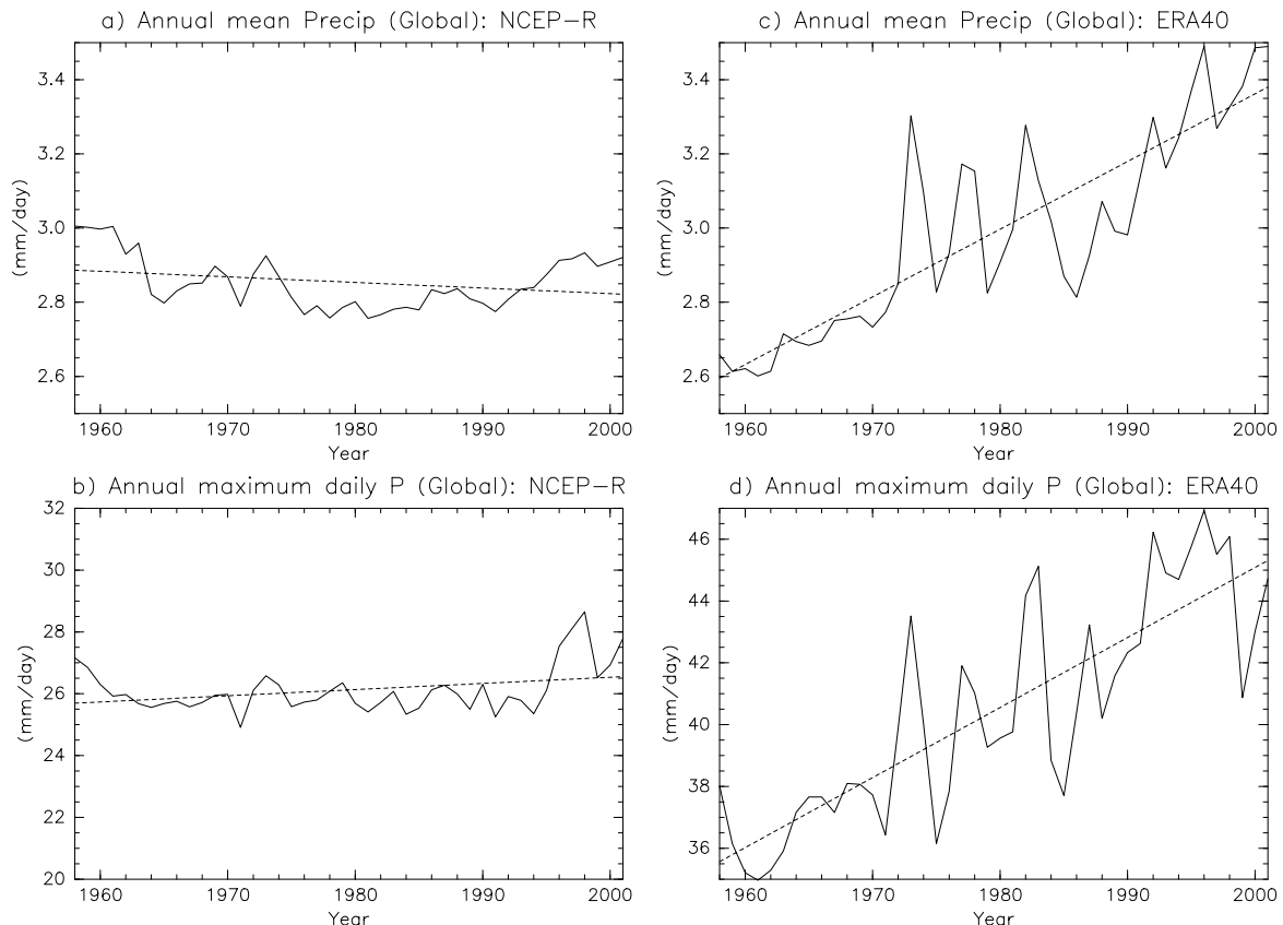
Fig. 4 Time evolution of globally averaged annual mean precipitation rates (a and c) and annual maximum daily precipitation rates (b and d), obtained from the NCEP reanalysis (a and b) and the ERA40 (c and d). The dashed lines show a linear least-square regression.
