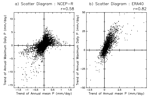
Fig. 9 Scatter diagrams between the linear trend of annual mean and annual maximum daily precipitation rates for a) the NCEP reanalysis and b) ERA40.
