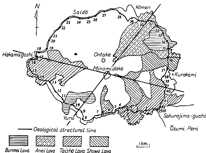
Fig. 1. The position of benchmarks and the distribution of the lava-flow in history in Sakurajima.
