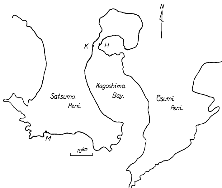
Fig. 7. The locations of the tidal gauge stations. H: Hakamagoshi. K: Kagoshima. M: Makurazaki.
