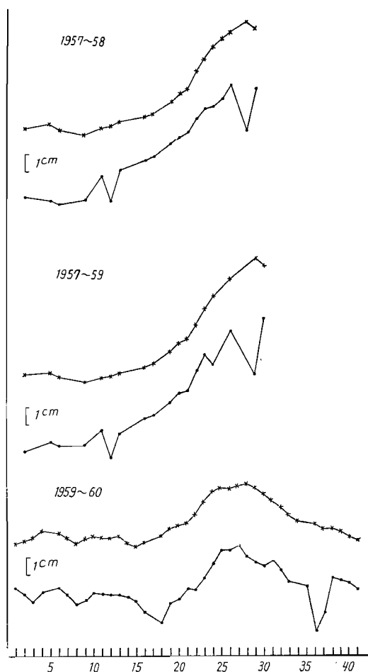
Fig. 5. The relation between the measured and the calculated vertical displacements of benchmarks in Sakurajima in the each period.
