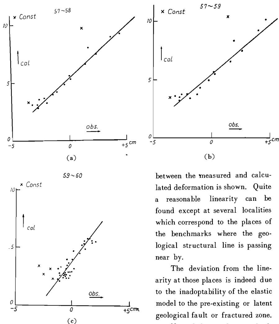
Fig. 6.** The linearity of the relation between the measured and the calculated vertical displacements of benchmarks in Sakurajima. × are abnormally depressed points.
