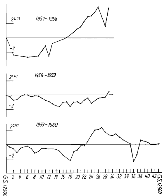
Fig. 2. The vertical displacement of benchmarks in the respective periods.
