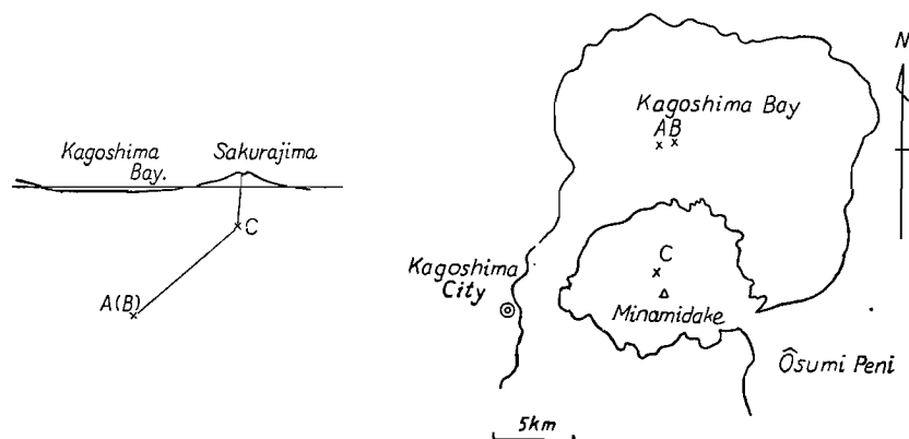
Fig. 4. The position of the pressure center.
