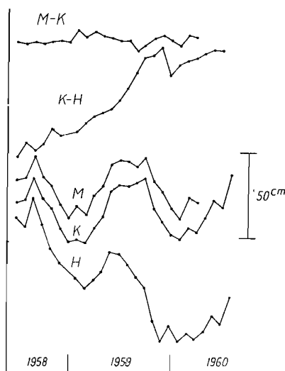
Fig. 8. The changes of the monthly mean values of the sea-level at each station, and the changes of the differences of these values between two stations. H Hakamagoshi. K Kagoshima. M . Makurazaki.
