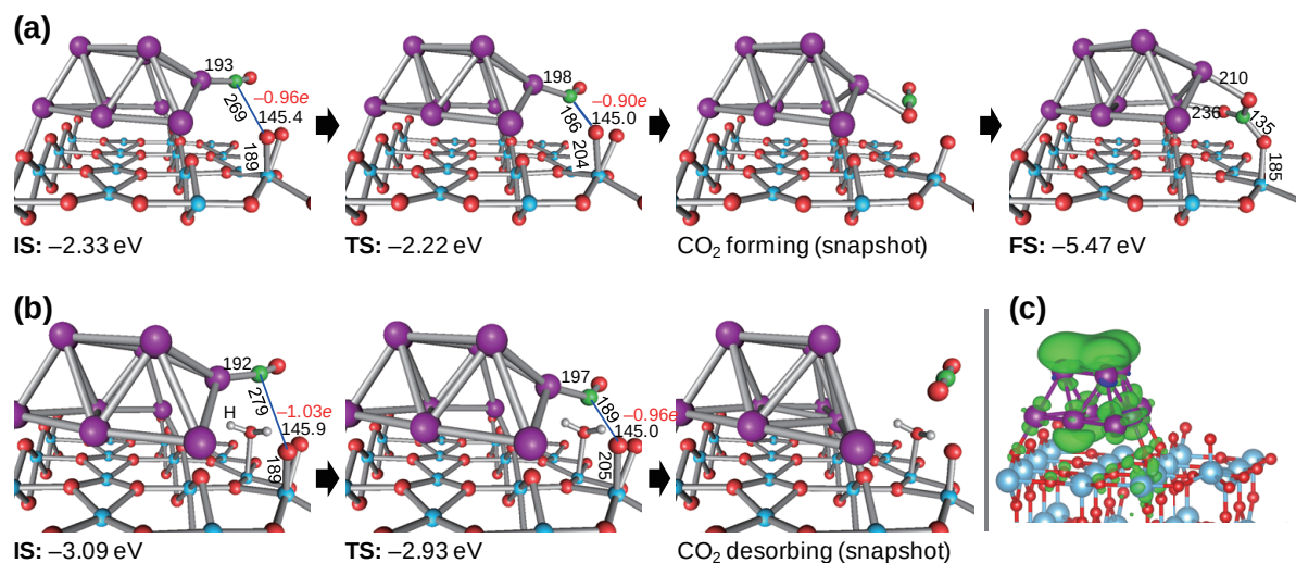
FIG. 6. Ti(2,1)-O_2 + Au-CO reaction over Au_9/TiO_2 . Adsorption energies, interatomic distances (pm), and Bader charges on O_2 are displayed in the figure. (b) Same with H_2O adsorbed next to O_2 . (c) Spin charge density plot for Au_9/TiO_2 with an O adatom on Ti(2,1) . Green and blue surfaces are isosurfaces drawn at +0.001e/Bohr^3 and -0.001e/Bohr^3 , respectively.
