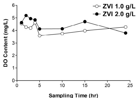
Fig. 9: DO variation with time (As 0.2 mg/L, control pH & ZVI type KB-90)
