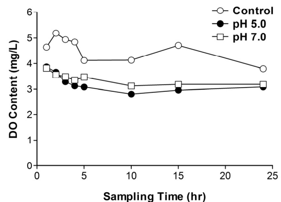
Fig. 8: DO variation with time (As 0.2 mg/L & ZVI (KB-90) 2.0 g/L)
