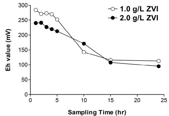
Fig. 7: Eh variation with time (As 0.2 mg/L, control pH & ZVI type KB-90)
