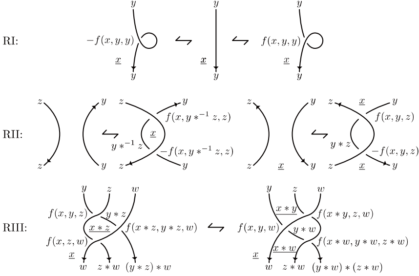
Figure 12: Reidemeister moves do not change the weights of shadow colorings of the diagrams.
