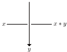
Figure 1: The condition for an X -coloring.
