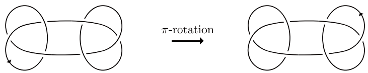
Figure 17: Deformation 5 of GK .
