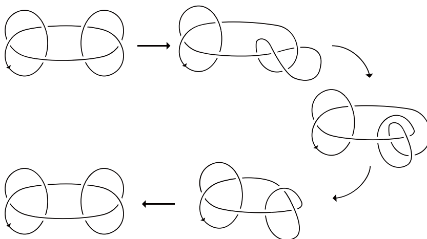
Figure 7: Deformation 2 of SK .
