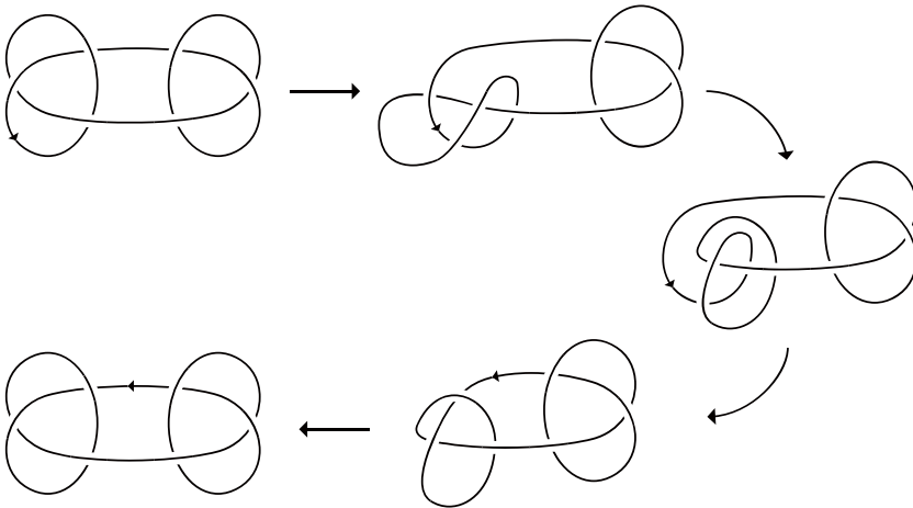
Figure 6: Deformation 1 of SK .
