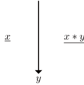
Figure 10: The condition for a region coloring.
