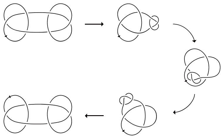
Figure 16: Deformation 4 of GK .
