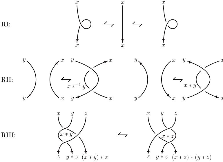
Figure 3: Reidemeister moves relate X -colorings of the diagrams uniquely.
