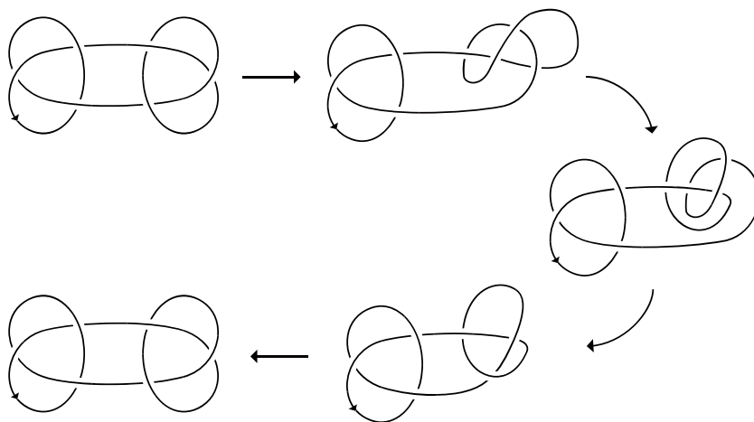
Figure 14: Deformation 2 of GK .
