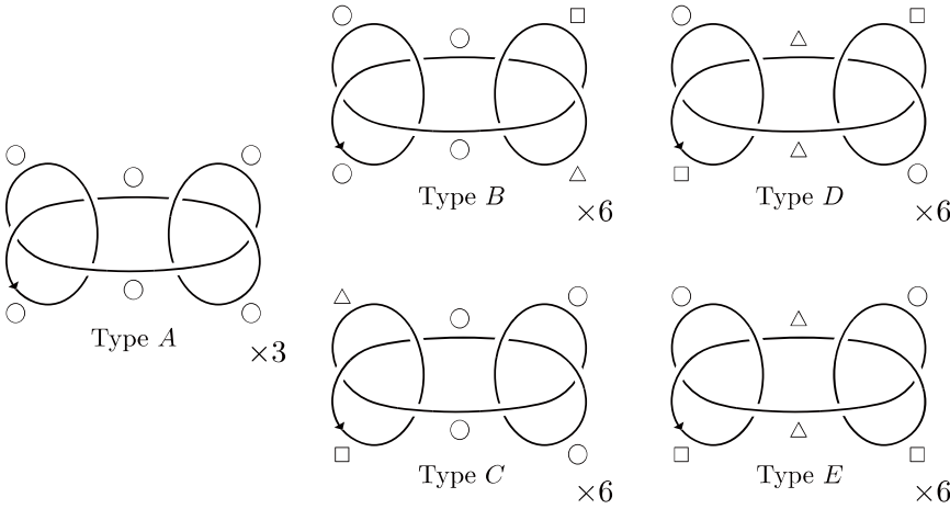
Figure 5: The R_3 -colorings of the diagram SK of the square knot.
