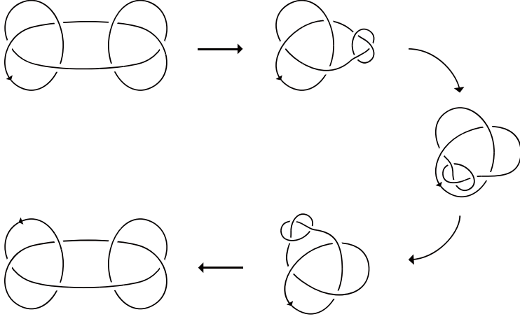
Figure 9: Deformation 4 of SK .
