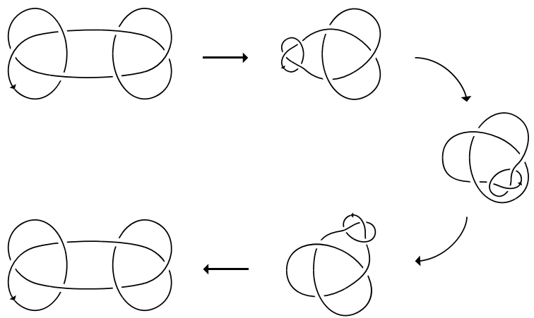
Figure 15: Deformation 3 of GK .
