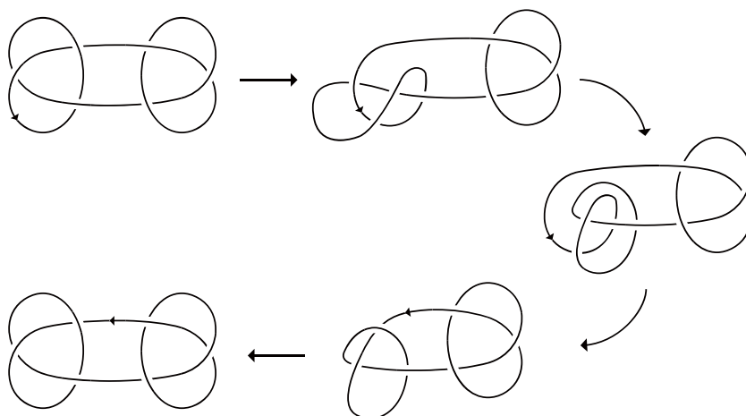
Figure 13: Deformation 1 of GK .
