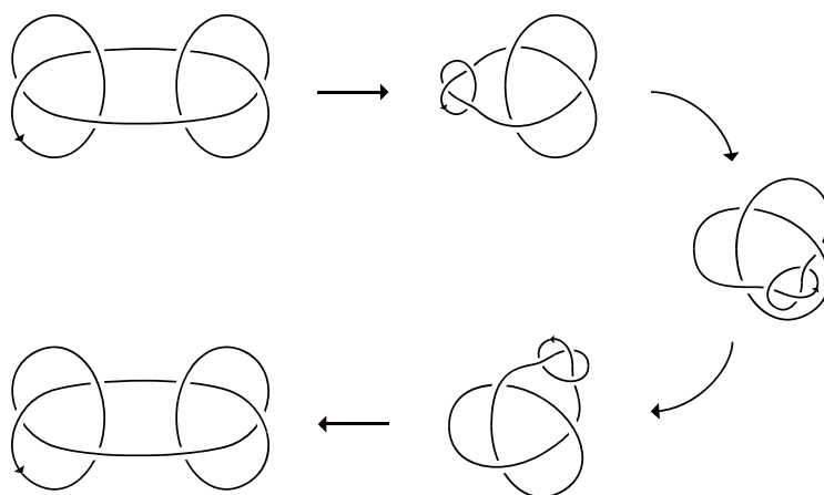
Figure 8: Deformation 3 of SK .
