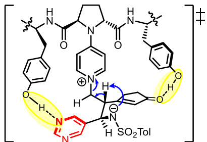
Fig. 3-2. Hypothetical conformational fixation by two attractive interactions
