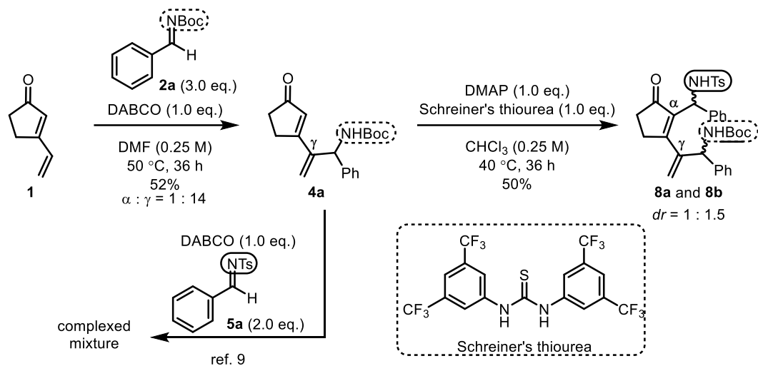
Scheme 2-10. double aza-MBH reaction via sequential incorporation of imines
