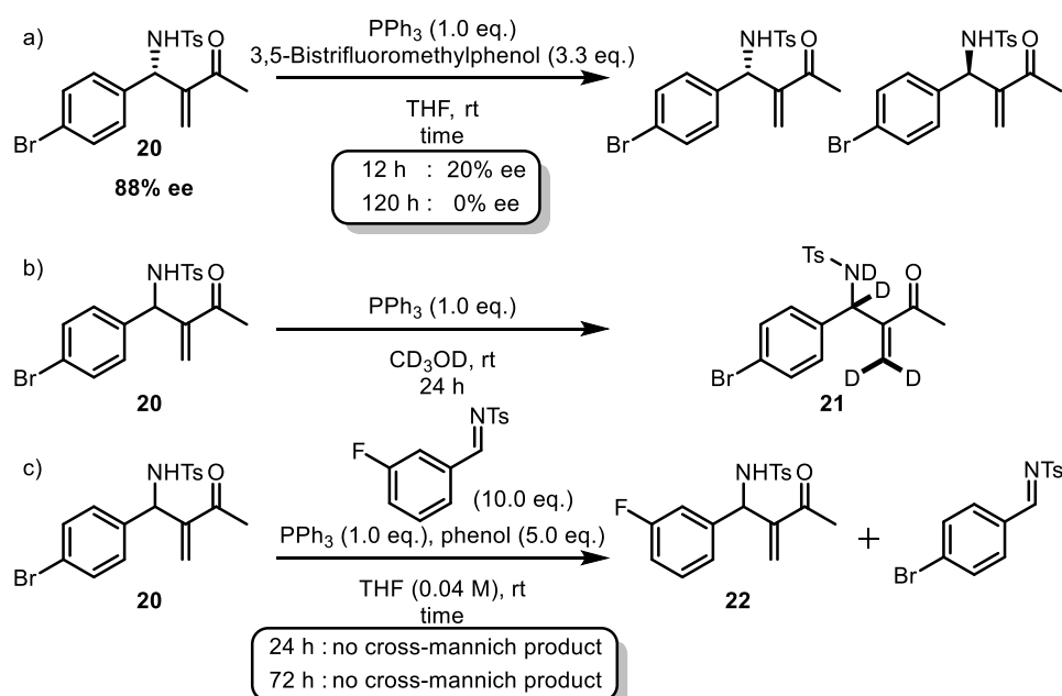
Scheme 3-8. Deprotonation of allylic C-H bond by \text{PPh}_3
