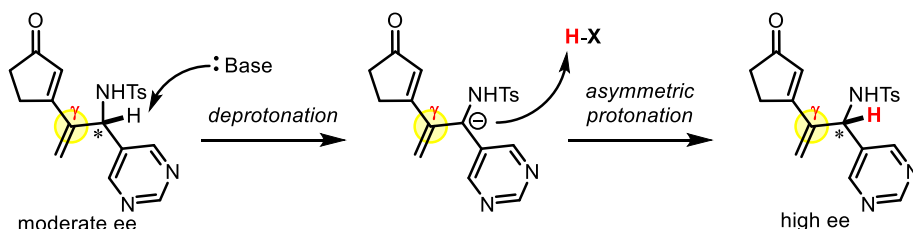
Scheme 3-10. Possible explanation for increase in ee
