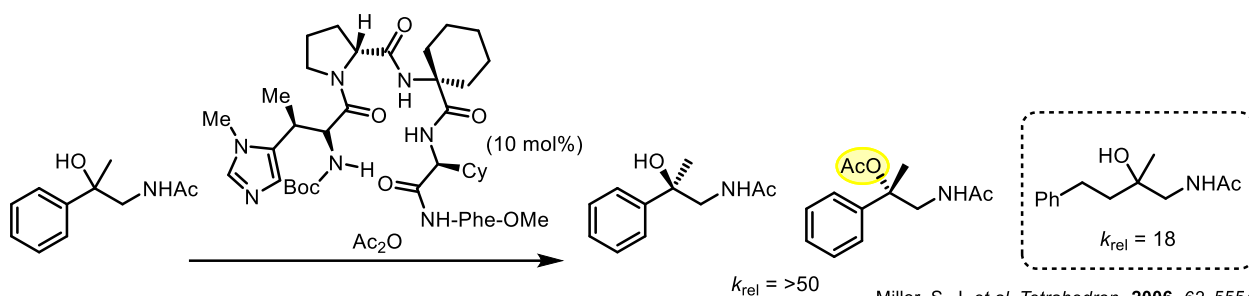
Scheme 5-1. Kinetic resolution of tert -alcohol by peptide catalyst
