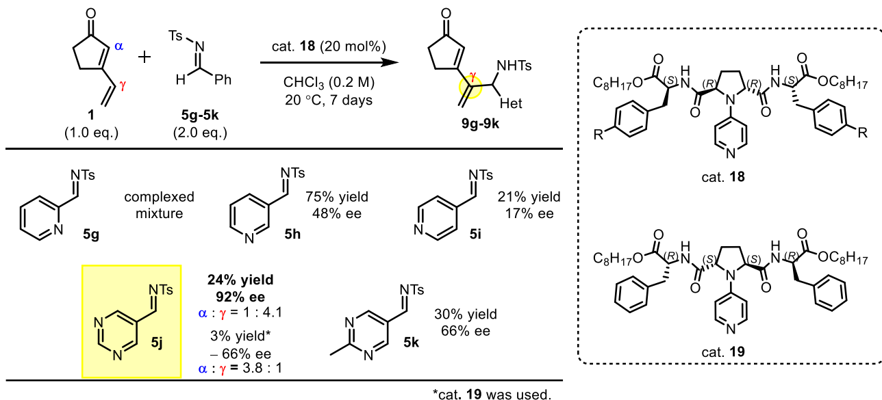
Scheme 3-6. Substrate optimization of pyridine or pyrimidine analogue
