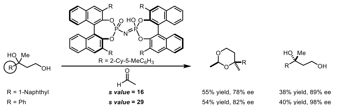
Scheme 5-4. Kinetic resolution of 1,3-diols with a tertiary hydroxy group
