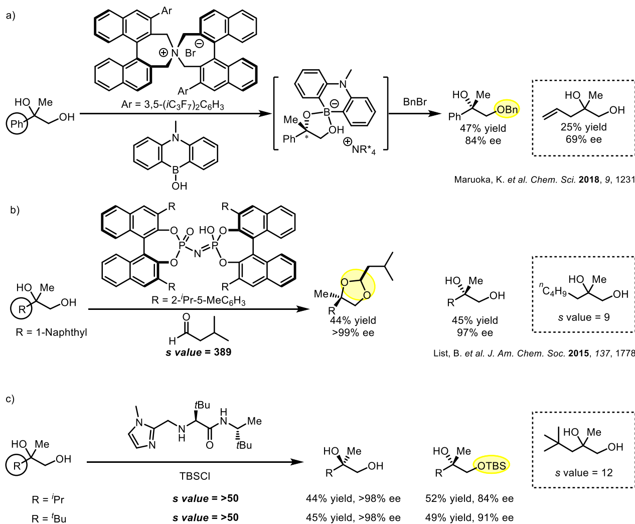
Scheme 5-3. Kinetic resolution of 1,2-diols with a tertiary hydroxy group
