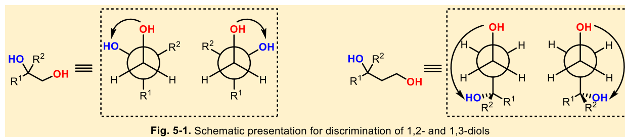
Fig. 5-1. Schematic presentation for discrimination of 1,2- and 1,3-diols
