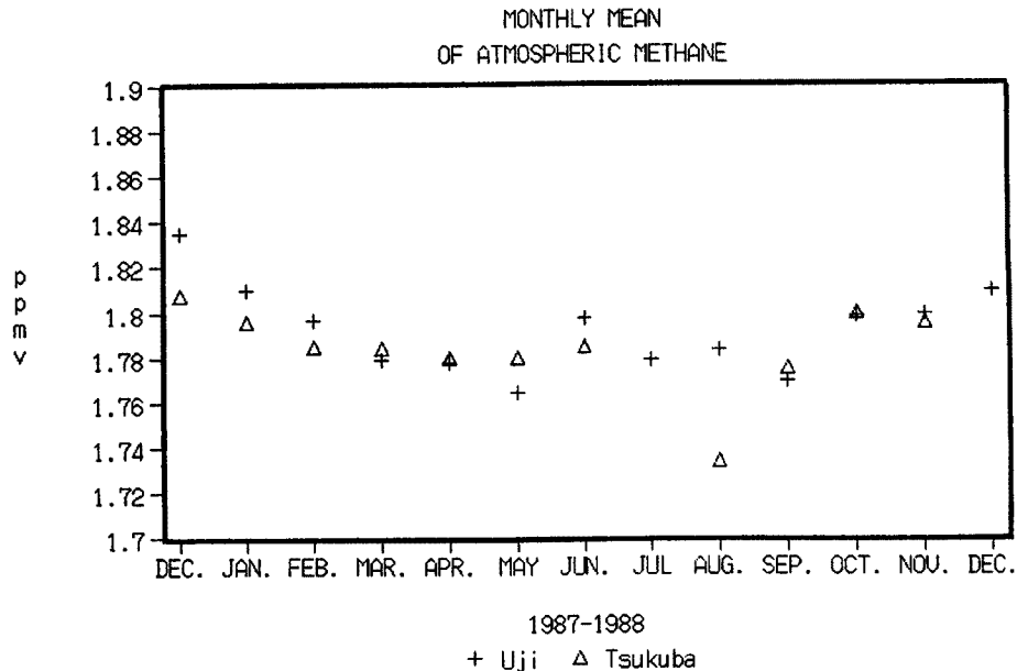
Fig. 2. Monthly mean of atmospheric methane.
