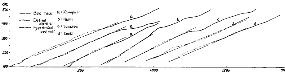
Fig. 8 Relations among slopes, bed-rocks and detrital materials
