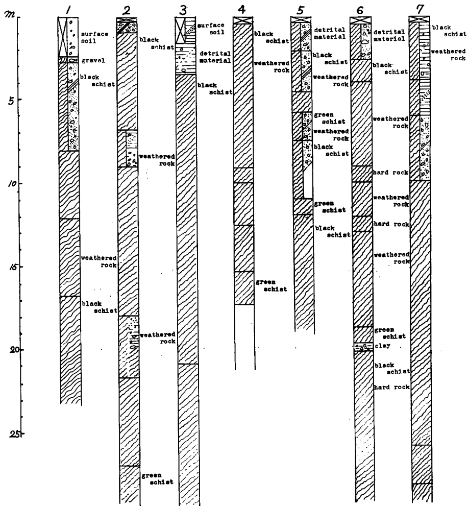
Fig. 9 Columnar sections in Kunimasa's landslide area
