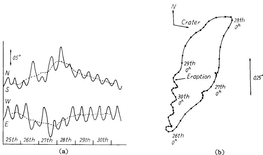
Fig. 8 (a) Abnormal tilt before the eruption on the 29th, March 1960
