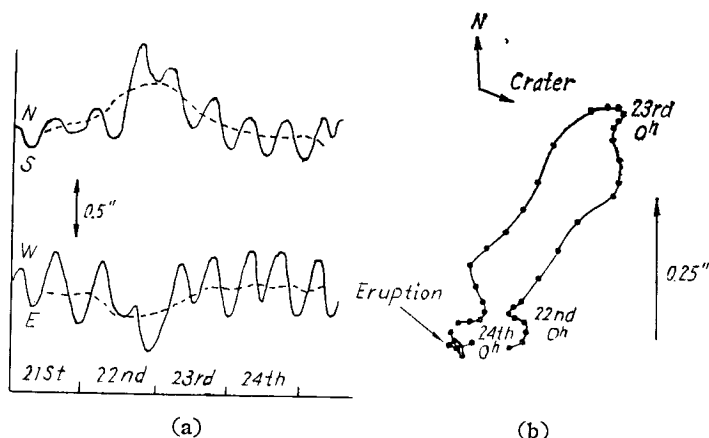
Fig. 7 (a) Abnormal tilt before the eruption on the 24th, Feb. 1959
