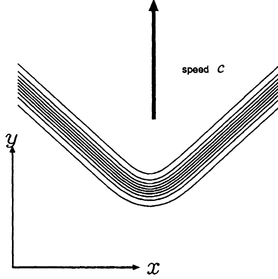
Figure 4: Contour lines of a two-dimensional V-form wave v_*(x, y) ([17]).
