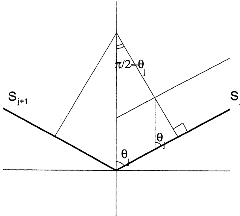
Figure 7: The angle between surfaces S_j and S_{j+1}
