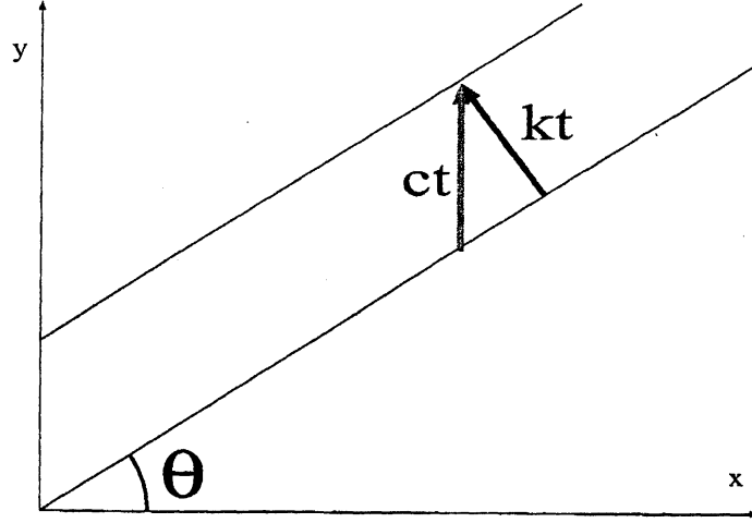
Figure 5: For a two-dimensional V-form front one has \tan \theta = \frac{\sqrt{c^2 - k^2}}{k} .
