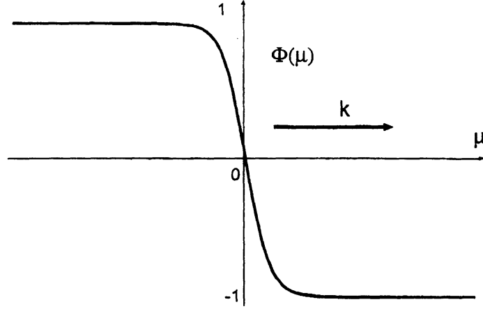
Figure 1: One-dimensional traveling wave \Phi
