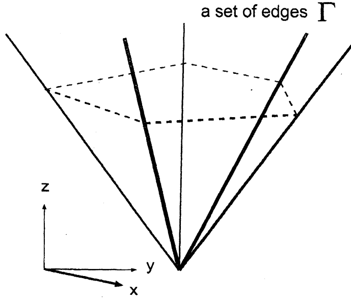
Figure 2: The edge lines \Gamma
