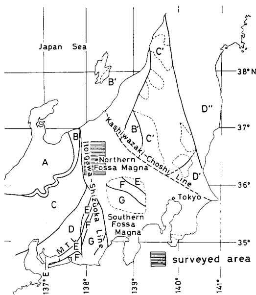
Fig. 1. Index map of the surveyed area.
