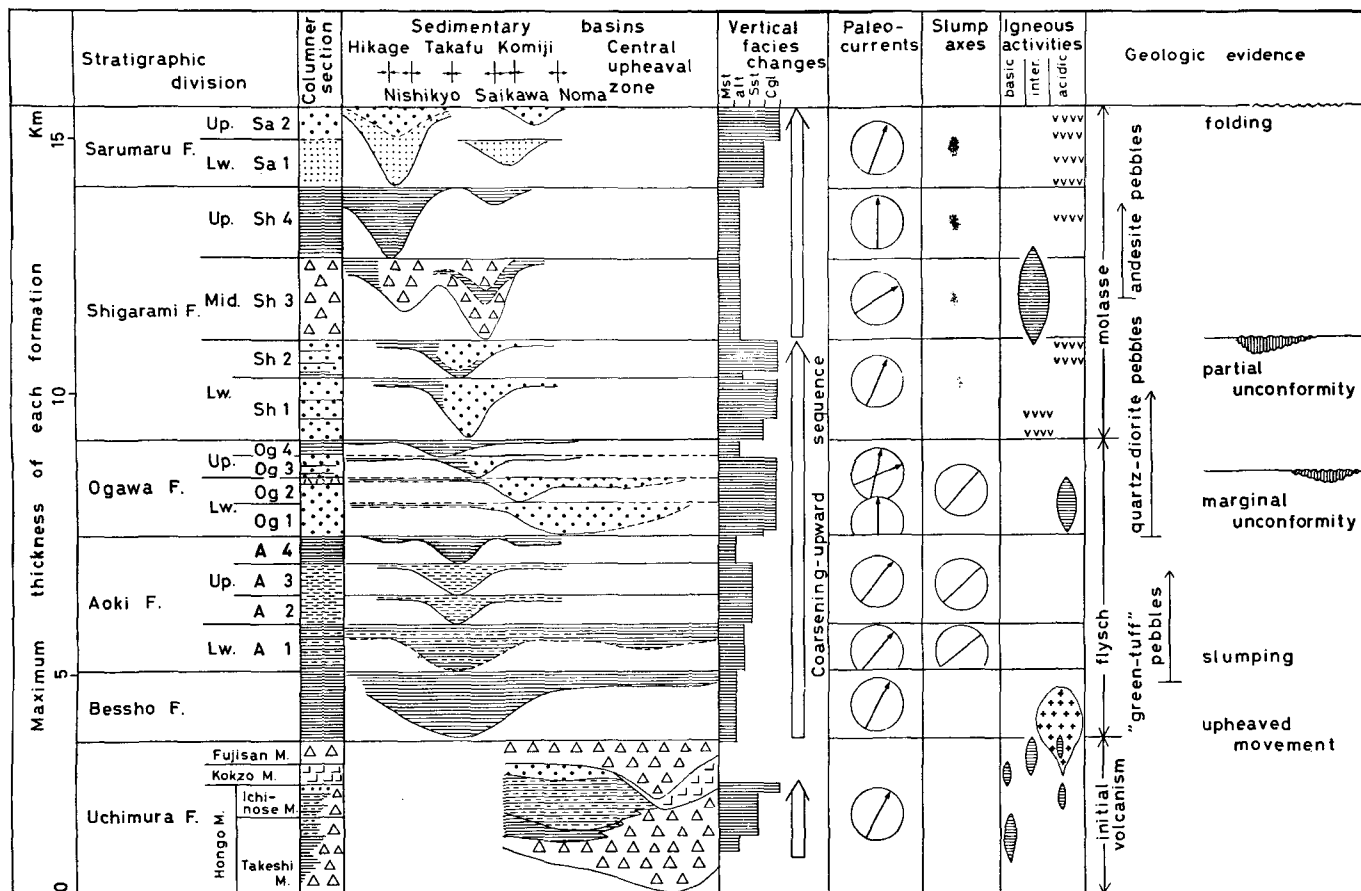
Fig. 13. Schematic relations of vertical facies changes, paleocurrents, slump axes and igneous activities of the Neogene sedimentary basins.
