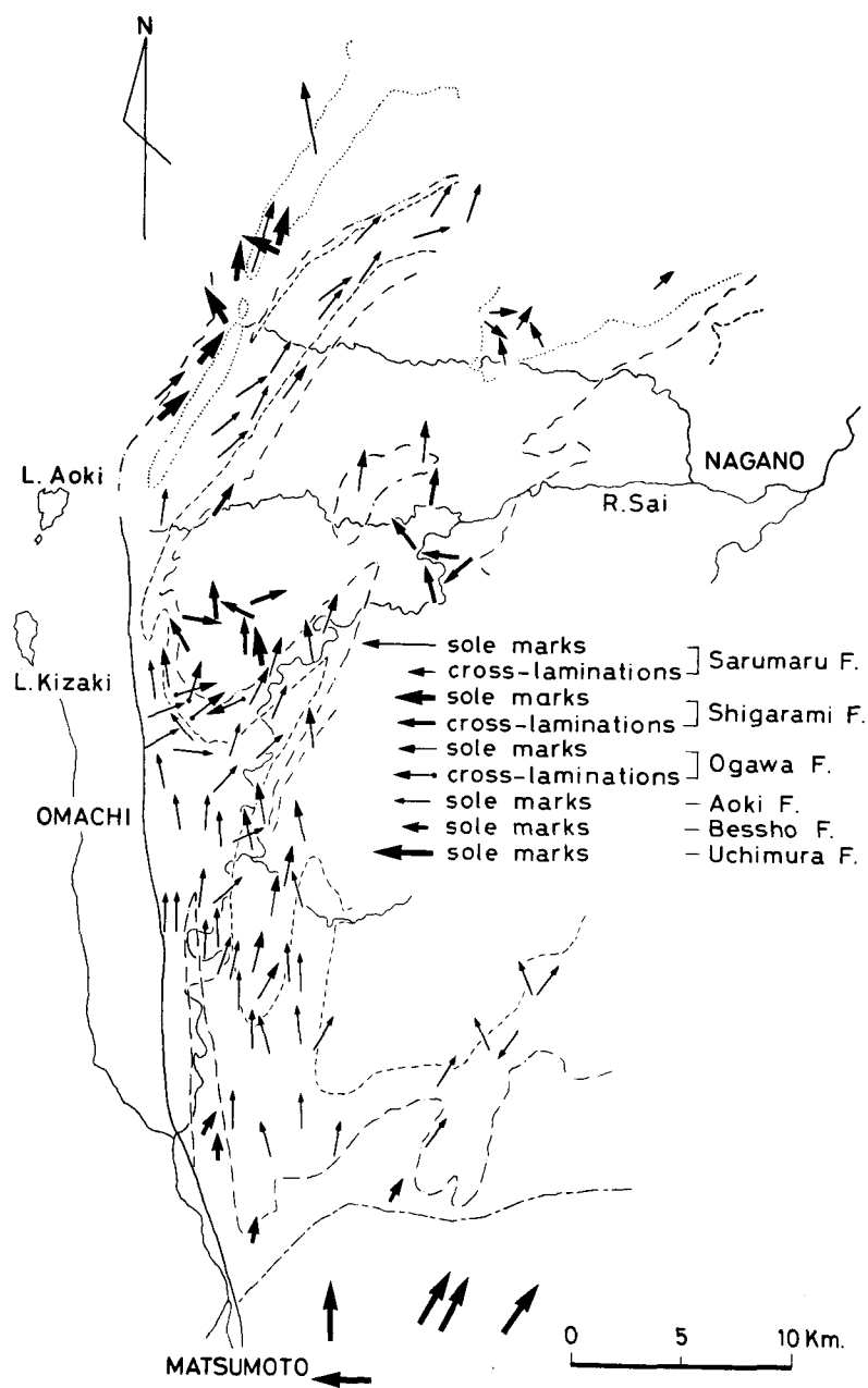
Fig. 9a. Paleocurrent direction of each Formation.
