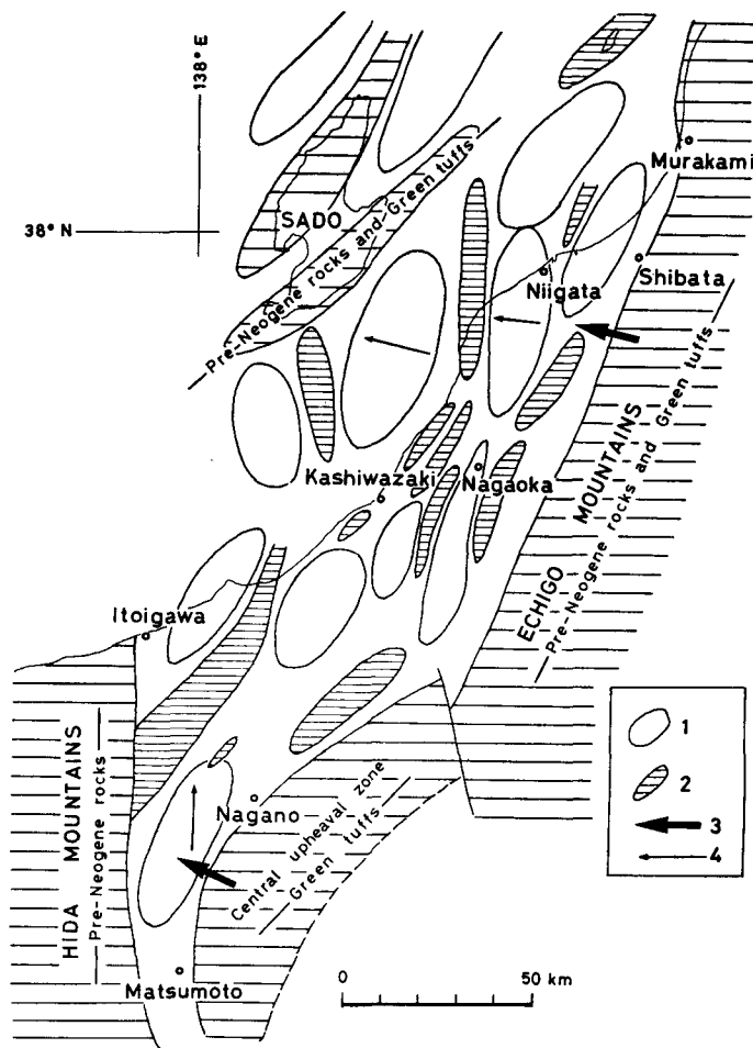
Fig. 15. Structure of the Shin'etsu mega-sedimentary basin. The southernmost sedimentary basin is a surveyed area.
