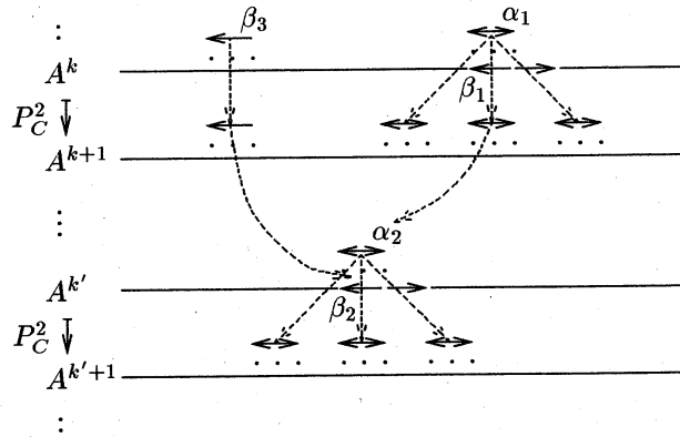
Figure 6: Proof of lemma 5.5
