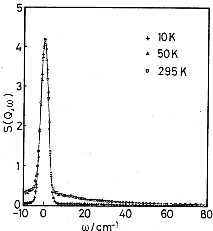
Fig. 2. Dynamic scattering laws S(Q, \omega) of TPC at 10K (+), 50K ( \Delta ) and 295K ( \circ ), normalized by the elastic peak intensity.
