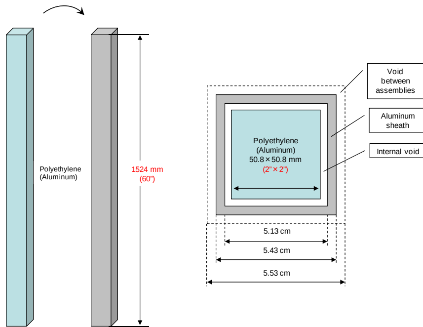
Fig. 1-5 Description of polyethylene reflector at KUCA
