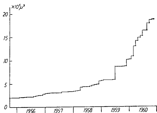
Fig. 1 Successive accumulation of the square of maximum amplitude of eruption earthquake.
