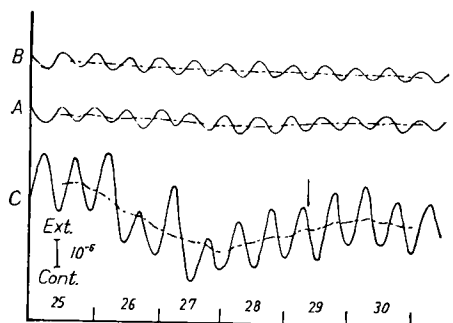
Fig. 7(c) Abnormal vertical contraction at Hakamagoshi on the occasion of the eruption on 29th of Mar., 1960.
