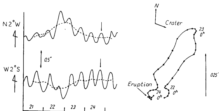
Fig. 8 Abnormal tilt at Hakamagoshi on the occasion of the eruption on 24th of Feb., 1959.
