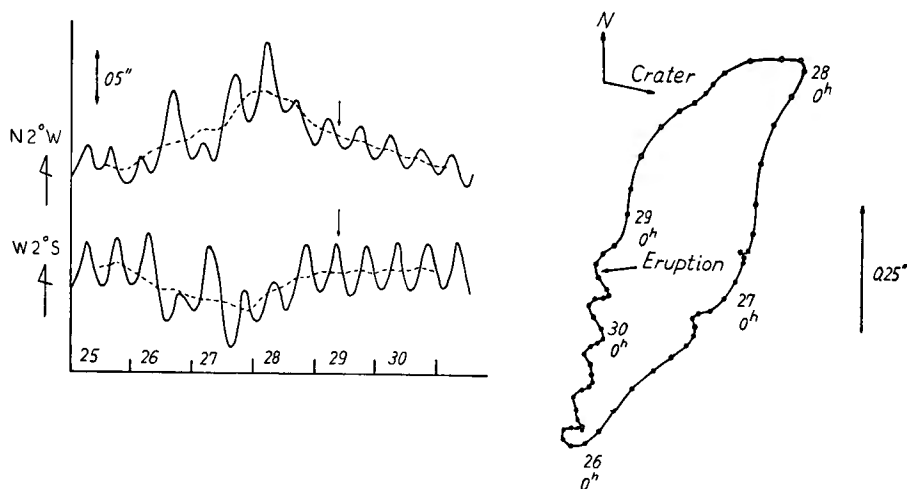
Fig. 7(a) Abnormal tilt at Hakamagoshi on the occasion of the eruption on 29th of Mar., 1960.
