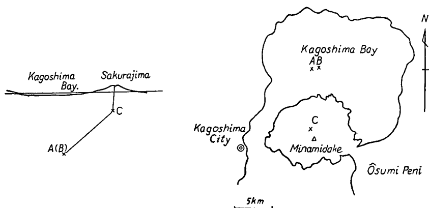
Fig. 5 The position of the pressure center.
