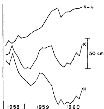
Fig. 6 The change of the monthly mean values of the sea-level, and the change of the differences of these values between two stations.
