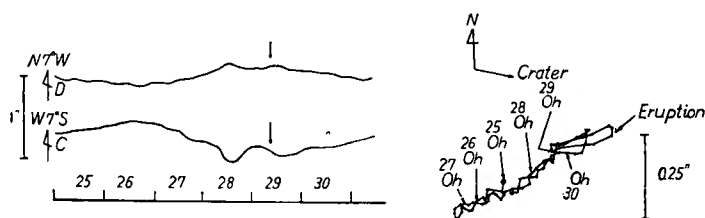
Fig. 7(b) Abnormal tilt at Hi Yamizu on the occasion of the eruption on 29th of Mar., 1961.
