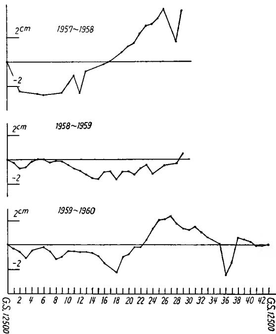
Fig. 3 The vertical displacement of benchmarks in the respective periods.
