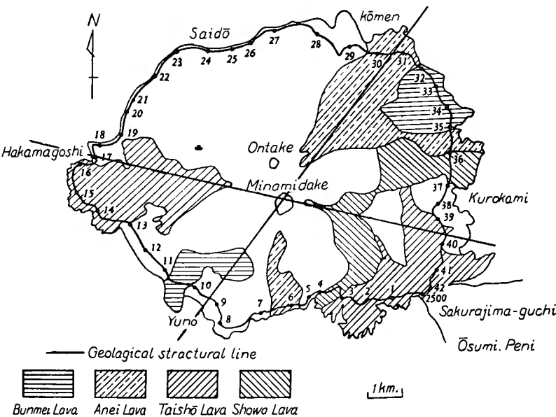
Fig. 2 The position of benchmarks and the distribution of the lava-flow in history in Sakurajima.
