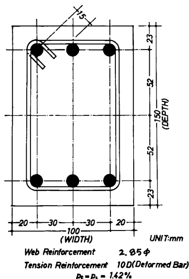
Fig. 2 Column cross section.
