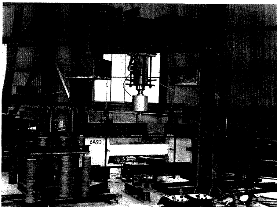
Photo. Test set-up.
