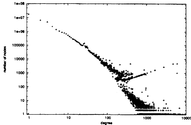
Figure 2: Degree distribution of the undirected webgraph.
