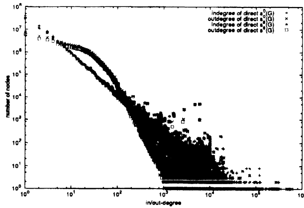
Figure 7: Degree distribution of is-contracted directed webgraphs.
