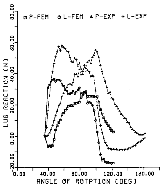
Fig.6-9. Soil reaction by RPFEM for CASE-I.
