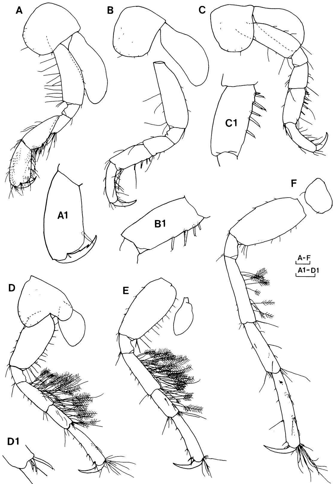
Fig. 22. Aoroides myojinensis sp. nov. Male (holotype), 3.5mm: A, gnathopod 2; A1, articles 6-7 of gnathopod 2; B, pereopod 3; B1, article 5 of pereopod 3; C, pereopod 4; C1, article 5 of pereopod 4; D, pereopod 5; D1, distal end of pereopod 5 article 5; E, pereopod 6 (coxal plate damaged); F, pereopod 7. Scale: 0.1mm.
