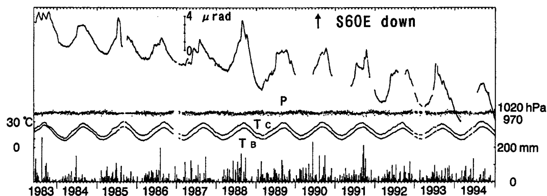
Fig. 4. Daily mean values of hourly sampling data: The uppermost graph shows tilting (upward indicates ground tilting toward the Suruga trough), the center graphs show atmospheric pressure (P) and air-temperature in the cellar ( T_B : the site B, T_C : the middle of both the site), respectively. Daily precipitation at Makinohara (by Japan Meteorological Agency) are shown on the bottom.
