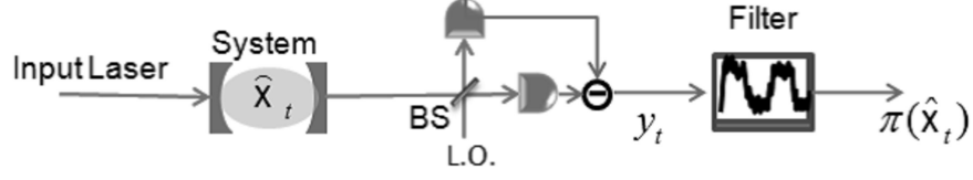
Fig. 1 Schematic of the quantum Kalman filter. First, the system couples with an input laser. The output laser is mixed, by a beam splitter (BS), with a strong reference light called the local oscillator (LO), and two outputs are then respectively detected via a photon detector. This whole measurement configuration is called the homodyne detection. Finally, the quantum Kalman filter uses the output to calculate the best estimation \pi(\hat{x}_t) .
