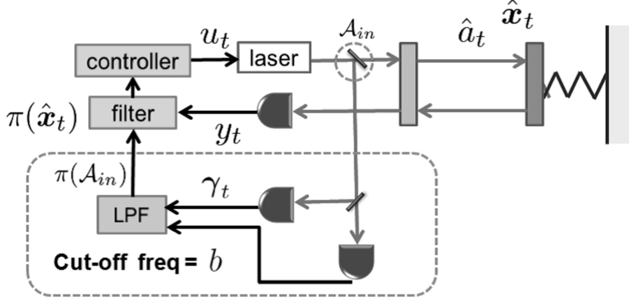
Fig 3 Schematic of the adaptive quantum Kalman filter and LQG controller.
