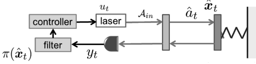
Fig. 2 Schematic of the optomechanical oscillator. The right end mirror of the Fabry-Perot cavity serves as the oscillator, where \hat{x}_t is the system variable, \hat{a}_t is an annihilation operator corresponding to the intra-cavity, and \mathcal{A}_{in} is the mean amplitude of the input laser.
