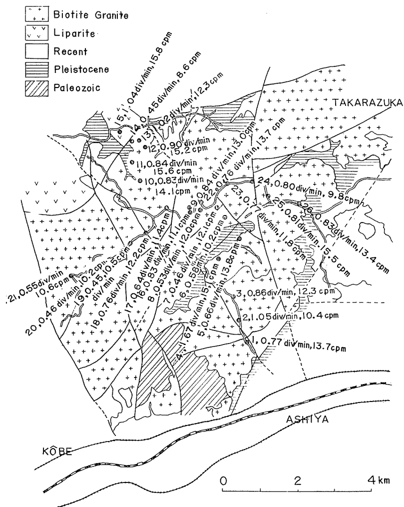
Fig. 3. Distribution of radioactivity (Rokkō).
