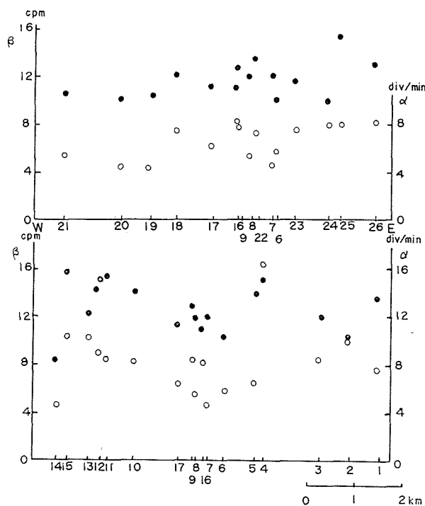
Fig. 4-3. Plot of the alpha-radioactivity ( \circ ) and beta-radioactivity ( \cdot ) across Rokkô intrusive mass,
