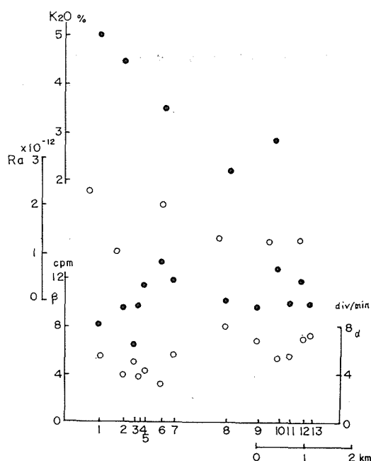
Fig. 4-1. Plot of the alpha-radioactivity ( \circ ), beta-radioactivity ( \bullet ), Ra content ( \circ ) and K_2O content ( \bullet ) across Kitashirakawa intrusive mass.
