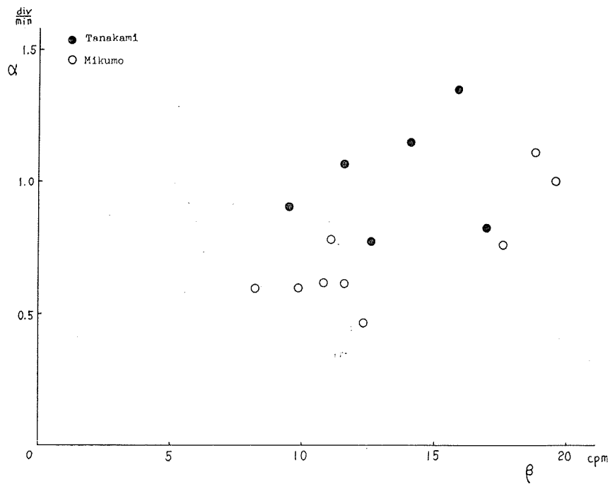
Fig. 5-2. Relation between alpha-radioactivity and beta-radioactivity (Tanakami-Mikumo).
