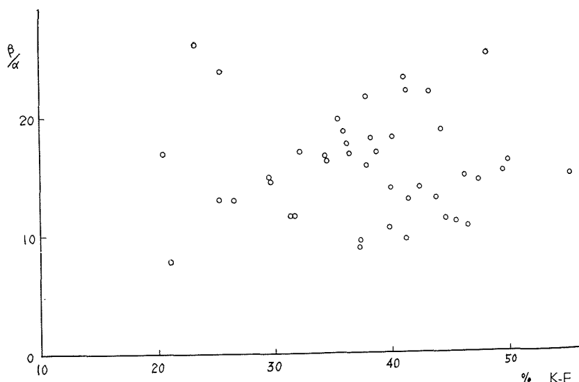
Fig. 9. Scatter diagram \beta/\alpha ratio vs. potash-feldspar.
