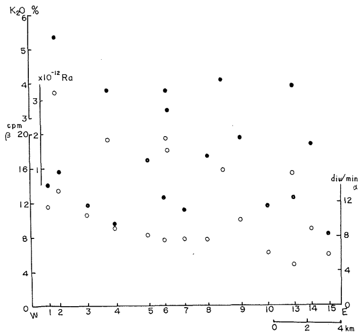
Fig. 4-2. Plot of the alpha-radioactivity ( \circ ), beta-radioactivity ( \cdot ), Ra content ( \circ ) and K_2O content ( \cdot ) across Tanakami-Mikumo intrusive mass.
