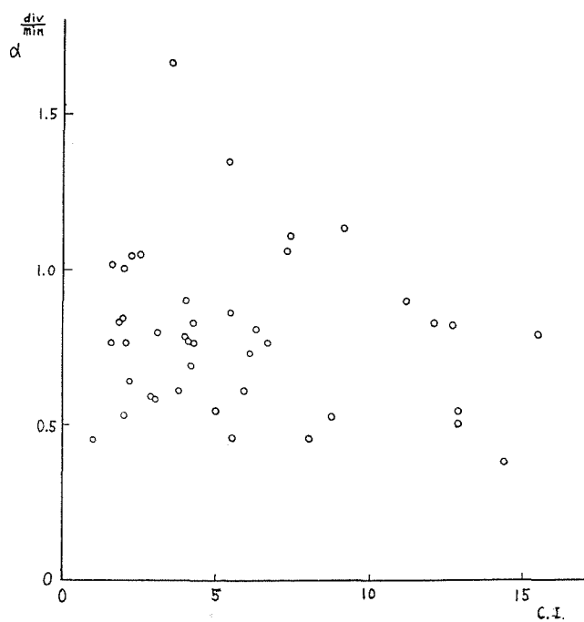
Fig. 7-1. Relationship between alpha-radioactivity and colour index.
