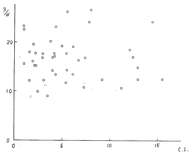
Fig. 7-3. Relationship between \beta/\alpha ratio and colour index.
