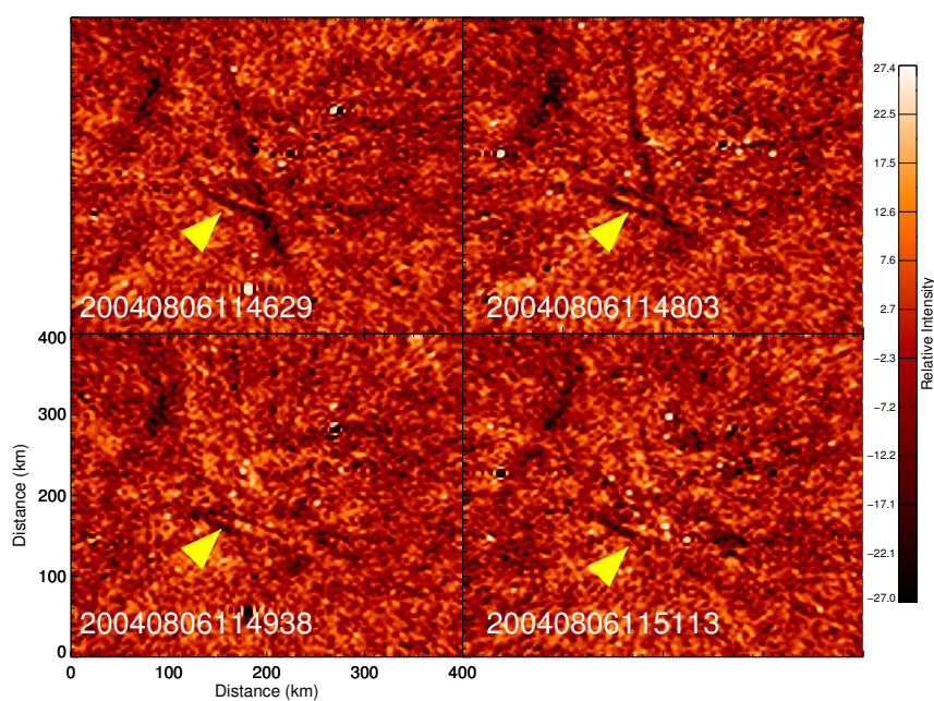
Figure 1. Processed Na image from August 6, 2004. The images were unwarped onto a 400 x 400 km geographic grid (shown in the bottom left image) with the positive y-axis corresponding to 0° longitude. Yellow arrows mark the location of the observed wave in each image. Time stamps are shown in the bottom left of each image, and is read as YYYYMMDDHHMMSS. The sequence of images starts at the top left, and follows to the top right, bottom left, and finally bottom right.
