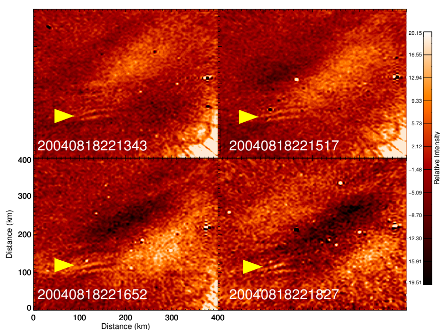
Figure 2. Processed Na image from August 18, 2004. The images were unwarped onto a 400 x 400 km geographic grid (shown in the bottom left image) with the positive y-axis corresponding to 0° longitude. Yellow arrows mark the location of the observed wave in each image. Time stamps are shown in the bottom left of each image, and is read as YYYYMMDDHHMMSS. The sequence of images starts at the top left, and follows to the top right, bottom left, and finally bottom right.
