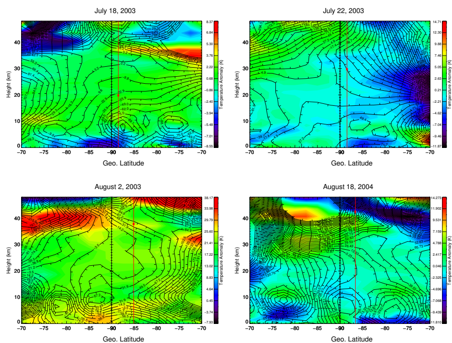
Figure 7. 24-hr time differenced contour plots of geopotential height (black contours) and temperatures obtained from ECMWF Reanalysis from 0-50 km along the direction of the ray path for waves observed on July 18, 2003 (top left), July 22, 2003 (top right), August 2, 2003 (bottom left) and August 18, 2004 (bottom right), as determined by our GROGRAT model runs. Ticks on contour lines point to lower geopotential height. Vertical red lines mark the latitude at which the rays terminate, and the corresponding red 'X' denotes the location of the wave source.
