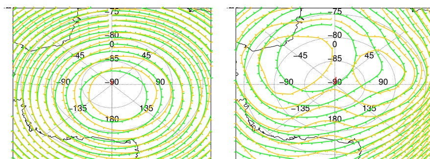
Figure 3. (left) Results of the GROGRAT “climatological” run for the wave observed on August 06, 2004 using background pressures, temperatures, and horizontal winds reconstructed from NRLMSISE-00 and HWM-93. (right) Results of the GROGRAT run for the same wave using an atmosphere constructed from ECMWF Reanalysis below 50 km altitude and NRLMSISE-00 and HWM-93 between 50 km and 100 km altitude. The two contours in each panel represent geopotential heights at 3 mbar (orange) and 10 mbar (green), and the red line in each panel represents the wave ray path.
