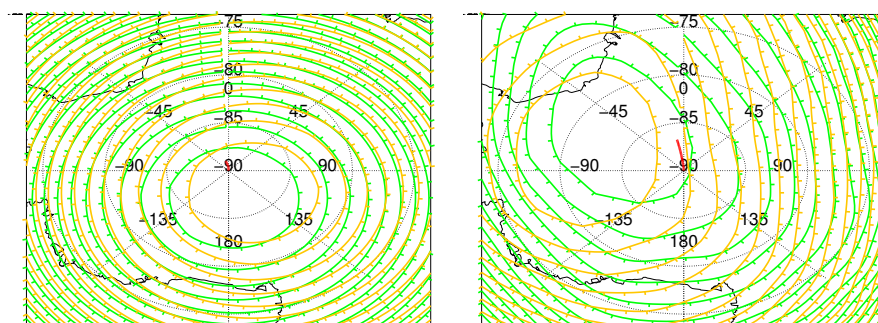
Figure 4. (left) Results of the GROGRAT "climatological" run for the wave observed on August 18, 2004 using background pressures, temperatures, and horizontal winds reconstructed from NRLMSISE-00 and HWM-93. (right) Results of the GROGRAT run for the same wave using an atmosphere constructed from ECMWF Reanalysis below 50 km altitude and NRLMSISE-00 and HWM-93 between 50 km and 100 km altitude. The two contours in each panel represent geopotential heights at 3 mbar (orange) and 10 mbar (green), and the red line in each panel represents the wave ray path.
