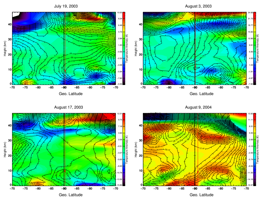
Figure 8. 24-hr time differenced contour plots of geopotential height (black contours) and temperatures obtained from ECMWF Reanalysis from 0-50 km along the direction of the ray path for waves observed on July 19, 2003 (top left), August 3, 2003 (top right), August 17, 2003 (bottom left) and August 9, 2004 (bottom right), as determined by our GROGRAT model runs. Ticks on contour lines point to lower geopotential height. Vertical red line marks the latitude at which the ray terminates, and the corresponding red 'X' denotes the location of the wave source.
