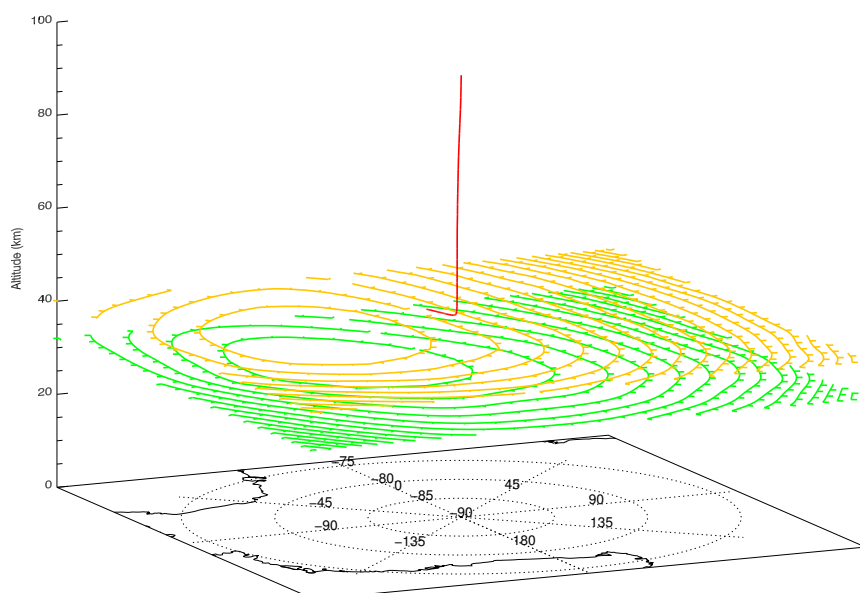
Figure 5. GROGRAT ray-tracing results for the August 19, 2004 wave projected in 3-D over Antarctica. The two contours represent geopotential heights at 3 mbar (orange) and 10 mbar (green), and show the wave ray path (red line).
