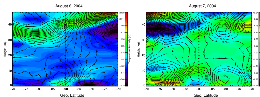
Figure 9. 24-hr time differenced contour plots of geopotential height (black contours) and temperatures obtained from ECMWF Reanalysis from 0-50 km along the direction of the ray path of the August 6, 2004 (left) and August 7, 2004 (right) waves, as determined by GROGRAT. Ticks on contour lines point to lower geopotential height.
