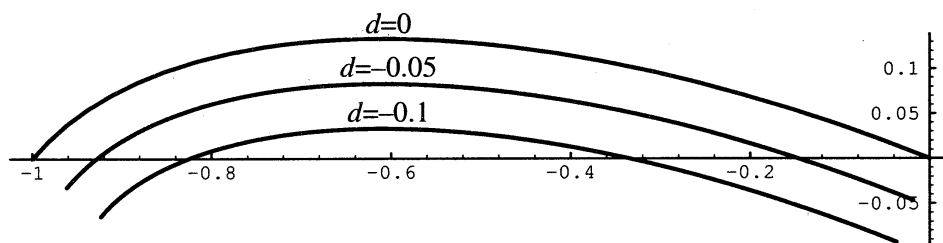
Fig. 10. Offset curves.
