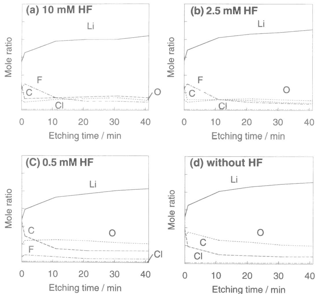
Figure 4-9 XPS depth profiles for the elements in the surface film formed on lithium deposited on the Ni substrate at 0.2 \text{ mA cm}^{-2} from PC containing 1.0 \text{ M LiClO}_4 and (a) 10 \text{ mM HF} , (b) 2.5 \text{ mM HF} , (c) 0.50 \text{ mM HF} , or (d) without HF.
