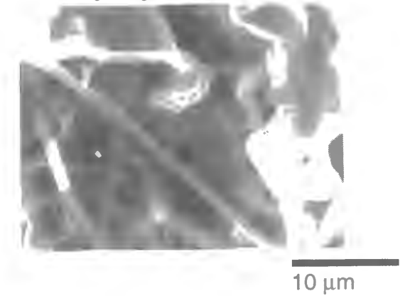
Figure 1-18 Scanning electron micrographs of lithium deposited on the as-received lithium foil electrode immersed for 72 h in in various electrolytes at 0.2 mA cm -2 (1.0 C cm -2 ), electrolyte ; PC containing 1.0 mol dm -3 (a) LiClO 4 , (b) LiCF 3 SO 3 , and (c) LiPF 6 .
