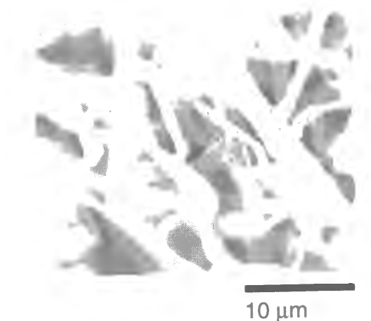
Figure 4 Scanning electron micrograph of typical dendritic lithium
