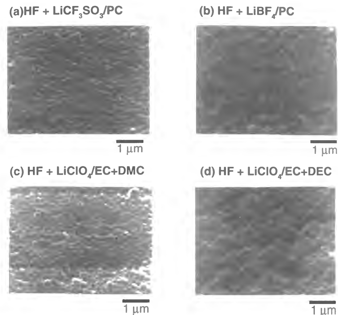
Figure 5-2 Scanning electron micrographs of lithium electrodeposited ( 1.0 \text{ mA cm}^{-2} ) on the Ni substrate in (a) 1.0 \text{ M LiCF}_3\text{SO}_3 / \text{PC} , (b) 1.0 \text{ M LiBF}_4 / \text{PC} , (c) 1.0 \text{ M LiClO}_4 / \text{EC+DMC} , or (d) 1.0 \text{ M LiClO}_4 / \text{EC+DEC} containing 10 \text{ mM HF} and 14 \text{ mM H}_2\text{O} .
