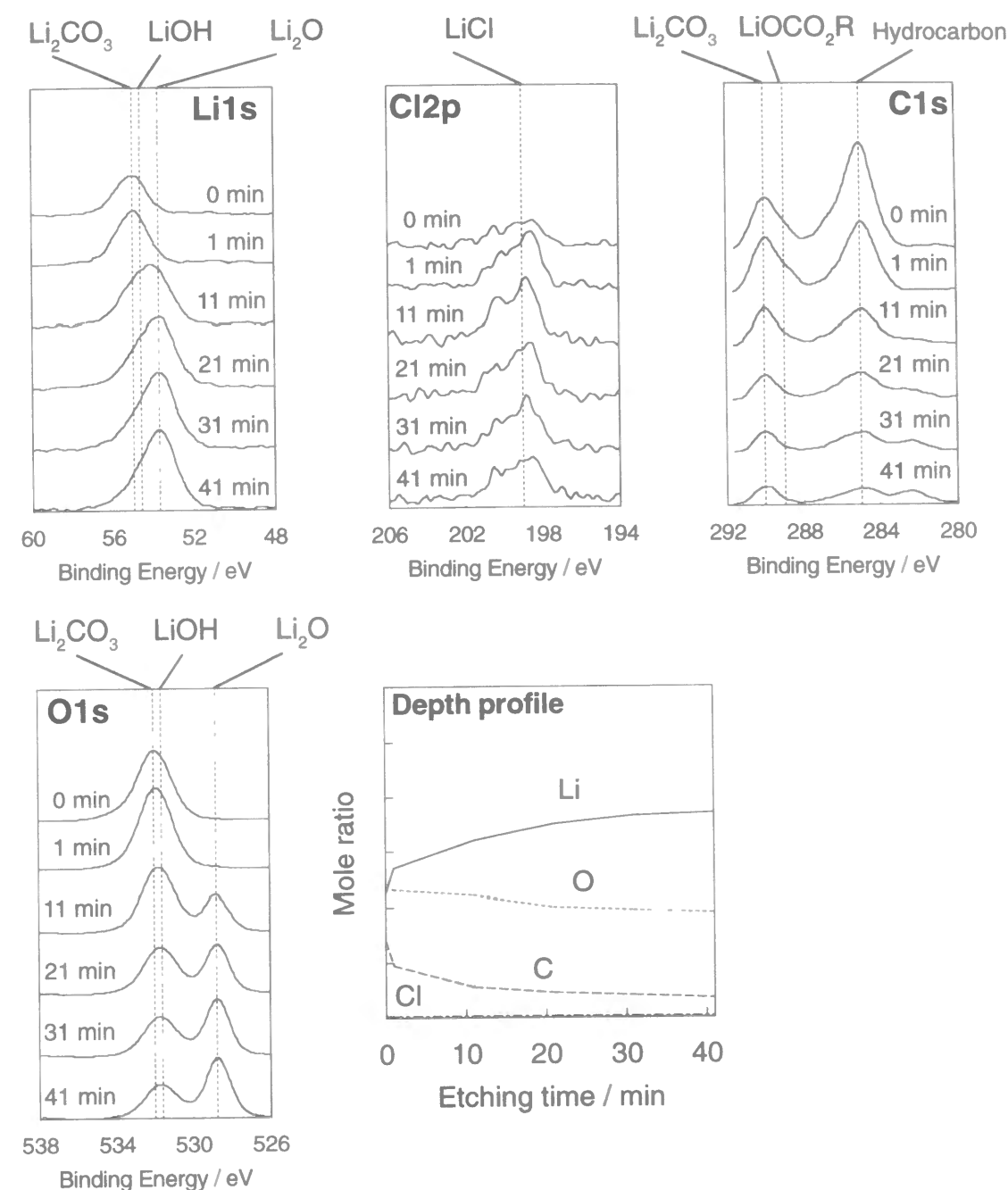
Figure 3-1 XPS spectra of \text{Li } 1s , \text{Cl } 2p , \text{C } 1s , and \text{O } 1s for lithium deposited on the Ni substrate in \text{LiClO}_4/\text{PC} at 1.0 \text{ mA cm}^{-2} ( 1.0 \text{ C cm}^{-2} ), and depth profile of each element in the surface film. The time in each figure indicates the duration of the Ar ion etching.
