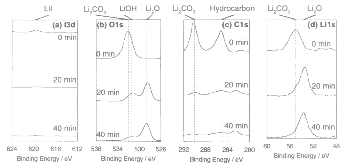
Figure 2-4 XPS spectra of (a) I 3d5/2 , (b) O 1s , (c) C 1s , and (d) Li 1s for the lithium foil after the immersion in the PC containing 0.2 mM HI for 72 h. Time indicate the duration of the argon ion etching.
