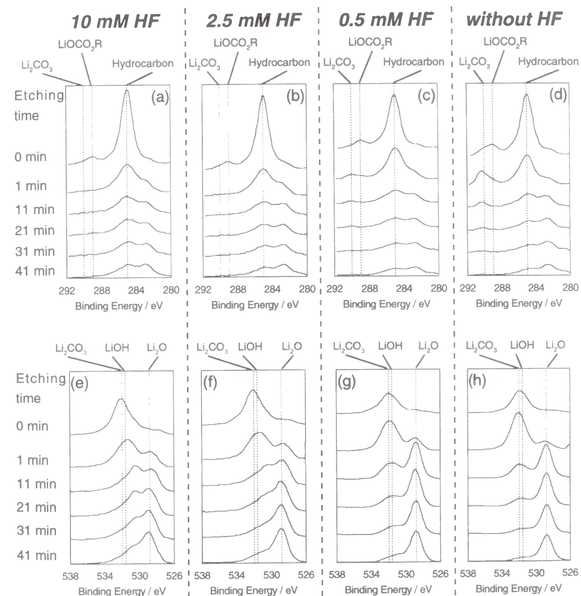
Figure 4-8 XPS spectra of C 1s and O 1s for lithium deposited on the Ni substrate at 0.2 \text{ mA cm}^{-2} from PC containing 1.0 \text{ M LiClO}_4 and (a, e) 10 \text{ mM HF} , (b, f) 2.5 \text{ mM HF} , (c, g) 0.50 \text{ mM HF} , or (d, h) without HF; time indicates the duration of the argon ion etching.
