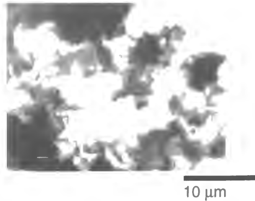
Figure 1-19 Scanning electron micrographs of lithium deposited on the as-received lithium foil electrode immersed for 10 min in various electrolytes at 0.2 mA cm -2 (1.0 C cm -2 ), electrolyte ; PC containing 1.0 M LiPF 6 .
