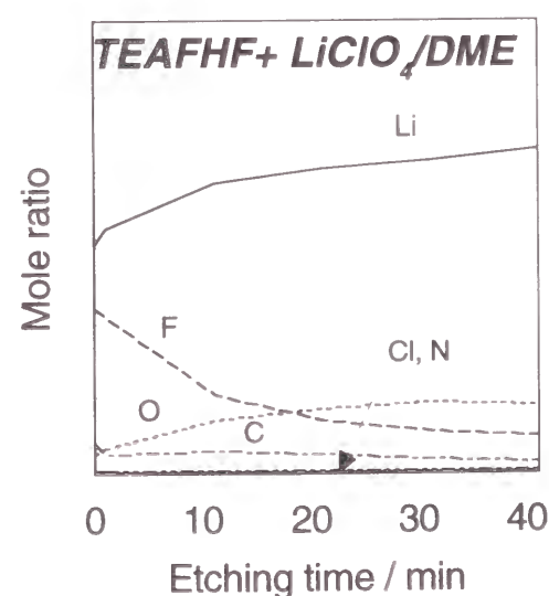
Figure 9-9 Depth profiles of the elements involved in the surface film on lithium deposited in dimethoxy ethane containing 0.4 \text{ M LiClO}_4 and 2.5 \text{ mM TEAFHF} .
