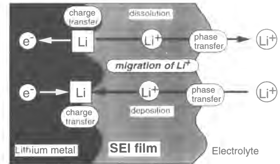
Figure 6 Schematic illustration of solid electrolyte interface (SEI) model [21] .
