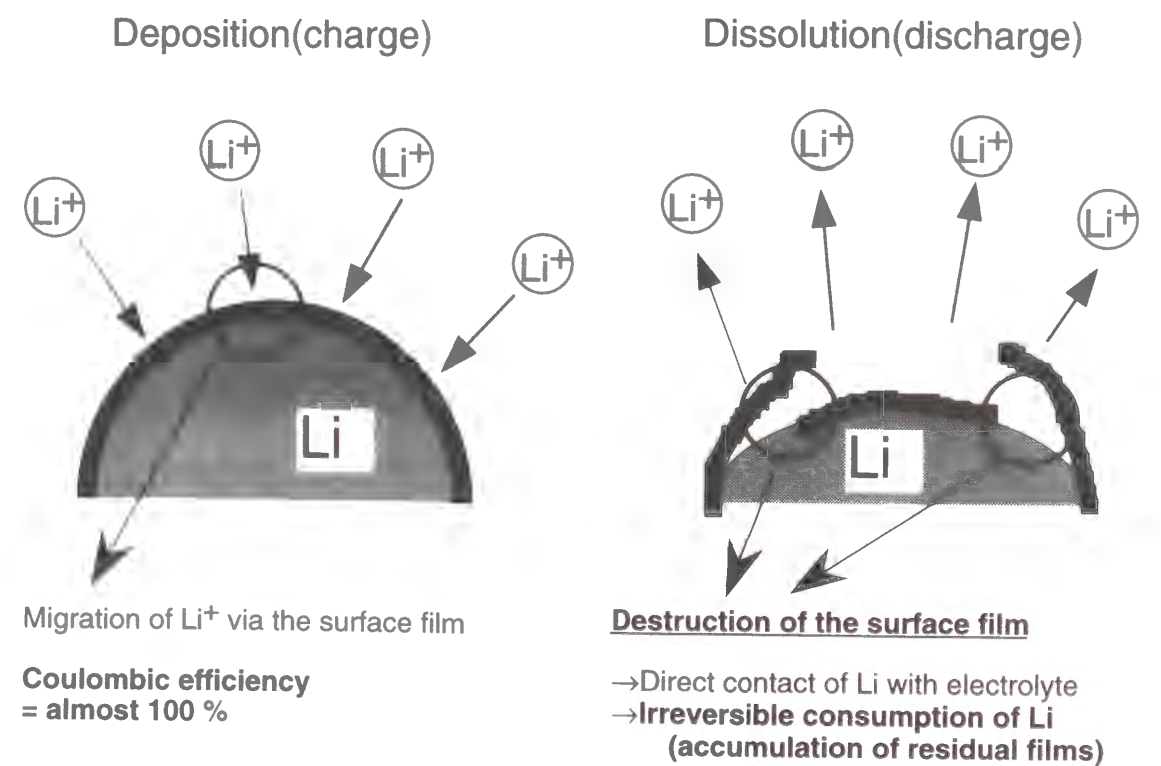
Figure 8-5 Schematic illustration of the deposition and dissolution process of lithium metal in the electrolyte containing HF.
