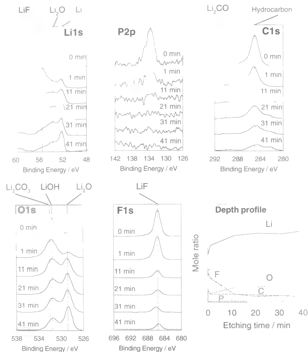
Figure 3-4 XPS spectra of Li 1s, P 2p, C 1s, O 1s, and F 1s for lithium deposited on the Ni substrate in \text{LiPF}_6/\text{PC} at 1.0 \text{ mA cm}^{-2} ( 1.0 \text{ C cm}^{-2} ), and depth profile of each element in the surface film. The time in each figure indicates the duration of the Ar ion etching.
