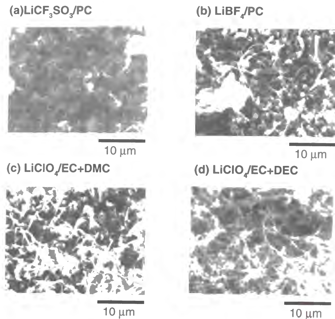
Figure 5-1 Scanning electron micrographs of lithium electrodeposited ( 1.0 \text{ mA cm}^{-2} ) on the Ni substrate in (a) 1.0 \text{ M LiCF}_3\text{SO}_3 / \text{PC} , (b) 1.0 \text{ M LiBF}_4 / \text{PC} , (c) 1.0 \text{ M LiClO}_4 / \text{EC+DMC} , or (d) 1.0 \text{ M LiClO}_4 / \text{EC+DEC} ,
