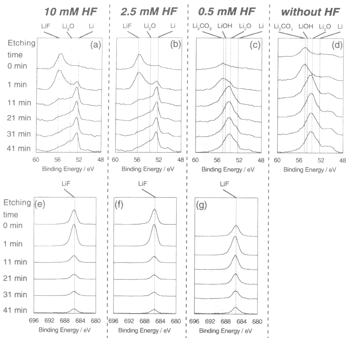
Figure 4-7 XPS spectra of Li 1s and F 1s for lithium deposited on the Ni substrate at 0.2 \text{ mA cm}^{-2} from PC containing 1.0 \text{ M LiClO}_4 and (a, e) 10 \text{ mM HF} , (b, f) 2.5 \text{ mM HF} , (c, g) 0.50 \text{ mM HF} , or (d) without HF; time indicates the duration of the argon ion etching.
