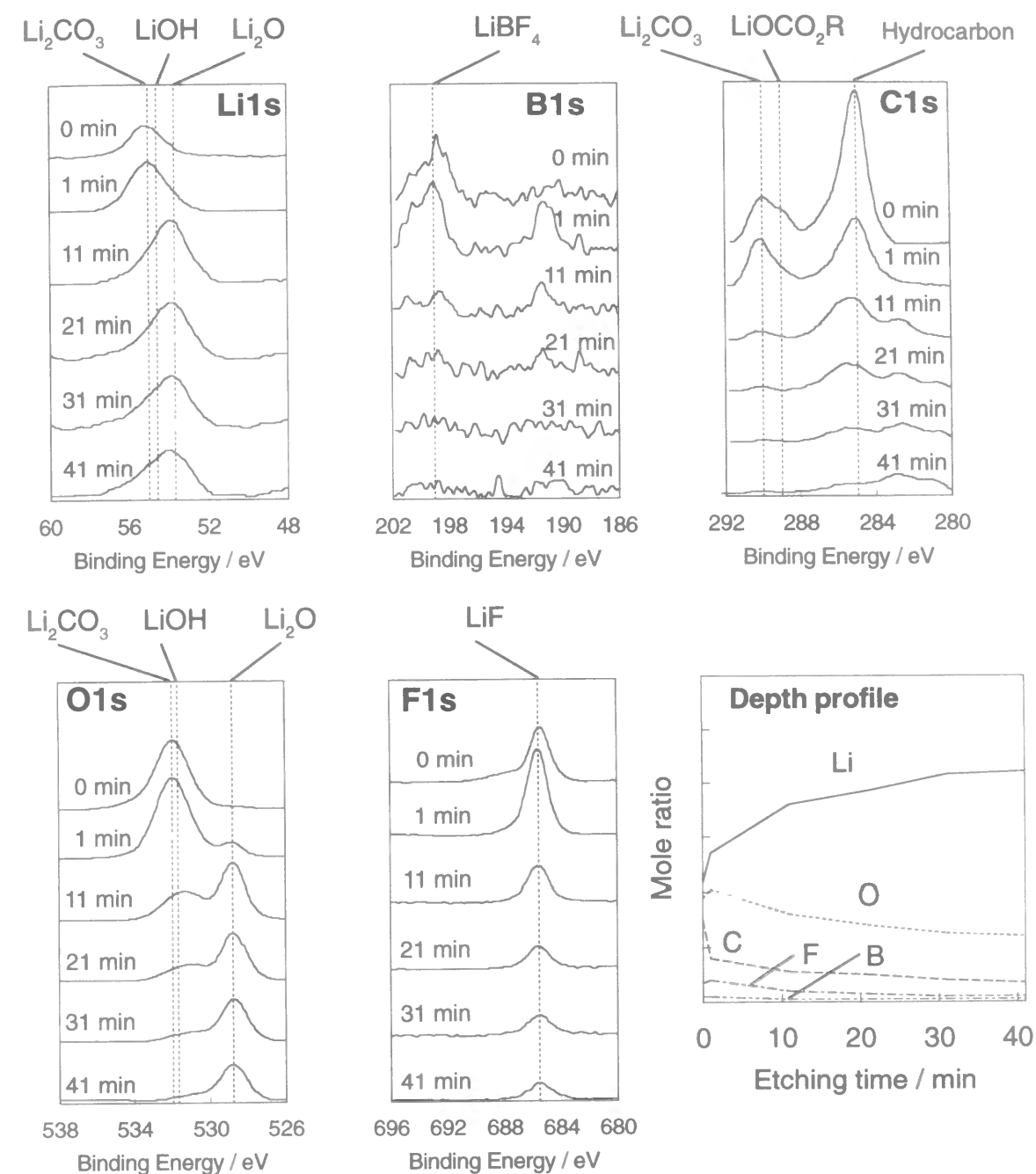
Figure 3-3 XPS spectra of Li 1s, B 1s, C 1s, O 1s, and F 1s for lithium deposited on the Ni substrate in LiBF 4 /PC at 1.0 mA cm -2 (1.0 C cm -2 ), and depth profile of each element in the surface film. The time in each figure indicates the duration of the Ar ion etching.
