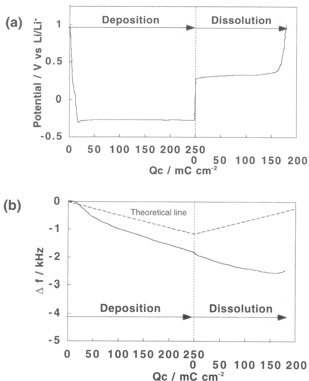
Figure 8-3 (a) Potential changes and (b) frequency changes of 6 MHz Ni quartz crystal microbalance electrode at the electrodeposition and dissolution (current density: 1.0 mA cm -2 ) of lithium in 1.0 M LiClO 4 /PC containing 10 mM HF and 14 mM H 2 O, dotted line is theoretical line if only lithium metal (mass:7) is deposited.
