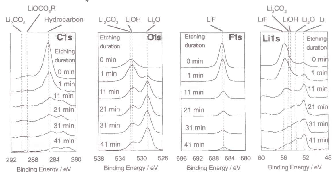
Figure 9-8 XPS spectra of Li 1s, C 1s, O 1s, and F 1s electrons for lithium deposited in dimethoxy ethane containing 0.4 \text{ M LiClO}_4 and 2.5 \text{ mM TEAFHF} . Times in figures indicate the argon ion etching duration. The current density; 1.0 \text{ mA cm}^{-2} , the total charge; 7.2 \text{ C cm}^{-2} .
