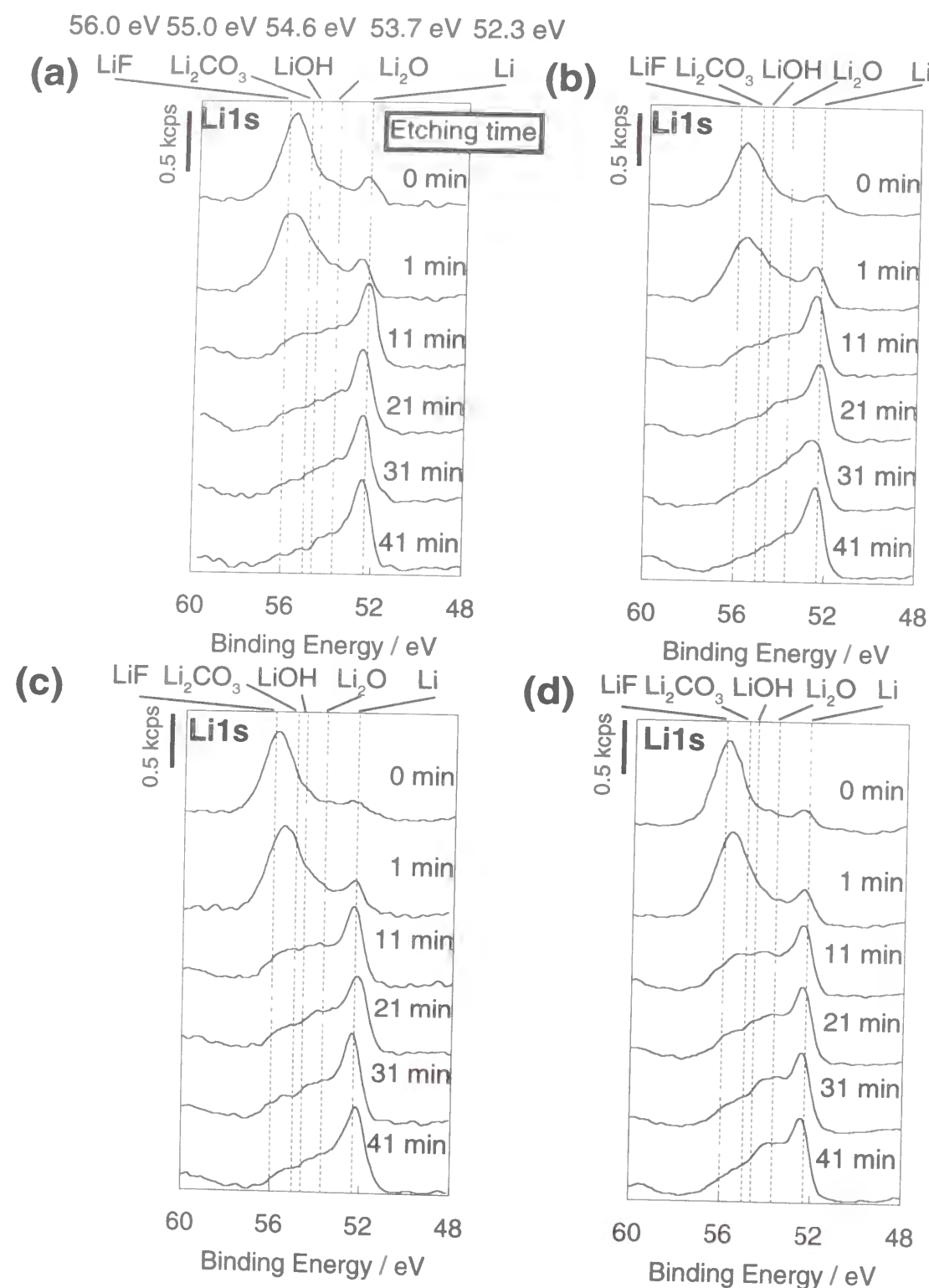
Figure 5-8 XPS spectra of Li1s for lithium deposited ( 1.0 \text{ mA cm}^{-2} , 1.0 \text{ C cm}^{-2} ) on the Ni substrate in (a) 1.0 \text{ M LiCF}_3\text{SO}_3/\text{PC} , (b) 1.0 \text{ M LiBF}_4/\text{PC} , (c) 1.0 \text{ M LiClO}_4/\text{EC} + \text{DMC} , and (d) 1.0 \text{ M LiClO}_4/\text{EC} + \text{DEC} containing 10 \text{ mM HF} + 14 \text{ mM H}_2\text{O} .
