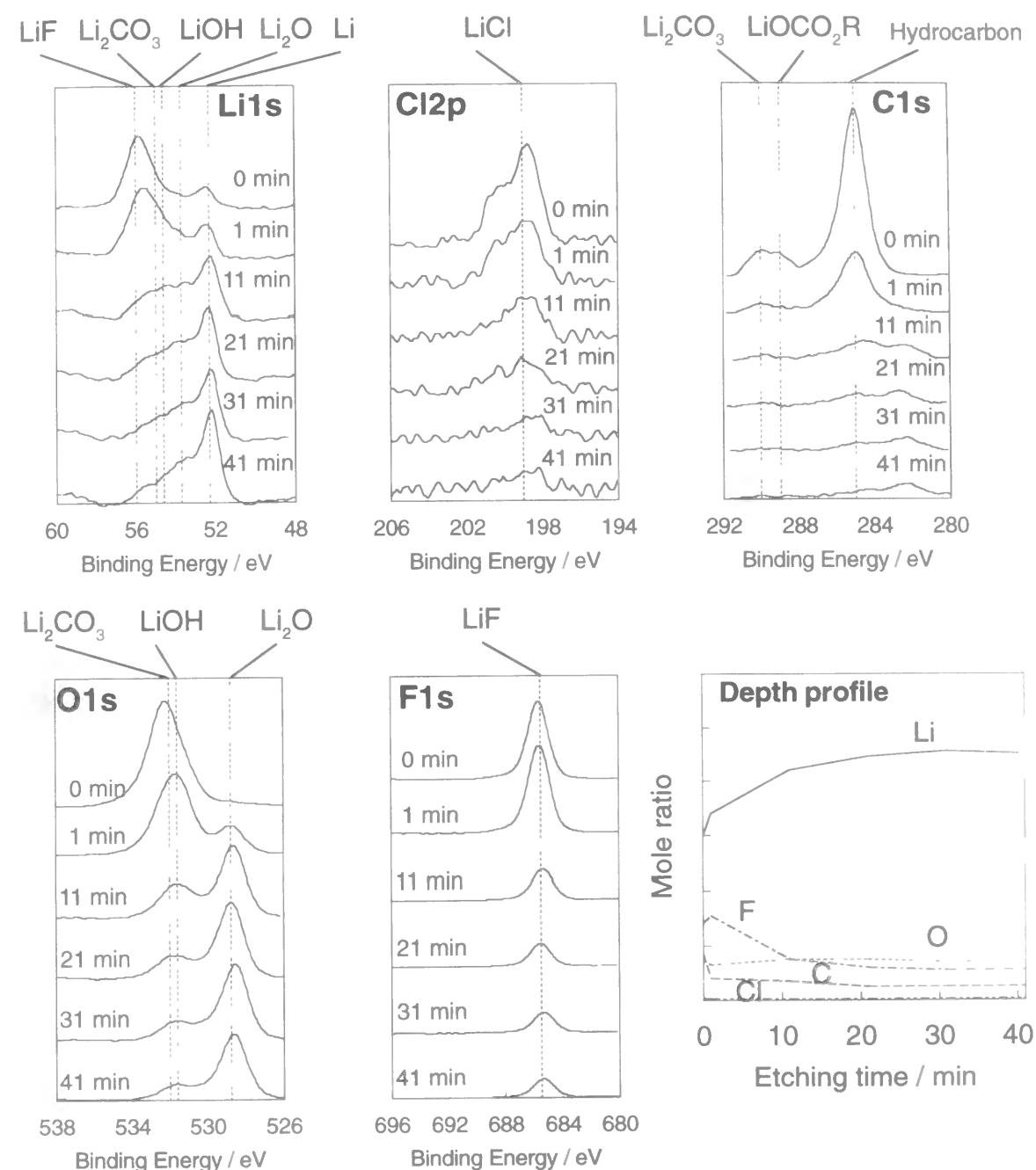
Figure 3-8 XPS spectra of \text{Li 1s} , \text{Cl 2p} , \text{C 1s} , \text{O 1s} , and \text{F 1s} for lithium deposited on the Ni substrate in propylene carbonate containing 1.0 \text{ M LiClO}_4 and 5.0 \text{ mM HF} at 1.0 \text{ mA cm}^{-2} ( 1.0 \text{ C cm}^{-2} ). The time in each figure indicates the duration of the Ar ion etching.
