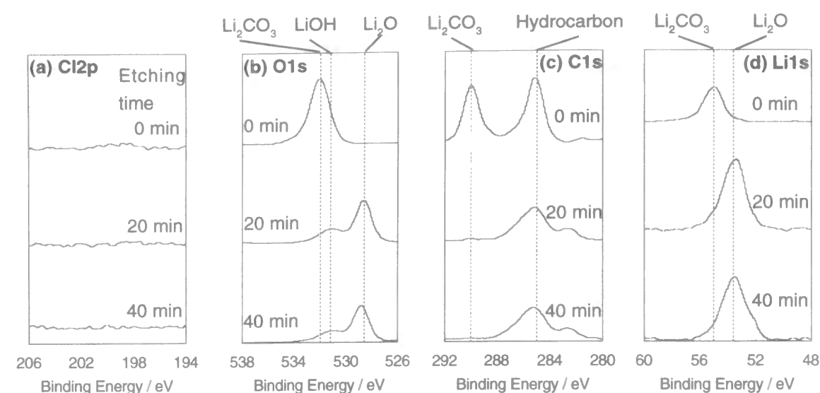
Figure 2-3 XPS spectra of (a) Cl 2p , (b) O 1s , (c) C 1s , and (d) Li 1s for the lithium foil after the immersion in the PC containing 0.2 mM HCl for 72 h. Time indicate the duration of the argon ion etching.
