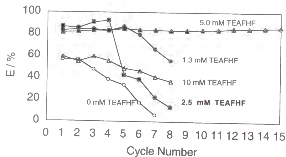
Figure 9-10 Utilization of lithium deposited in dimethoxy ethane containing 0.4 mM \text{LiClO}_4 and various contents of TEAFHF. The current density; 1.0 \text{ mA cm}^{-2} , the total charge; 2.0 \text{ mA h cm}^{-2} ( 7.2 \text{ C cm}^{-2} ), the cut off potential; 0.4 \text{ V vs. Li/Li}^+ .
