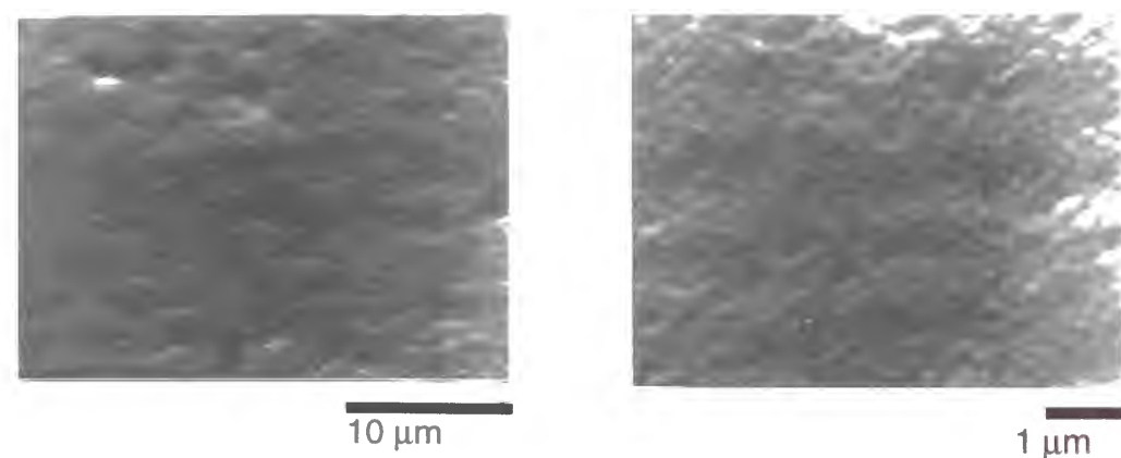
Figure 3-7 Scanning electron micrographs of lithium deposited on the Ni substrate in propylene carbonate containing 1.0 \text{ mol dm}^{-3} \text{ LiClO}_4 and 5 \times 10^{-3} \text{ mol dm}^{-3} \text{ HF} at 1.0 \text{ mA cm}^{-2} ( 1.0 \text{ C cm}^{-2} ).
