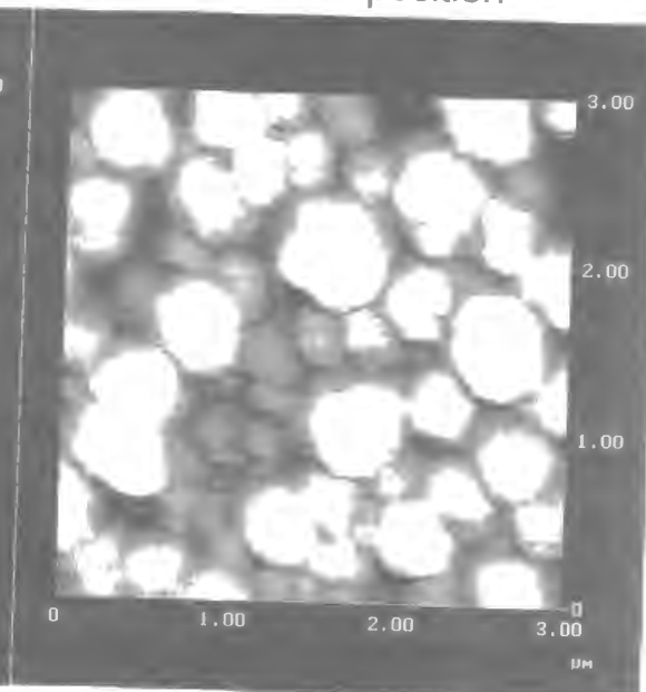
(b) 300 mC cm -2 deposition
