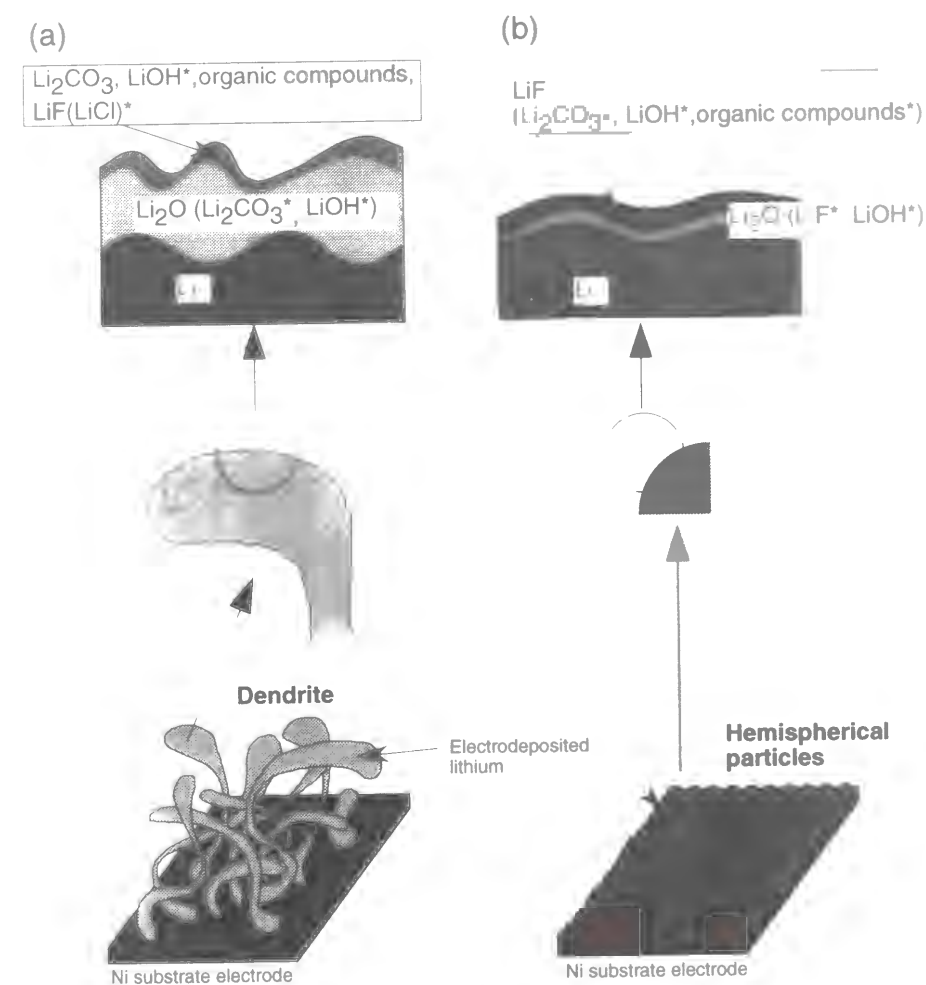
Figure 3-5 Schematic illustrations of the surface condition and the morphology of lithium deposited on the Ni substrate (a) in \text{LiAsF}_6 , \text{LiBF}_4 , and \text{LiClO}_4/\text{PC} and (b) in \text{LiPF}_6/\text{PC} . *: minor species
