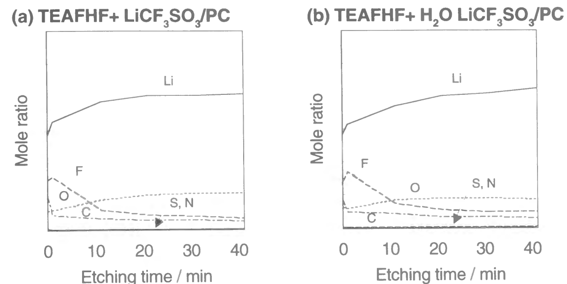
Figure 9-3 Depth profiles of the elements involved in the surface film on lithium deposited in (a) propylene carbonate containing 1.0 M \text{LiCF}_3\text{SO}_3 and 2.5 mM TEAFHF, and (b) propylene carbonate containing 1.0 M \text{LiCF}_3\text{SO}_3 , 2.5 mM TEAFHF, and 10 mM \text{H}_2\text{O} .
