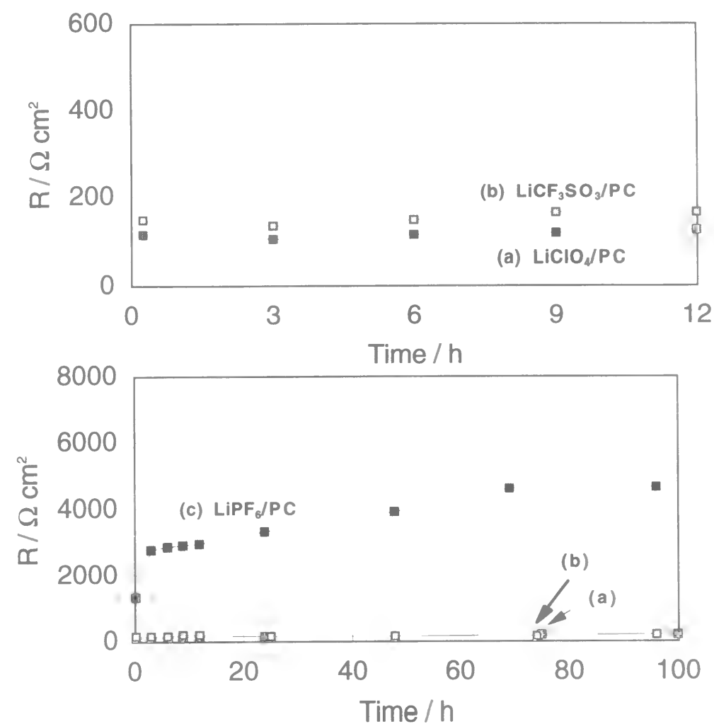
Figure 1-6 The resistance change of the surface film on the lithium electrode, obtained from the Cole- Cole plots in PC containing 1.0 M (a) LiClO 4 , (b) LiCF 3 SO 3 , and (c) LiPF 6 .
