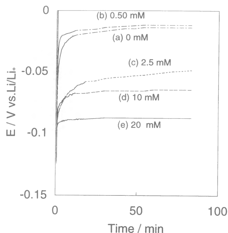
Figure 4-13 Charge curves on the Ni substrate from PC containing 1.0 M \text{LiClO}_4 (a) without HF, or (b) with 0.50 mM HF, (c) 2.5 mM HF, (d) 10 mM HF, or (e) 20 mM HF at 0.2 \text{ mA cm}^{-2} (charge ; 1.0 \text{ C cm}^{-2} ).
