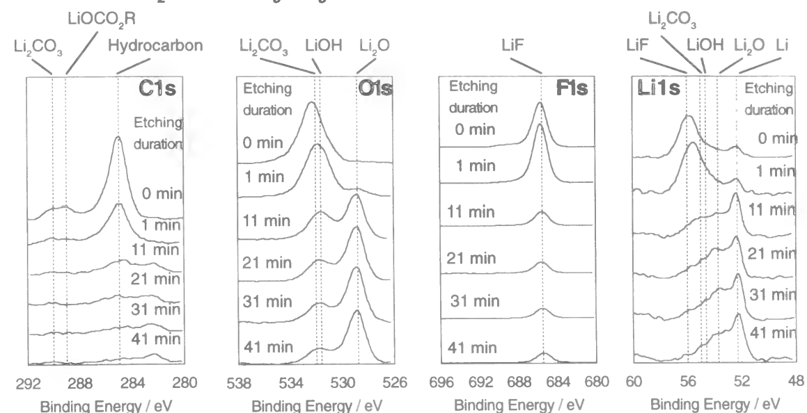
Figure 9-6 XPS spectra of Li 1s, C 1s, O 1s, and F 1s electrons for lithium deposited in propylene carbonate containing 1.0 M \text{LiCF}_3\text{SO}_3 , 2.5 \text{ mM} TEAFHF, and 10 \text{ mM} \text{H}_2\text{O} . Times in figures indicate the argon ion etching duration. The current density; 1.0 \text{ mA cm}^{-2} , the total charge; 1.0 \text{ C cm}^{-2} .
