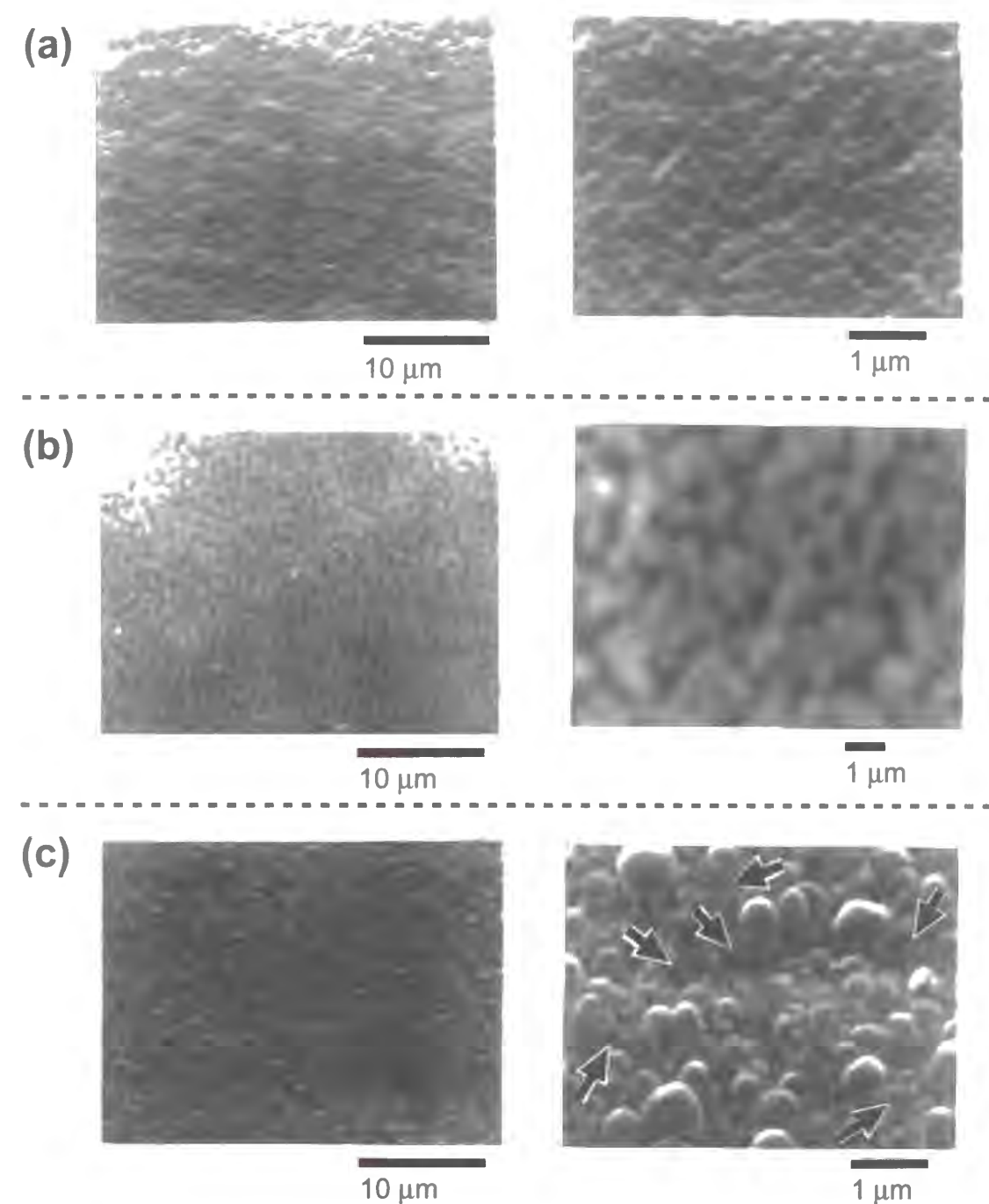
Figure 6-1 Scanning electron micrographs for the Ni substrate electrode in propylene carbonate containing 1.0 M LiCF 3 SO 3 , 10 mM HF, and 14 mM H 2 O after (a) the first deposition of lithium, (b) the first dissolution of lithium, and (c) the 2nd deposition of lithium.
