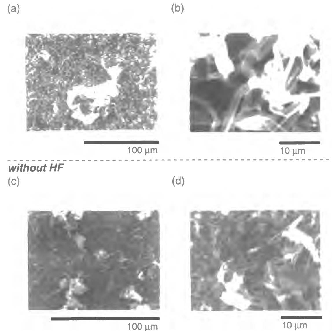
Figure 4-6 Scanning electron micrographs of lithium deposited on the Ni substrate at 0.2 \text{ mA cm}^{-2} from PC containing 1.0 \text{ M LiClO}_4 and various concentrations of HF [(a, b) 0.50 \text{ mM HF} ; (c, d) without HF].
