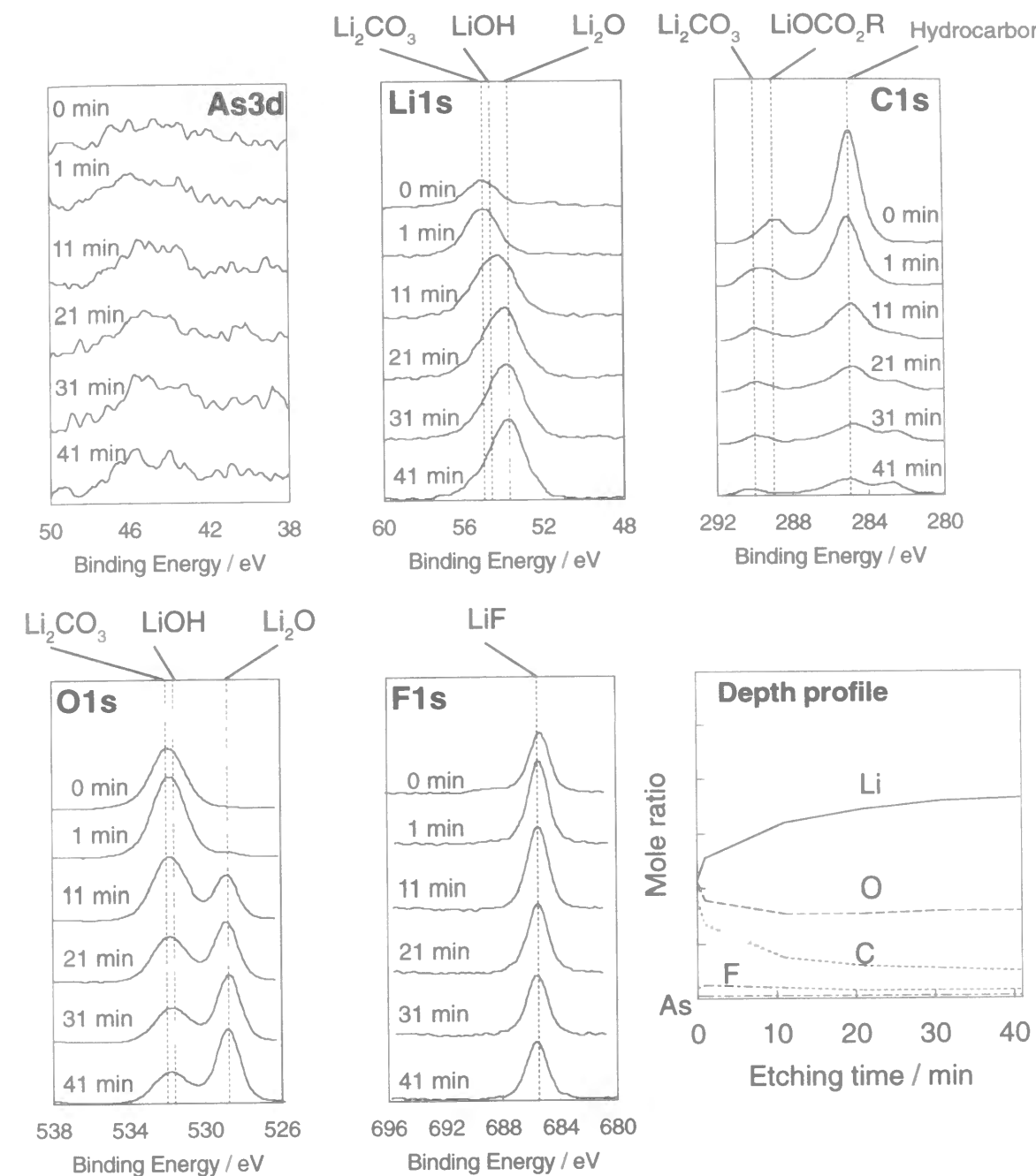
Figure 3-2 XPS spectra of As 3d, Li 1s, C 1s, O 1s, and F 1s for lithium deposited on the Ni substrate in \text{LiAsF}_6/\text{PC} at 1.0 \text{ mA cm}^{-2} ( 1.0 \text{ C cm}^{-2} ), and depth profile of each element in the surface film. The time in each figure indicates the duration of the Ar ion etching.
