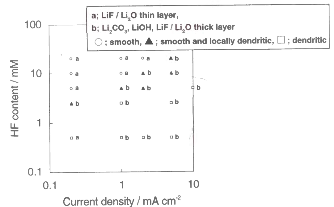
Figure 4-10 Dependence of condition of surface film and morphology of lithium on current density and HF content in 1.0 \text{ M LiClO}_4 / \text{PC} .
