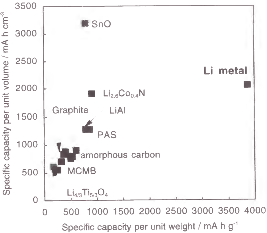
Figure 3 Energy density of various anode materials for rechargeable lithium battery.
