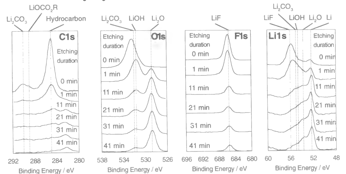
Figure 9-2 XPS spectra of Li 1s, C 1s, O 1s, and F 1s electrons for lithium deposited in propylene carbonate containing 1.0 M LiCF 3 SO 3 and 2.5 mM TEAFHF. Times in figures indicates the argon ion etching duration.
