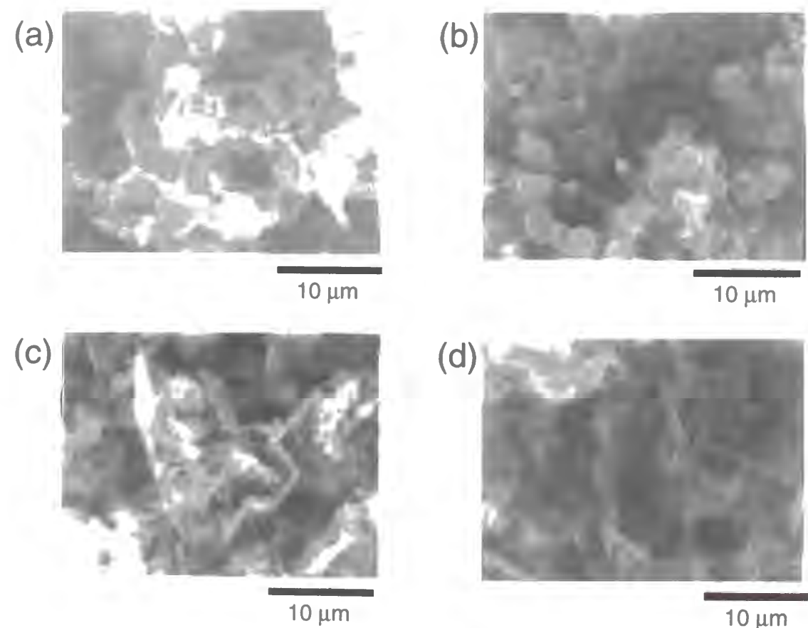
Figure 2-8 Scanning electron micrographs of lithium deposited on lithium foils after the immersion in the PC containing (a) 0.2 mM \text{H}_3\text{PO}_4 , (b) 0.2 mM \text{HF} , (c) 0.2 mM \text{HCl} , or (d) 0.2 mM \text{HI} for 72 h (the electrodeposition current : 0.20 \text{ mA cm}^{-2} , duration : 80 min, electrolyte : PC containing 1.0 M \text{LiPF}_6 ).
