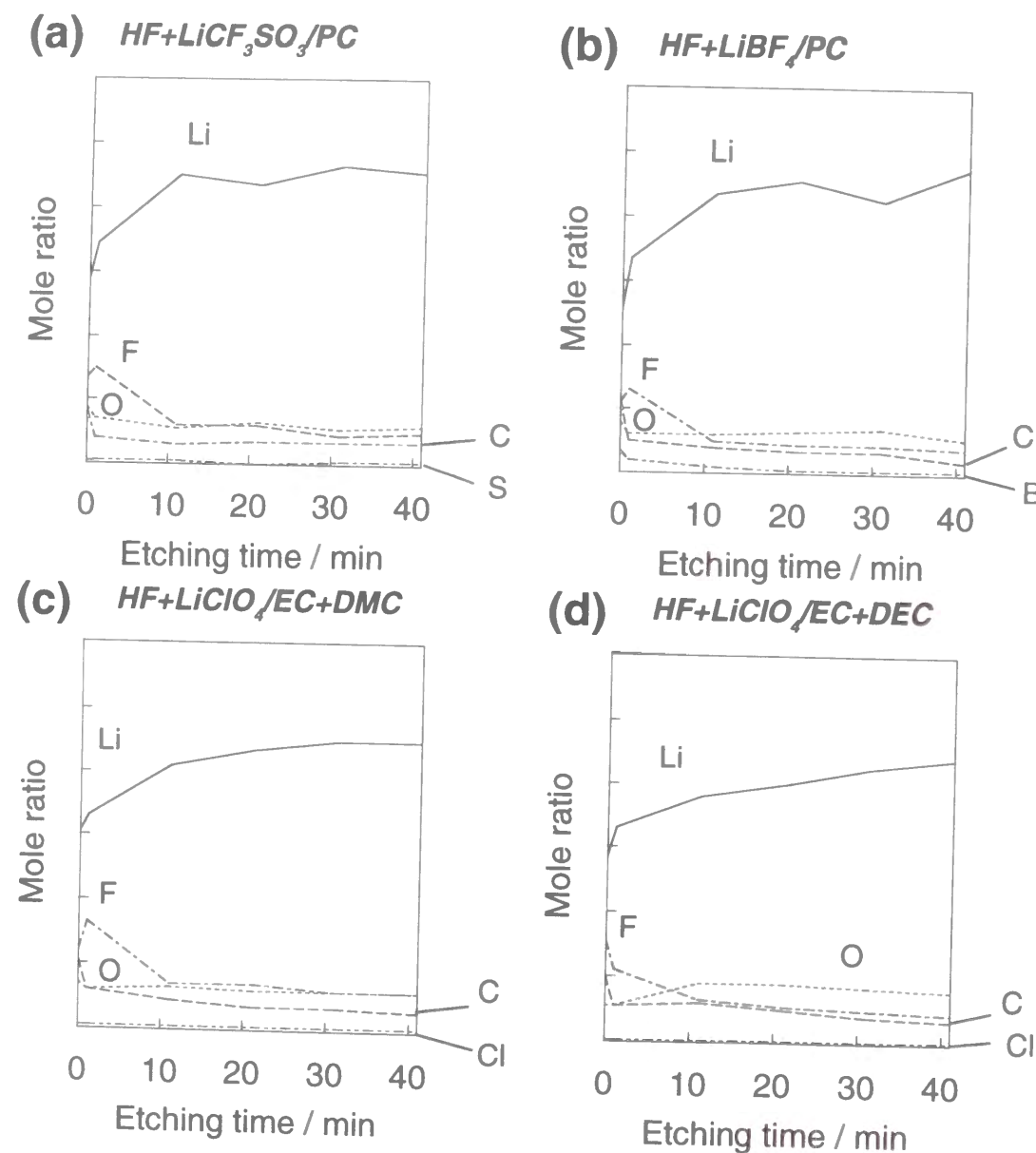
Figure 5-10 XPS depth profiles for each element in the surface film formed on lithium deposited ( 1.0 \text{ mA cm}^{-2} , 1.0 \text{ C cm}^{-2} ) on the Ni substrata in (a) 1.0 \text{ M LiCF}_3\text{SO}_3/\text{PC} , (b) 1.0 \text{ M LiBF}_4/\text{PC} , (c) 1.0 \text{ M LiClO}_4/\text{EC}+\text{DMC} , and (d) 1.0 \text{ M LiClO}_4/\text{EC}+\text{DEC} containing 10 \text{ mM HF} + 14 \text{ mM H}_2\text{O} .
