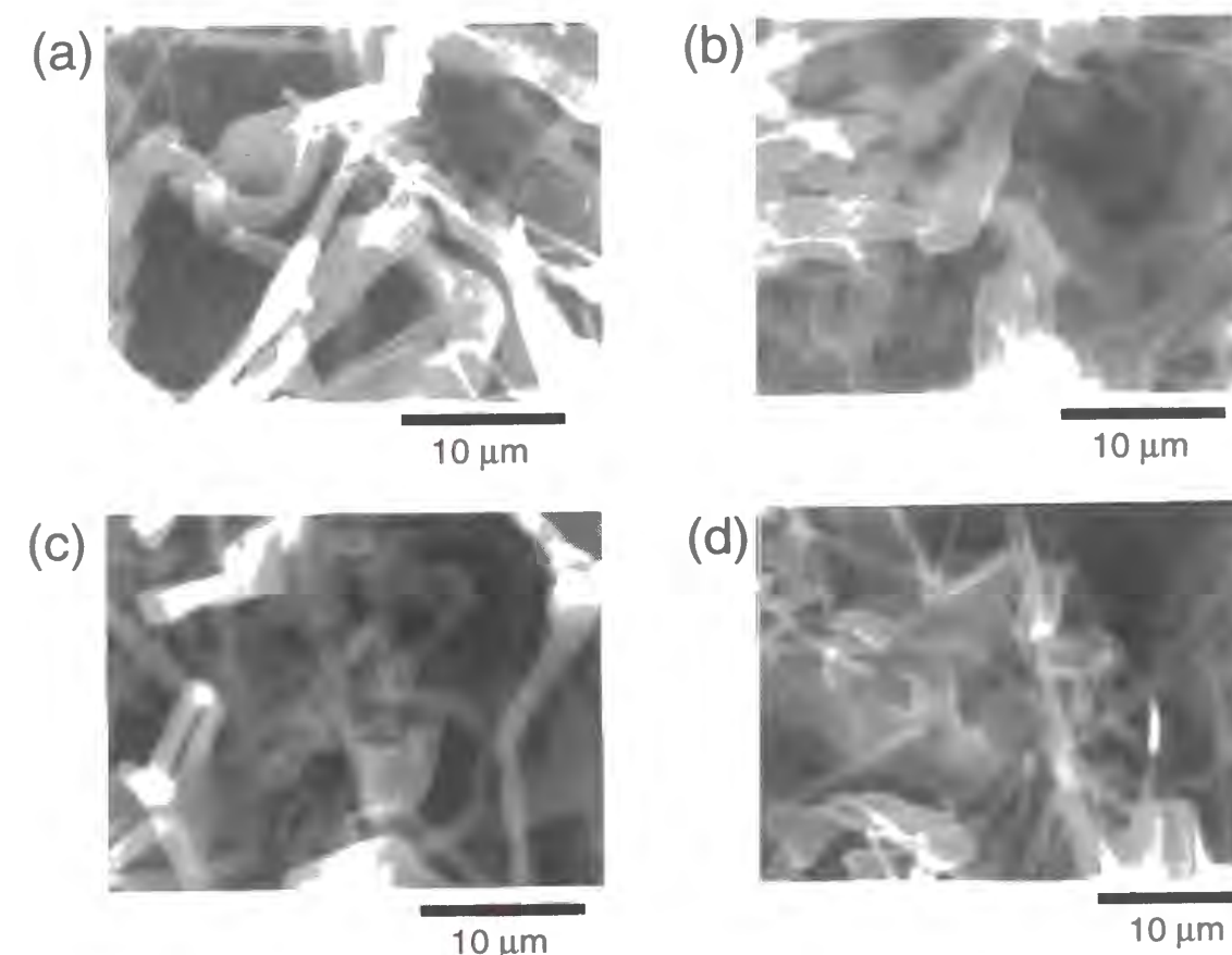
Figure 2-6 Scanning electron micrographs of lithium deposited on lithium foils after the immersion in the PC containing (a) 0.2 mM \text{H}_3\text{PO}_4 , (b) 0.2 mM HF, (c) 0.2 mM HCl, or (d) 0.2 mM HI for 72 h (the electrodeposition current : 0.20 \text{ mA cm}^{-2} , duration : 80 min, electrolyte : PC containing 1.0 \text{ M LiClO}_4 ).
