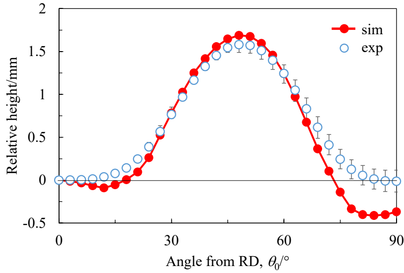
Fig. 10 Earing profile obtained from the experiment and simulation.
