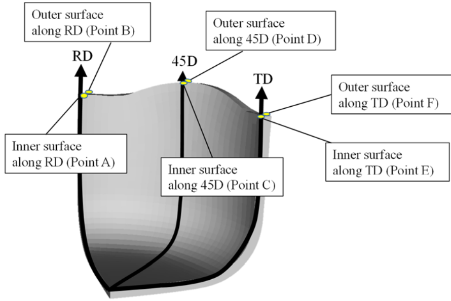
Fig. 4 Example of an EBSD measurement area.
