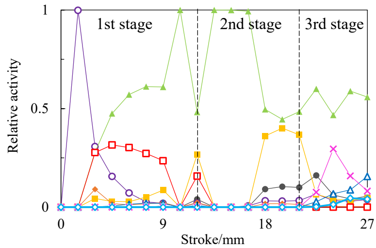
Fig. 22 Evolution of the relative activities obtained without considering friction at points (a) A, (b) B, (c) E, and (b) F shown in Fig. 3.
