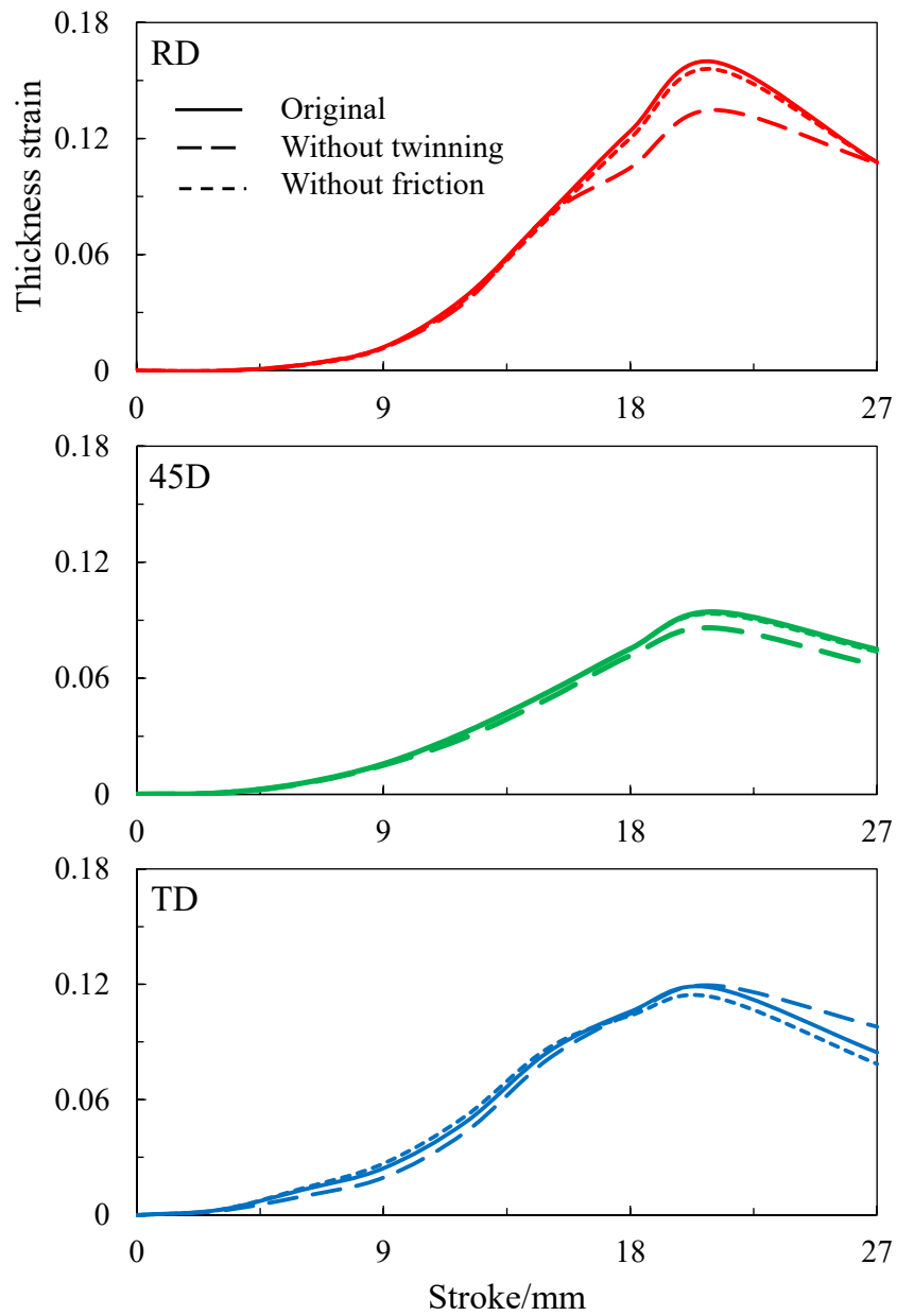
Fig. 21 Evolution of the thickness strain at the flange edge in the RD, 45D, and TD.
