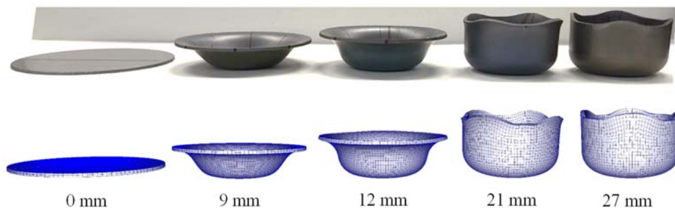
Fig. 8 Deformed shapes at the strokes of 0, 9, 12, 21, and 27 mm. The upper photographs are experimental results, and the lower figures are simulation results. For visibility purposes, the simulation results of the quarter part were mirror-copied to the other three quadrants to show the full geometries.
