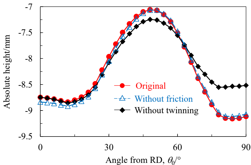
Fig. 19 Simulation result of the earing profile without twinning and without friction.
