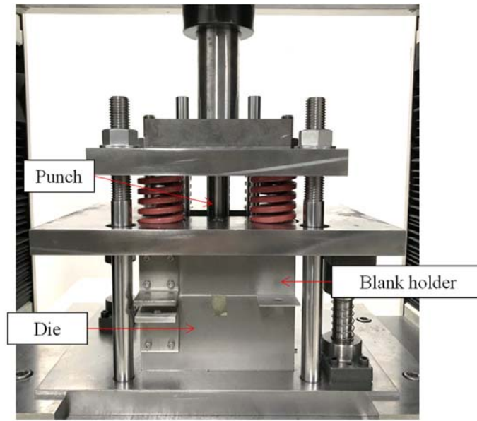
Fig. 1 Experimental setup for the cylindrical cup drawing.
