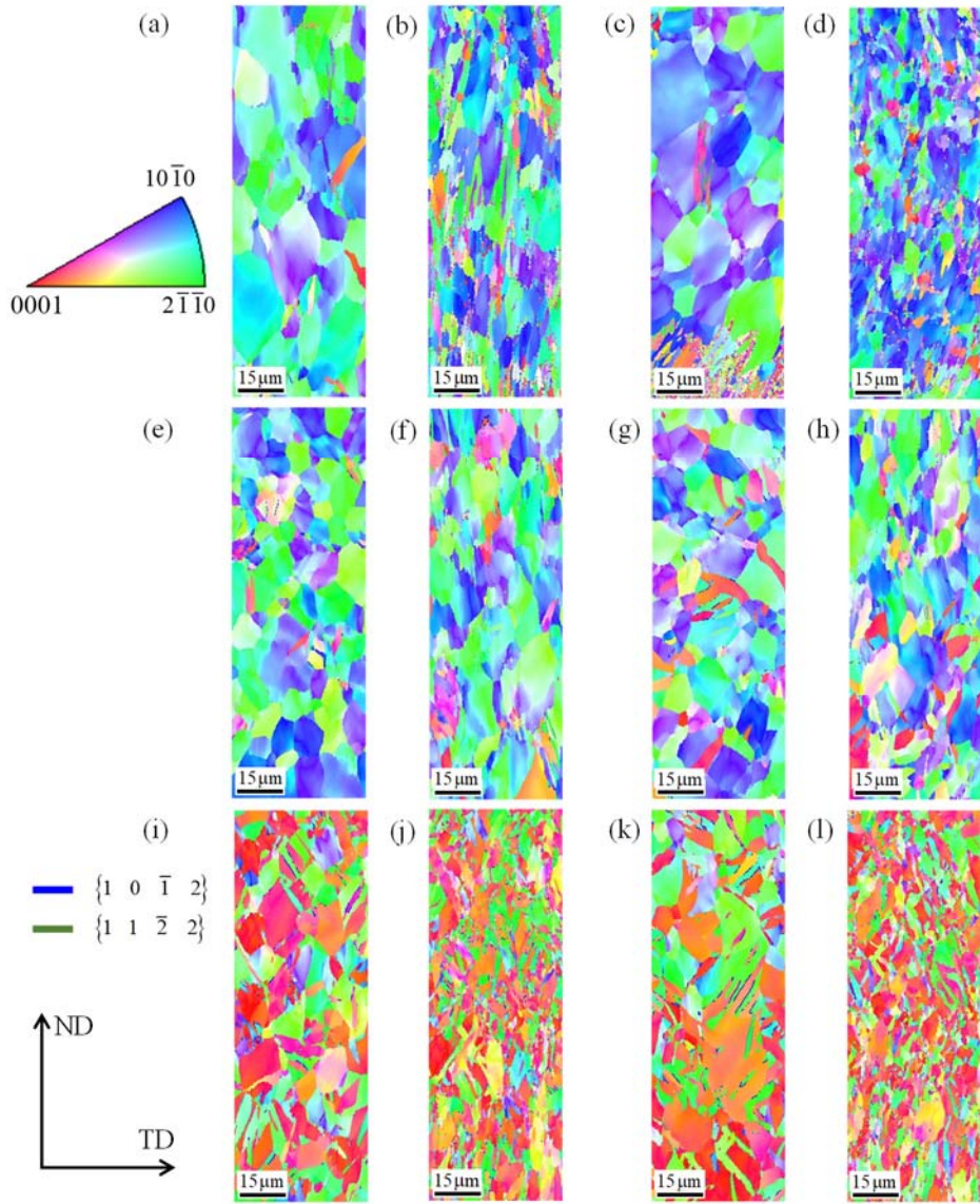
Fig. 17 IPF maps obtained from the experiment. Point A at the strokes of (a) 15 and (b) 27 mm; point B at the strokes of (c) 15 and (d) 27 mm; point C at the strokes of (e) 15 and (f) 27 mm; point D at the strokes of (g) 15 and (h) 27 mm; point E at the strokes of (i) 15 and (j) 27 mm; and point F at the strokes of (k) 15 and (l) 27 mm.
