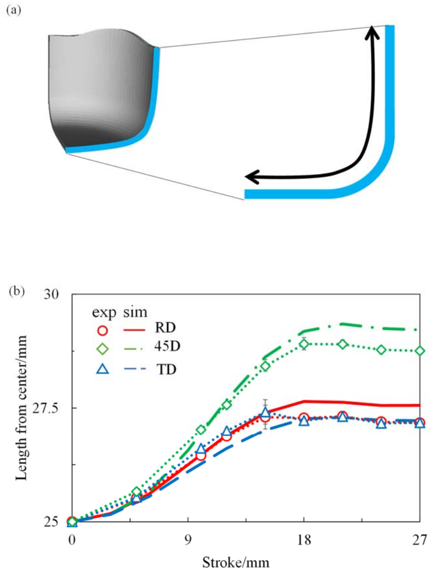
Fig. 11. Earing evolution obtained from the experiment and simulation. (a) Definition of length from the center of the cup and (b) evolution of length.
