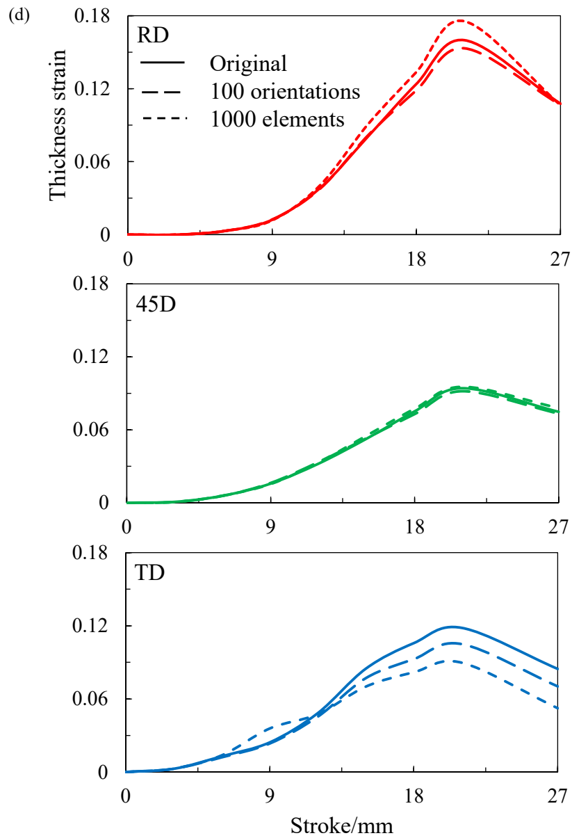
Fig. A1 Simulation results obtained using different numbers of orientations or finite elements. (a) The initial pole figures for 100 orientations, (b) the finite-element model with 1000 elements, (c) earing profile, and (d) evolution of the thickness strain at the flange edge.
