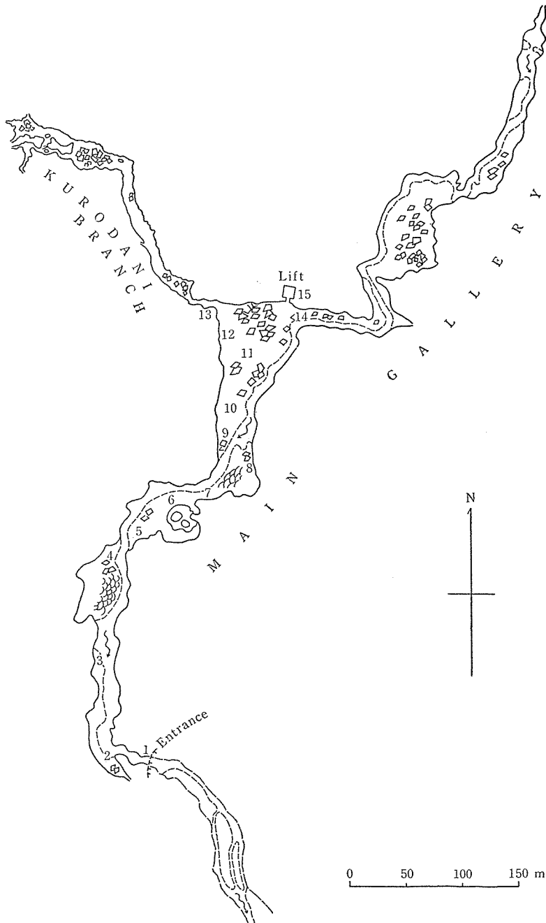
Fig. 1. Sketch map of Akiyoshi-dô Cave (adopted from ETO, partly modified by YAMAUTI, 1957); the numbers 1-15 indicate the stations investigated ( cf. pp. 318-319).
