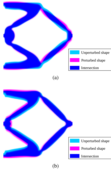
Fig. 17 Overlay image highlighting differences between unperturbed and perturbed shapes for optimized configurations obtained by l_C = 0.5L and L .
