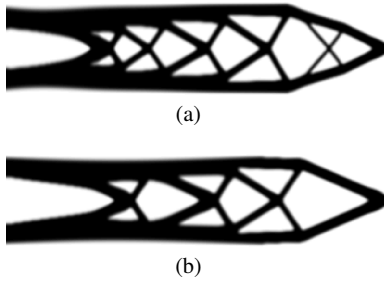
Fig. 11 Perturbed shapes at MPTPs when setting \beta_T = 5 for optimized configurations obtained with (a) l_C = 0.5L ; and (b) l_C = L .
