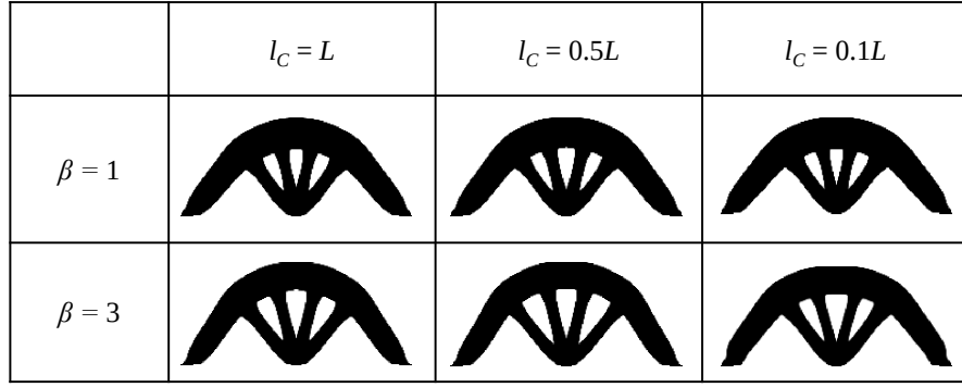
Fig. 5 Obtained optimized configurations.
