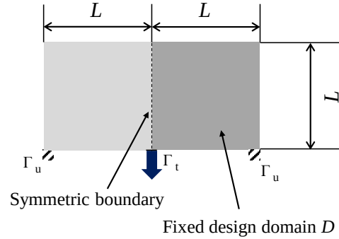
Fig. 4 Fixed design domain and boundary conditions for bridge design problem.
