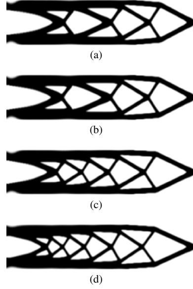
Fig. 8 Perturbed shapes at MPTP when setting \beta_T = 5 for optimized configurations obtained with (a) \beta_T = 0 ; (b) \beta_T = 1 ; (c) \beta_T = 3 ; and (d) \beta_T = 5 .
