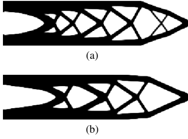
Fig. 9 Obtained optimized configurations for (a) l_C = 0.5L ; and (b) l_C = L .
