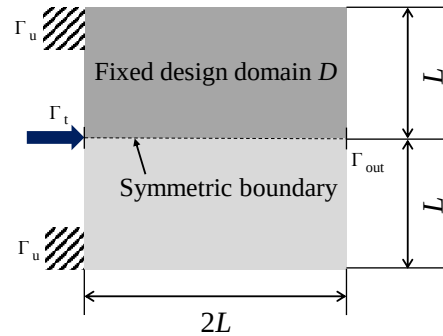
Fig. 12 Fixed design domain and boundary conditions for compliant mechanism optimum design problem.
