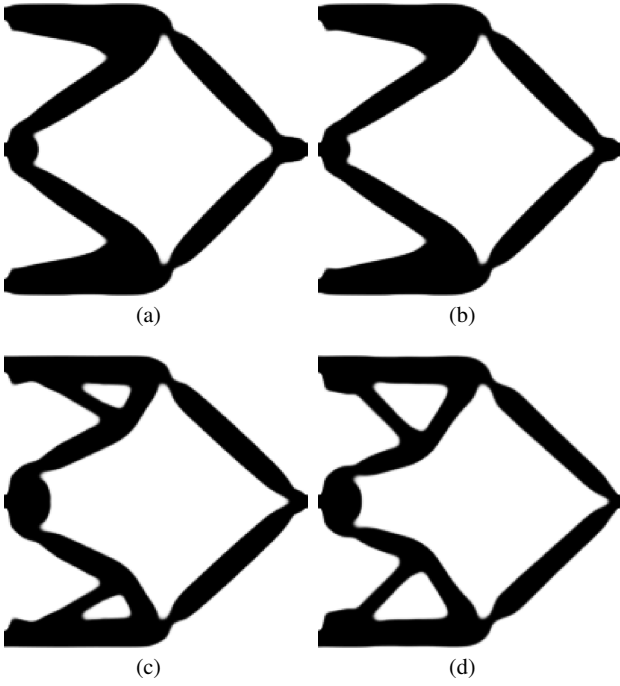
Fig. 13 Obtained optimized configurations for (a) \beta_T = 0 (deterministic solution); (b) \beta_T = 1 ; (c) \beta_T = 3 and (d) \beta_T = 5 .
