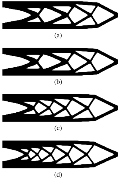
Fig. 7 Obtained optimized configurations for (a) \beta_T = 0 (deterministic solution); (b) \beta_T = 1 ; (c) \beta_T = 3 ; and (d) \beta_T = 5 .
