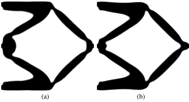
Fig. 15 Obtained optimized configurations for (a) l_C = 0.5L ; and (b) l_C = L .
