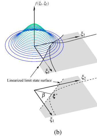
Fig. 3 Standard Gaussian probability density function: (a) limit state function; (b) linearized limit state function.
