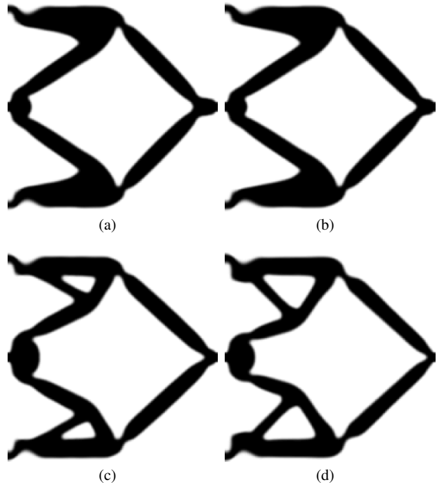
Fig. 14 Perturbed shapes at MPTPs when setting \beta_T = 5 for optimized configurations obtained when (a) \beta_T = 0 (deterministic solution); (b) \beta_T = 1 ; (c) \beta_T = 3 and (d) \beta_T = 5 .
