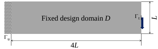
Fig. 6 Fixed design domain and boundary conditions for cantilever design problem.
