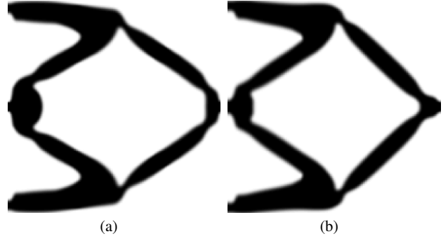
Fig. 16 Perturbed shapes at MPTPs when setting \beta_T = 5 for optimized configurations obtained with (a) l_C = 0.5L ; and (b) l_C = L .
