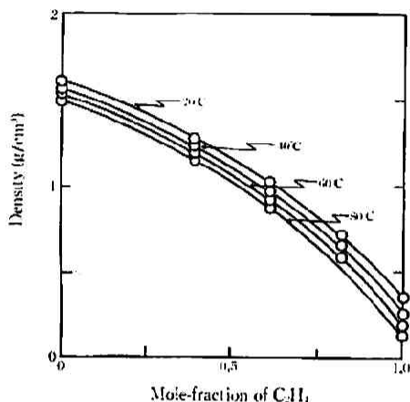
Fig. 5 Densities of C_2H_4-CCl_4 solutions at 100 kg/cm 2
