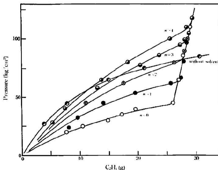
Fig. 3 Relations between amounts of C_2H_4 and pressure for mixtures of C_2H_4 and 60 ml of Cl(CH_2CH_2)CCl_3 , in constant volume 123 ml, at 30^\circ C
