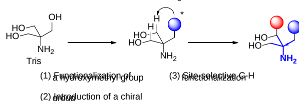
Scheme 1. Strategy for the Construction of the Quaternary Carbon Stereocenter of an \alpha -Tertiary Amine
