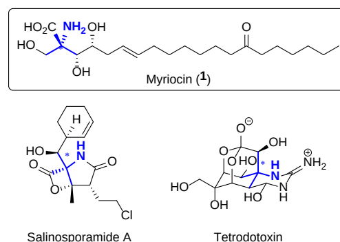
Figure 1. Structures of Myriocin and Natural Products with Chiral \alpha -Tertiary Amines
