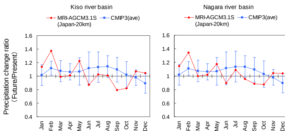
Fig. 9 Change of precipitation between present and future climate condition.
