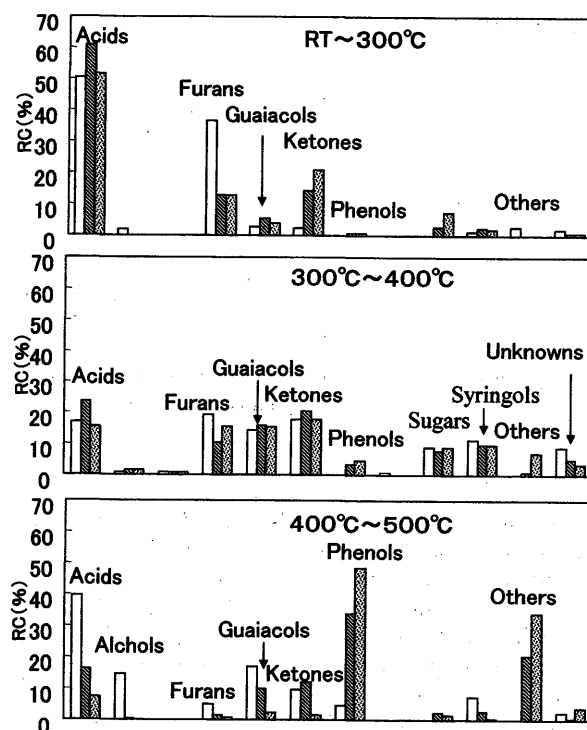
Fig. 2. Relative concentration of chemical components of pyrolyzed liquid of plywood and particleboard bonded with phenol-resin adhesive. Legend: □; solid wood, ▨; plywood, ▩; particleboard.
