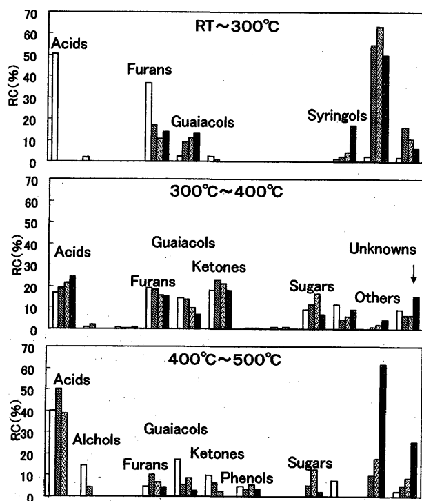
Fig. 1. Relative concentration of chemical components of pyrolyzed liquid of plywood, particleboard and MDF bonded with urea-resin adhesive. Legend: □; solid wood, ▨; plywood, ▩; particleboard, ■; MDF.
