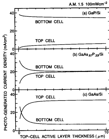
Fig. 7. Photo-generated current densities vs. top-cell active layer thickness ( w_p^t ) of \text{GaAs}_{1-x}\text{P}_x/\text{Si} cell assuming no recombination loss, (a) x=1 (GaP), (b) x=0.33 ( \text{GaAs}_{0.67}\text{P}_{0.33} ), and (c) x=0 (GaAs).
