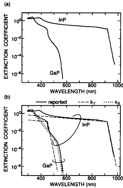
Fig. 6. Wavelength-dependence of extinction coefficients k(\lambda) of InP and GaP. (a) Reported values of InP and GaP. (b) Calculated values of k_r(\lambda) and k_x(\lambda) with measured values, based on our assumption.
