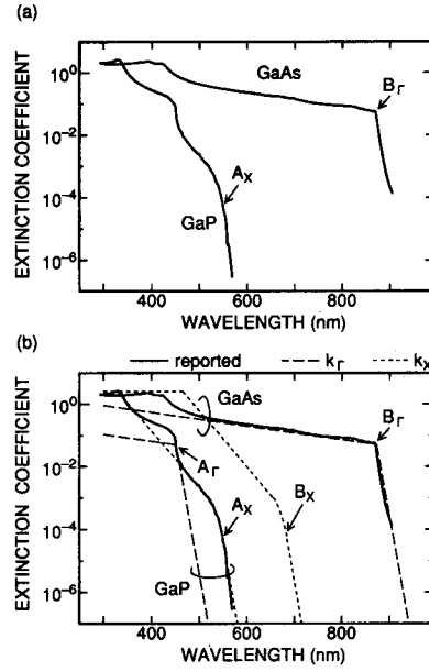
Fig. 4. Wavelength-dependence of extinction coefficients k(\lambda) of GaAs and GaP. (a) Reported values of GaAs and GaP. (b) Calculated values of k_r(\lambda) and k_x(\lambda) together with reported values, based on our assumption. Two solid lines represent reported values. Dashed and dotted lines represent k_r(\lambda) and k_x(\lambda) , respectively. The point A_r shows the \Gamma -valley bandgap of GaP, and the point A_x the X-valley one. The point B_r and B_x are for GaAs. The wavelengths of the points A_r , A_x , B_x , and B_r are 451, 549, 685, and 873 nm, respectively.
