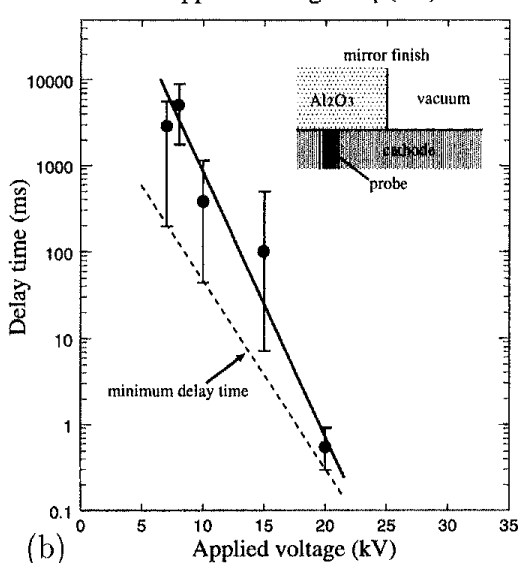
Figure 6. Delay characteristics for insulators with comparatively smooth surfaces (normal contact), (a) PMMA ( r_a=0.22 \mu\text{m} ), (b) \text{Al}_2\text{O}_3 ( r_a=0.16 \mu\text{m} ).
