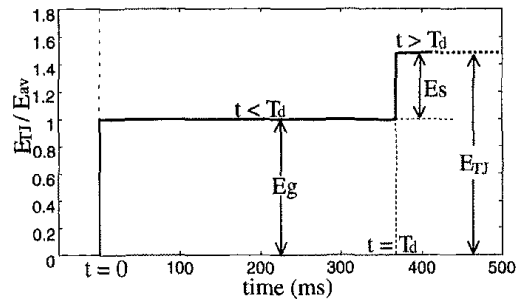
Figure 10. Calculated probe signal (PMMA).
