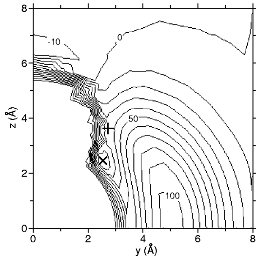
FIG. 13. Potential-energy surface calculated for the system Cs*He 2 -He. The Cs* atom was fixed at (y, z) = (0, 0) and the two He atoms of Cs*He 2 were fixed at (0, \pm 3.5) , in units of Å. The energy is in units of cm -1 and the zero of energy is at the dissociation limit Cs*He 2 ( A^2\Pi_{1/2} ) + He. The contour interval is 10 cm -1 . The marks “+” and “x” show the positions of saddle point and potential minimum, respectively.
