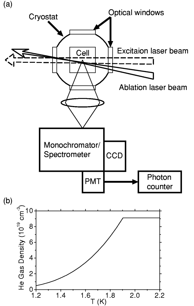
FIG. 5. (a) Experimental setup. (b) He gas density in the cell as a function of T .
