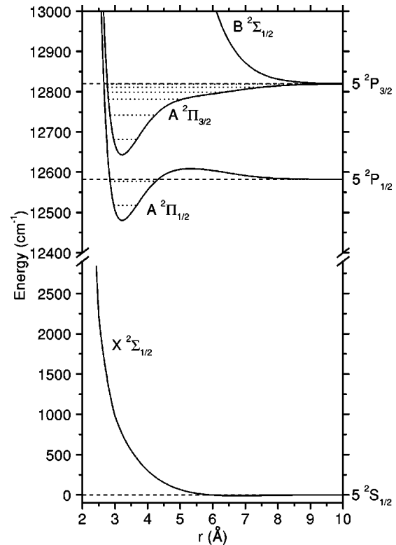
FIG. 1. Theoretical Rb-He potential curves of the ground state ( X^2\Sigma_{1/2} ) and the excited states ( A^2\Pi_{1/2} , A^2\Pi_{3/2} , and B^2\Sigma_{1/2} ) obtained from ab initio calculations. Dotted lines show the vibrational energy levels (see also Table I). Asymptotic energies of the potentials are shown by dashed lines, which are labeled on the right-hand side by atomic states of Rb.
