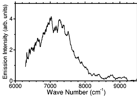
FIG. 6. Emission spectrum of \text{Rb}^*\text{He}_{n_{\max}} in liquid He.
