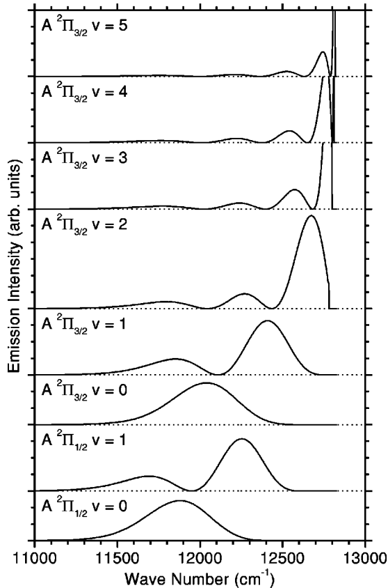
FIG. 2. Theoretical emission spectra from the vibrational levels of Rb*He.
