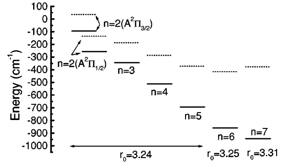
FIG. 3. Potential energy E'_n at the bottom of the potential well (solid lines) and the energy level E_n of the vibrational ground state (dotted lines) in the first electronic excited state for each n . The equilibrium radius r_0 in units of Å is also shown.
