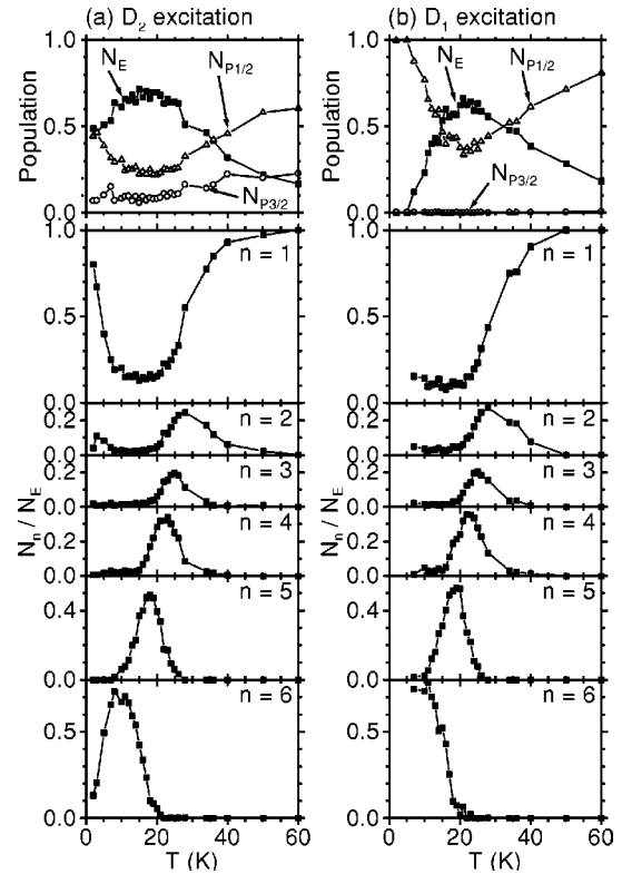
FIG. 10. Populations as functions of T in the cases of the D_2 excitation (a) and D_1 excitation (b). The N_n ( n=1-6 ) is the relative population of Rb*He n , and N_{P3/2} and N_{P1/2} are those of Rb( 5^2P_{3/2} ) and Rb( 5^2P_{1/2} ), respectively. The N_n has been normalized by the total population N_E (= \sum_{n=1}^6 N_n) of Rb*He n .
