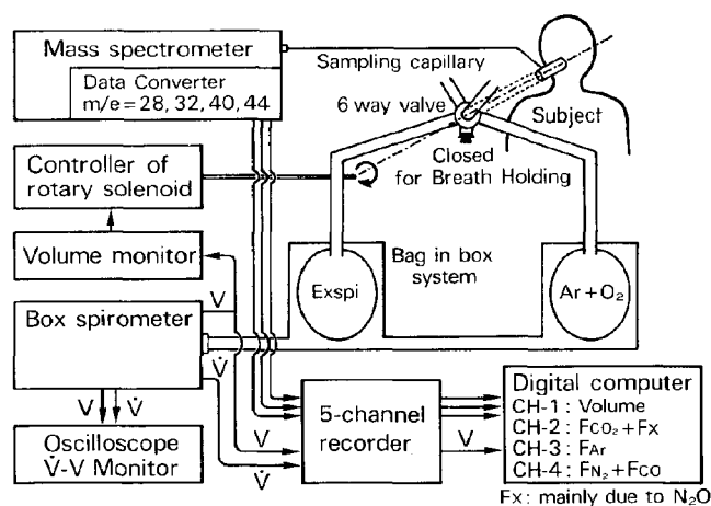
Fig. 1 Diagram of experimental arrangement
