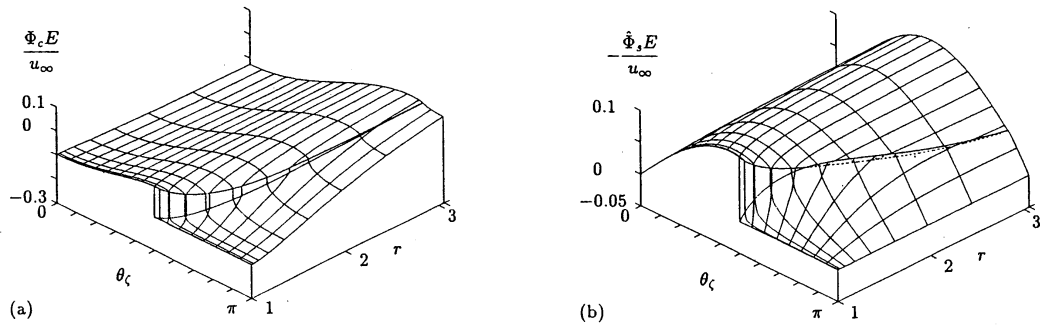
FIG. 15. The velocity distribution functions \Phi_c E and \hat{\Phi}_s E at \zeta = 0.556 for k_\infty = 1 . (a) \Phi_c E and (b) \hat{\Phi}_s E . (See the caption of Fig. 14.)
