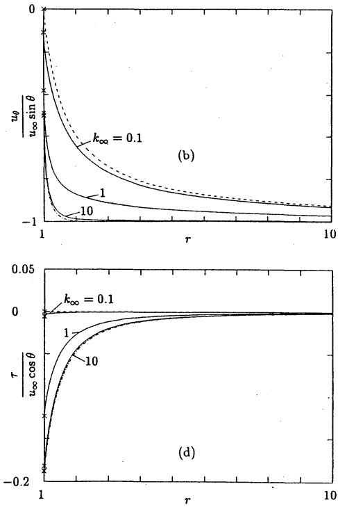
FIG. 3. The profiles of the macroscopic variables (hard sphere). (a) u_r/u_\infty \cos \theta vs r , (b) u_\theta/u_\infty \sin \theta vs r , (c) \omega/u_\infty \cos \theta vs r , and (d) \tau/u_\infty \cos \theta vs r . Here, — indicates the present numerical result, - - - the asymptotic solution (26a)-(26d) with k_\infty = 0 , and - - - the free molecular flow ( k_\infty = \infty ). The \times indicates the value at r = 1 .
