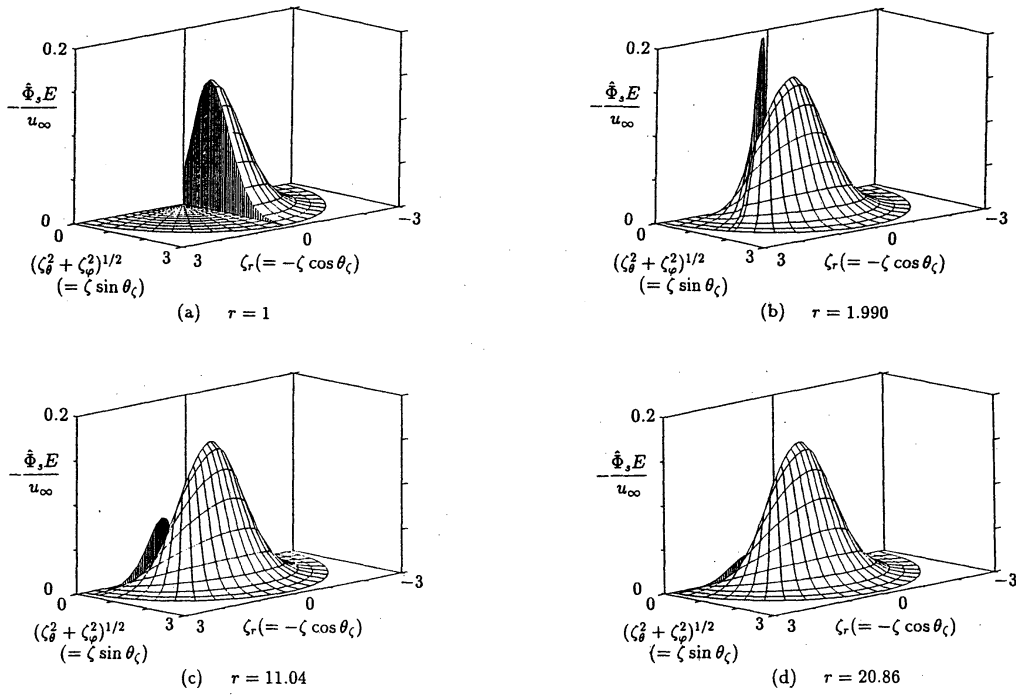
FIG. 11. The velocity distribution function \Phi_s E at four points in the gas for k_\infty = 10 . (a) r = 1 , (b) r = 1.990 , (c) r = 11.04 , and (d) r = 20.86 . (See the caption of Fig. 7.)
