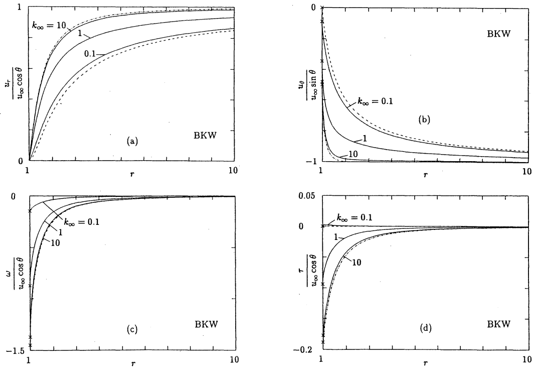
FIG. 4. The profiles of the macroscopic variables (BKW). (a) u_r/u_\infty \cos \theta vs r , (b) u_\theta/u_\infty \sin \theta vs r , (c) \omega/u_\infty \cos \theta vs r , and (d) \tau/u_\infty \cos \theta vs r . Here, — indicates the present numerical result, ---- the asymptotic solution (26a)-(26d) with k_\infty = 0 , and ..... the free molecular flow ( k_\infty = \infty ). The \times indicates the value at r = 1 . The conversion (58) of k_\infty is not made here.
