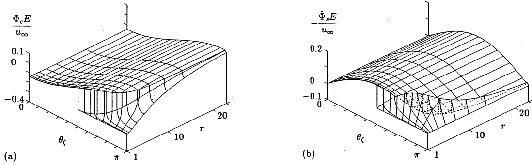
FIG. 16. The velocity distribution functions \Phi_c E and \hat{\Phi}_s E at \zeta = 0.556 for k_\infty = 10 . (a) \Phi_c E and (b) \hat{\Phi}_s E . (See the caption of Fig. 14.)
