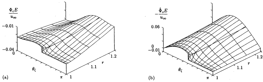
FIG. 14. The velocity distribution functions \Phi_c E and \hat{\Phi}_s E at \zeta = 0.556 for k_\infty = 0.1 . (a) \Phi_c E and (b) \hat{\Phi}_s E . The surfaces of \Phi_c E and \hat{\Phi}_s E are shown as functions of r and \theta_\zeta by lines r = \text{const} and \theta_\zeta = \text{const} . The vertical lines show the discontinuity. The invisible lines behind other parts are shown by dashed lines.
