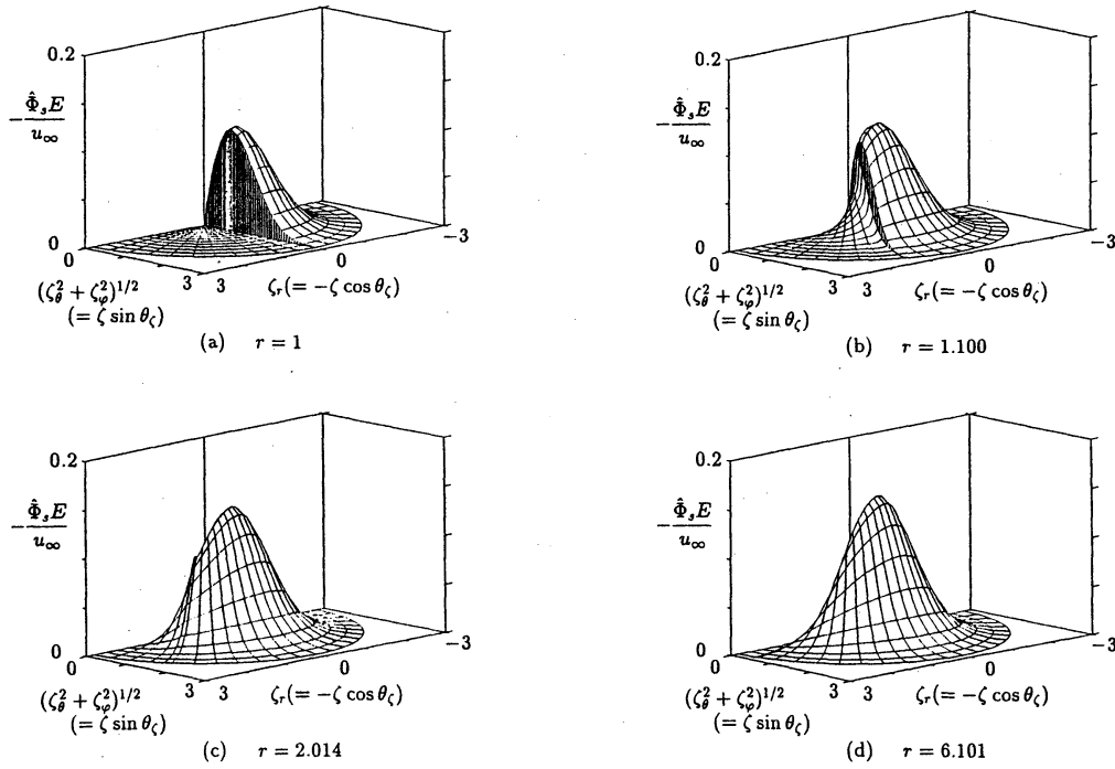
FIG. 9. The velocity distribution function \hat{\Phi}_s E at four points in the gas for k_\infty = 1 . (a) r = 1 , (b) r = 1.100 , (c) r = 2.014 , and (d) r = 6.101 . (See the caption of Fig. 7.)
