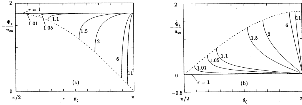
FIG. 13. The velocity distribution functions \Phi_c and \hat{\Phi}_s for \pi - \text{Arcsin}(1/r) < \theta_\zeta \le \pi (the molecules coming directly from the sphere) in the free molecular flow [Eqs. (23) and (24)]. (a) \Phi_c and (b) \hat{\Phi}_s .
