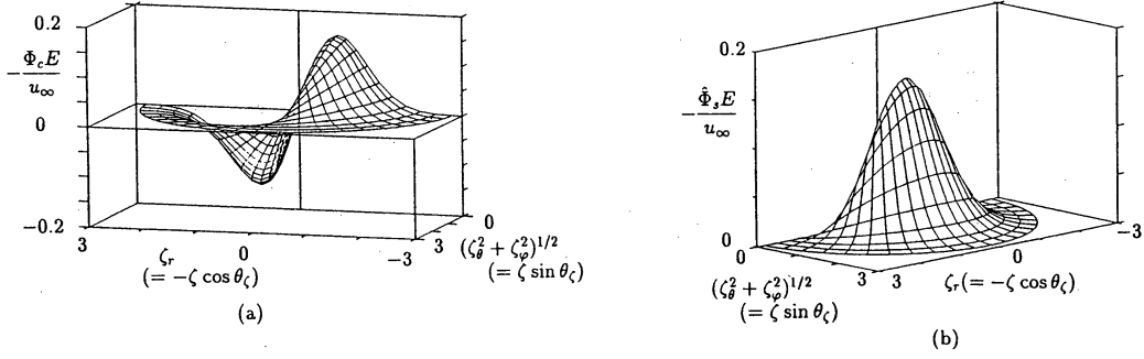
FIG. 12. The velocity distribution functions \Phi_c E and \hat{\Phi}_s E in the uniform flow at infinity. (a) \Phi_c E and (b) \hat{\Phi}_s E . (common to all k_\infty )
