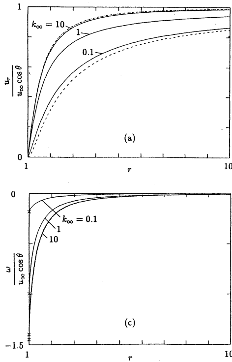
FIG. 3. The profiles of the macroscopic variables (hard sphere). (a) u_r/u_\infty \cos \theta vs r , (b) u_\theta/u_\infty \sin \theta vs r , (c) \omega/u_\infty \cos \theta vs r , and (d) \tau/u_\infty \cos \theta vs r . Here, — indicates the present numerical result, - - - the asymptotic solution (26a)-(26d) with k_\infty = 0 , and - - - the free molecular flow ( k_\infty = \infty ). The \times indicates the value at r = 1 .
