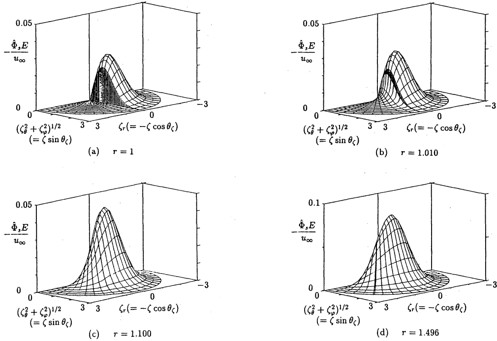
FIG. 7. The velocity distribution function \hat{\Phi}_s E at four points in the gas for k_\infty = 0.1 . (a) r = 1 , (b) r = 1.010 , (c) r = 1.100 , and (d) r = 1.496 . The surface of \hat{\Phi}_s E is shown as a function of \zeta \cos \theta_\zeta and \zeta \sin \theta_\zeta by lines \zeta = \text{const} and \theta_\zeta = \text{const} . The vertical stripes show the discontinuity. Note the difference of the ordinate in Fig. 7d.
