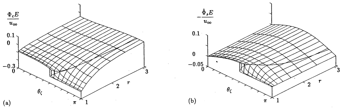
FIG. 17. The velocity distribution functions \Phi_c E and \hat{\Phi}_s E at \zeta = 0.139 for k_\infty = 1 . (a) \Phi_c E and (b) \hat{\Phi}_s E . (See the caption of Fig. 14.)
