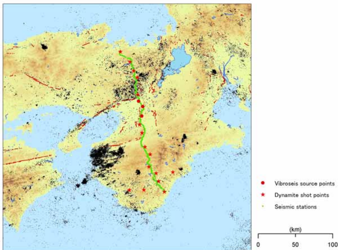
Fig.1 Location of shots (red stars), multiple vibration points (circles) and observation stations (green dots) of seismic survey in 2004. Dots show epicenter of earthquakes with M > 3 and depth < 30\text{km} from Oct., 1997 to Dec., 2004 after JMA unified hypocenter data. Active faults (red lines) are also indicated.
