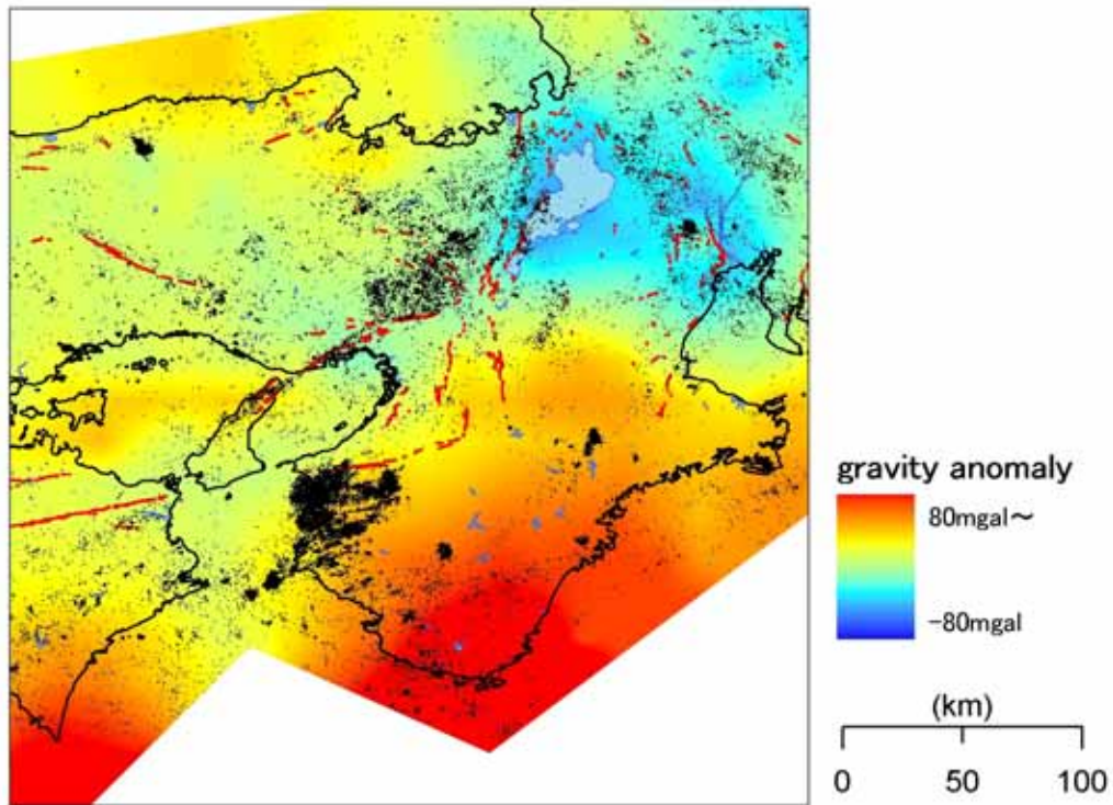
Fig.7(a) Variations of Bouguer gravity anomaly after Komazawa(2000). Dots indicate epicenter distribution of earthquakes with M>3 and depth <30\text{km} from Oct., 1997 to Dec., 2004. Red lines show active faults.
