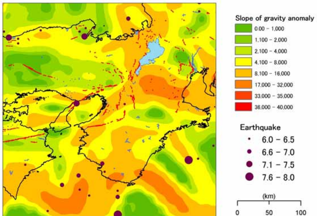
Fig.7(b) Gradient of gravity anomaly. Dots indicate large earthquake with M\ 6 or greater from 1926 to 2004. Red lines show active faults.
