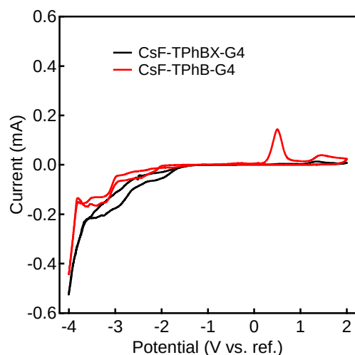
Figure 2. Cyclic voltammograms of a Pt electrode in CsF-TPhBX-G4 and CsF-TPhB-G4. Sweep rate: 0.1 mA s -1 . Sweep range: -4.0 - 2.0 V (vs. ref.).
