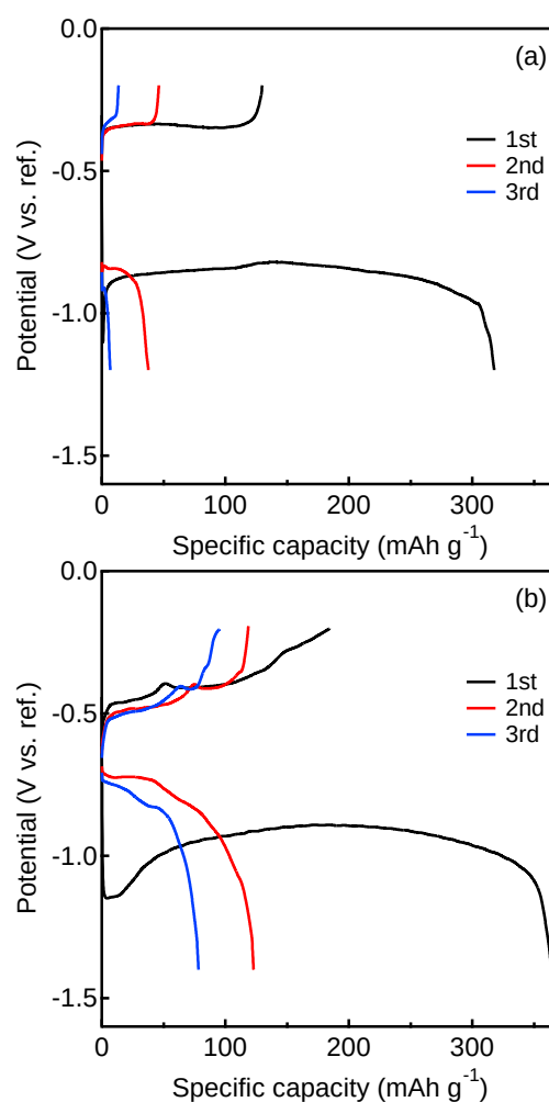
Figure 3. Discharge and charge curves of BiF 3 electrode with electrolyte (a) CsF-TPhBX-G4 within potential range from -1.2 to -0.2 V (vs. ref.) and (b) CsF-TPhB-G4 within potential range from -1.4 to -0.2 V (vs. ref.) in the first, second, and third cycle.
