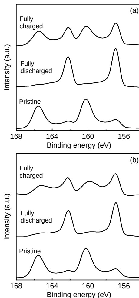
Figure 4. Bi 4f spectra of BiF 3 electrode during the discharge and charge processes in the first cycle [Electrolyte: (a) CsF-TPhBX-G4 and (b) CsF-TPhB-G4].
