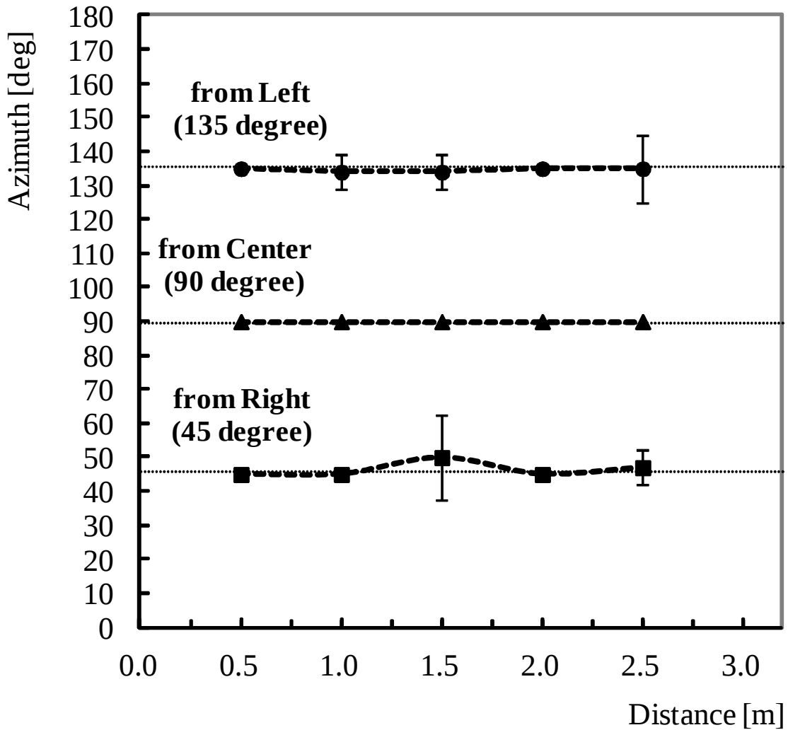
Figure 3.3: The sound source localization at various distances (MUSIC)
