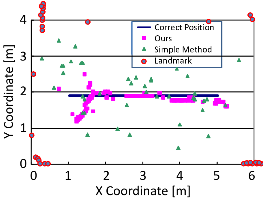
Figure 7.15: The localization results of the developed method and the simple method (7, Figure 11)
