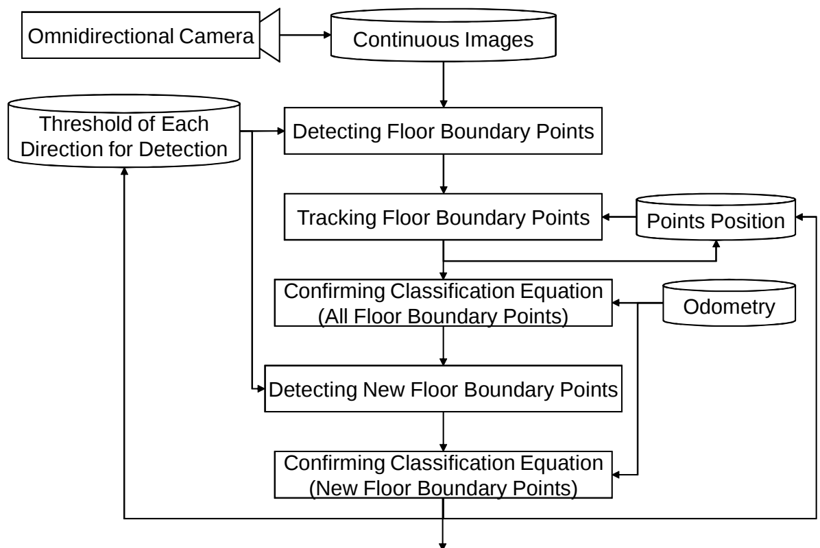
Figure 7.4: The classification system in ApriTau TM (5, Figure 7)
