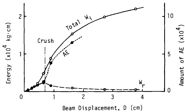
Fig. 5.16. Energy-Displacement Relationship of Beam B25.
