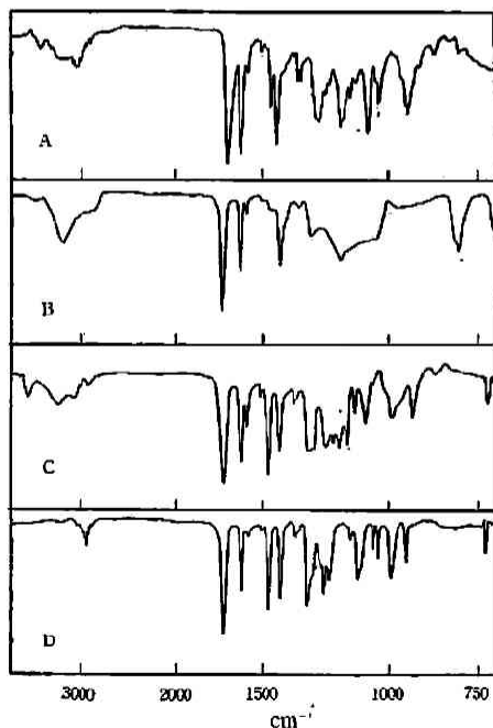
Fig. 14 Infrared spectra of derivatives of benzoylformoin: 1st mono-O-methyl benzoylformoin in chloroform (A); 2nd mono-O-methyl benzoylformoin in tetrahydrofuran (B) and chloroform (C); di-O-methyl benzoylformoin in carbon tetrachloride (D)
