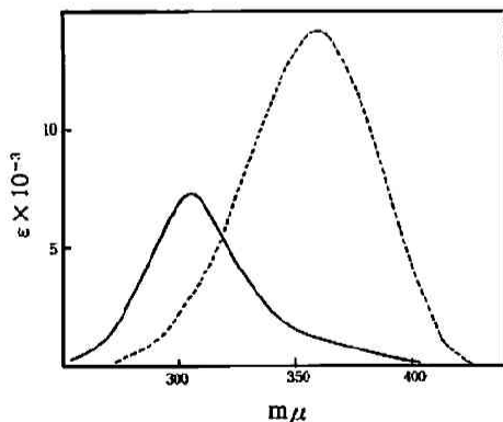
Fig. 6a Ultraviolet spectra of isobutyrylformoin in tetrahydrofuran (—) and chloroform (.....)
