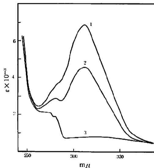
Fig. 8 Ultraviolet spectra of neopentoylformoin in chloroform: (1) in vacuo; (2) 5 hours after breaking the seal; (3) 1 day after breaking the seal
