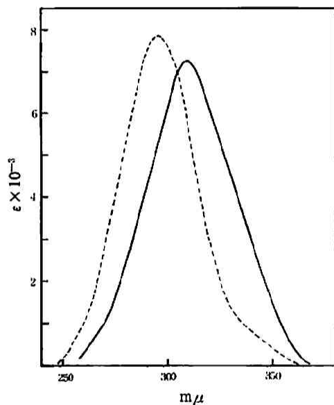
Fig. 11 Ultraviolet spectra of derivatives of neopentylformoin in ethanol: mono-O-methyl neopentylformoin (—); di-O-methyl neopentylformoin (-----)
