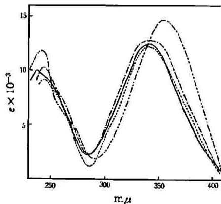
Fig. 12 Ultraviolet spectra of derivatives of benzoylformoin: 1st mono-O-methyl benzoylformoin in ethanol (---); di-O-methyl benzoylformoin in ethanol (---); 2nd mono-O-methyl benzoylformoin in tetrahydrofuran (—) and chloroform (.....)
