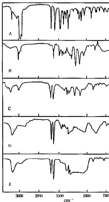
Fig. 2 Infrared spectra of isobutyrylformoin in Nujol (A), chloroform (B), acetonitrile (C), tetrahydrofuran (D) and ether (E)
