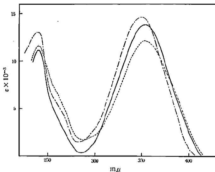
Fig. 9 Ultraviolet spectra of benzoylformoin in tetrahydrofuran (—), ether (---) and ethanol (.....)
