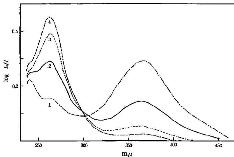
Fig. 10 Ultraviolet spectra of benzoylformoin in chloroform: (1) in vacuo ; (2) 2 hours after breaking the seal; (3) 4 hours after breaking the seal; (4) 1 day after breaking the seal
