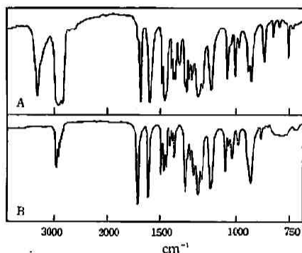
Fig. 13 Infrared spectra of derivatives of neopentoylformoin: mono-O-methyl neopentoylformoin in Nujol (A); di-O-methyl neopentoylformoin in carbon tetrachloride (B)
