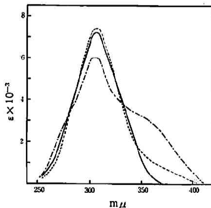
Fig. 6b Ultraviolet spectra of isobutyrylformoin in ethanol (—), acetonitrile (---) and ether (.....)
