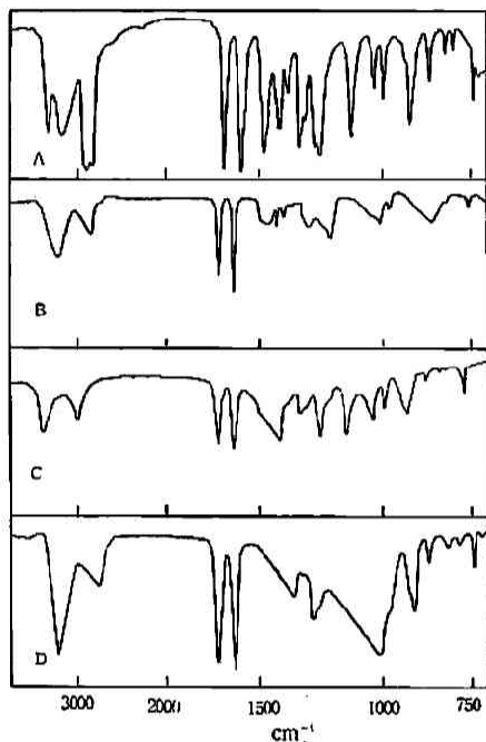
Fig. 3 Infrared spectra of neopentoylformoin in Nujol (A), tetrahydrofuran (B), acetonitrile (C) and ether (D); in ether a 0.2 mm cell was used
