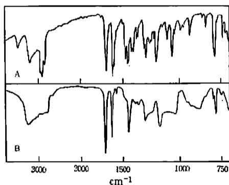
Fig. 4 Infrared spectra of benzoylformoin in Nujol (A) and tetrahydrofuran (B)
