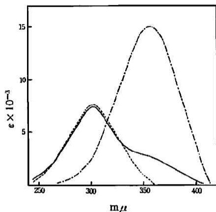
Fig. 5 Ultraviolet spectra of acetylformoin in tetrahydrofuran (—), chloroform (---) and ethanol (.....)
