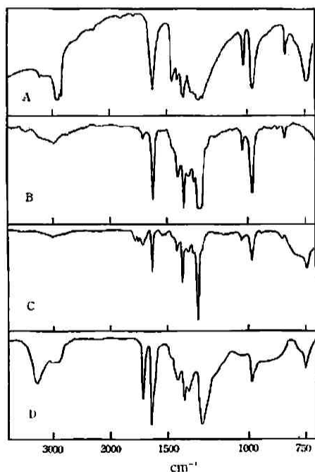
Fig. 1 Infrared spectra of acetylformoin in Nujol (A), chloroform (B), carbon tetrachloride (C) and tetrahydrofuran (D)
